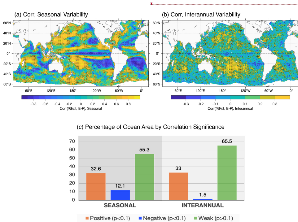
Figure 3. Correlation between E-P and \partial S/\partial t at seasonal and interannual timescales (2012–2022). Spatial distribution of correlation coefficients for (a) seasonal variability (demeaned) and (b) interannual variability (detrended and
