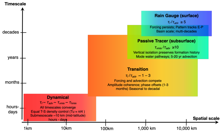
Figure 8. Salinity regime diagram. Four regimes from timescale competition (Table 3). Rain gauge (surface, cyan-blue):
