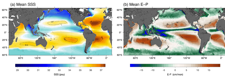
85 Figure 1. Time-mean fields. (a) sea surface salinity (SSS) and (b) evaporation minus precipitation (E – P) averaged over 2012-2022. SSS is from OISSS monthly 0.25° product (Melnichenko 2023), E from OAFflux monthly 0.25° analysis (Yu 2019), and P from GPCP Monthly 0.5° v3.2 (Huffman et al. 2022). Adapted from Yu (2023).
