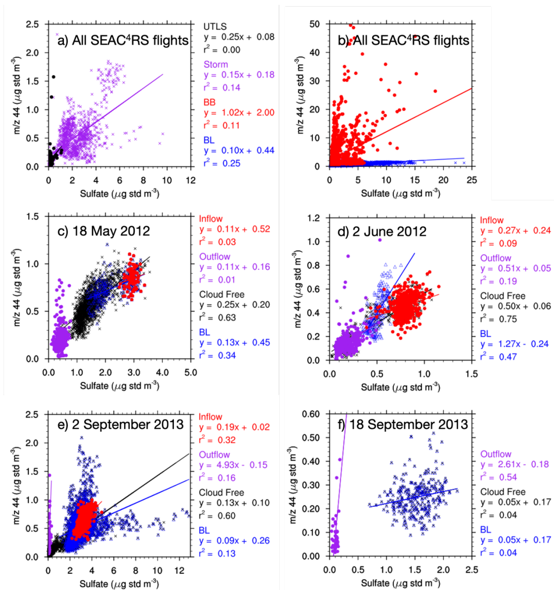
585 Figure 5. Scatter plots of AMS m/z 44 and AMS sulfate concentrations. In a) and b) concentrations from all the SEAC 4 RS flights are shown separating the data by region where a) shows cloud free UTLS data (black circles) at altitudes > 8 km and data near storms (purple crosses), and b) shows cloud free BL data (blue crosses) at altitudes < 2 km and data in BB regions (red circles). In panels c-f) data are separated by inflow (red), outflow (purple), cloud free (black), and BL regions (blue) as defined in the scavenging analysis (and BL data is below 2 km) for c) 18 May 2012, d) 2 June 2012, e) 2 September 2013, and 590 f) 18 September 2013 land convection.
