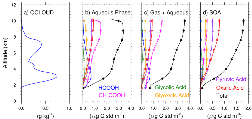
Figure 6. Prescribed cloud parcel model results for organic acid formation using the no lightning-NO x scenario for the 2 September 2013 case. Panel a) shows the prescribed cloud water content ( \text{g kg}^{-1} ) for the model run, panel b) the aqueous-phase organic acid mixing ratios ( \mu\text{g C std m}^{-3} ), panel c) the total (gas + aqueous) organic acid mixing ratios ( \mu\text{g C std m}^{-3} ), and panel d) potential SOA ( \mu\text{g C std m}^{-3} ) using partitioning ratios, for formic acid (blue with asterisks), acetic acid (magenta with open circles), glycolic acid (green with open square), glyoxylic acid (gold with left pointing triangles), pyruvic acid (purple with triangles), oxalic acid (red with right pointing triangles), and the sum of the six organic acids (black with closed circles).
