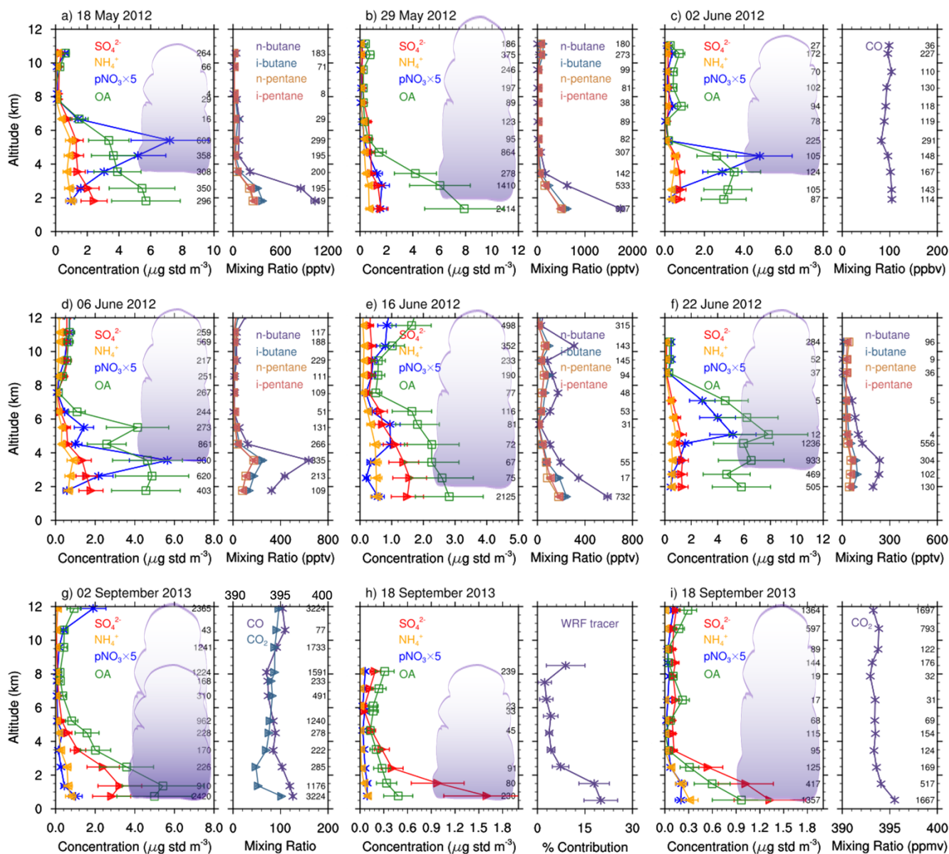
380 Figure 2. Clear air vertical profiles of sulfate (red with right arrows), particulate nitrate (blue with asterisks), ammonium (gold with left arrows), and organic aerosol (green with squares) and the passive, insoluble trace gases used in the entrainment model for for a) 18 May 2012, b) 29 May 2012, c) 2 June 2012, d) 6 June 2012, e) 16 June 2012, f) 22 June 2012, g) 2 September 2013, h) 18 September 2013 over the Gulf of Mexico, and i) 18 September 2013 over South Texas. Average and standard deviations are plotted for each altitude bin, which is plotted at the average altitude of each 1-km bin. Nitrate concentrations shown are multiplied by a factor of 5 for visibility. In g), the CO 2 mixing ratio (ppmv) axis is at the top of the panel. The cloud schematic in each panel is used to locate the approximate cloud base and cloud top heights for each case.
