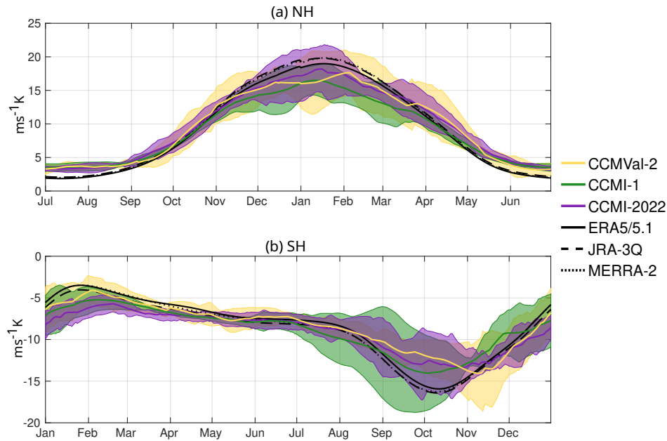
Figure 12. Annual cycle of the eddy heat flux at 100 hPa averaged over the latitude band 45°-75° in the NH (a) and the SH (b). Note that positive fluxes in the NH and negative fluxes in the SH both indicate poleward eddy heat transport and upward wave propagation.
