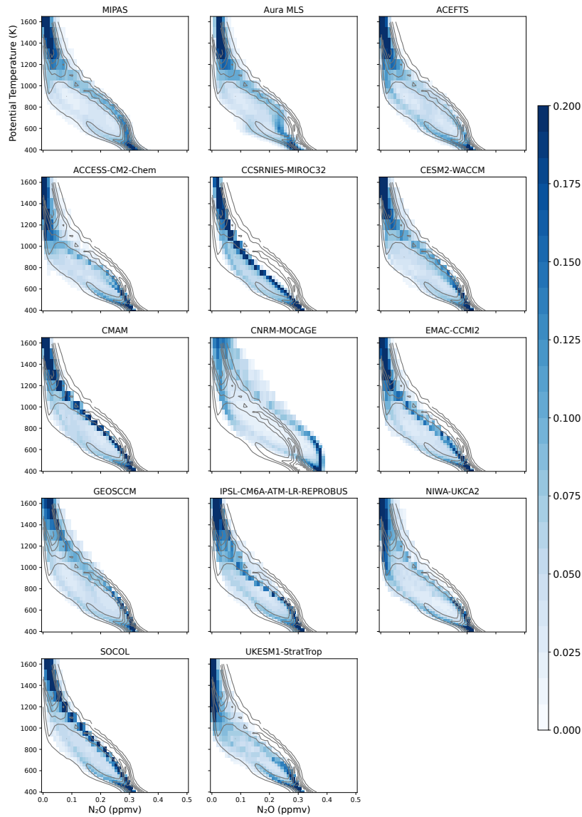
Figure 7. PDFs for N_2O satellite data from MIPAS, MLS, ACE-FTS (top panels), and monthly mean model data from CCMIs-2022 models. 10S-45N, MAM season 2005-2012 period. The ACE-FTS PDF contours are shown in all panels to facilitate the comparison (gray contours). The tracer mixing ratios are binned in 100 bins in the range 0-5 ppmv, and the PDF is normalized such that the total frequency on each level adds up to 1.
