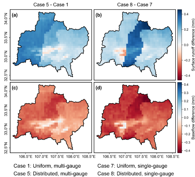
565 Figure 7. Spatial distribution of differences in (a, b) surface runoff and (c, d) baseflow volumes between the two parameterization schemes over the validation period. Differences are calculated as spatially explicit minus uniform parameterization.
