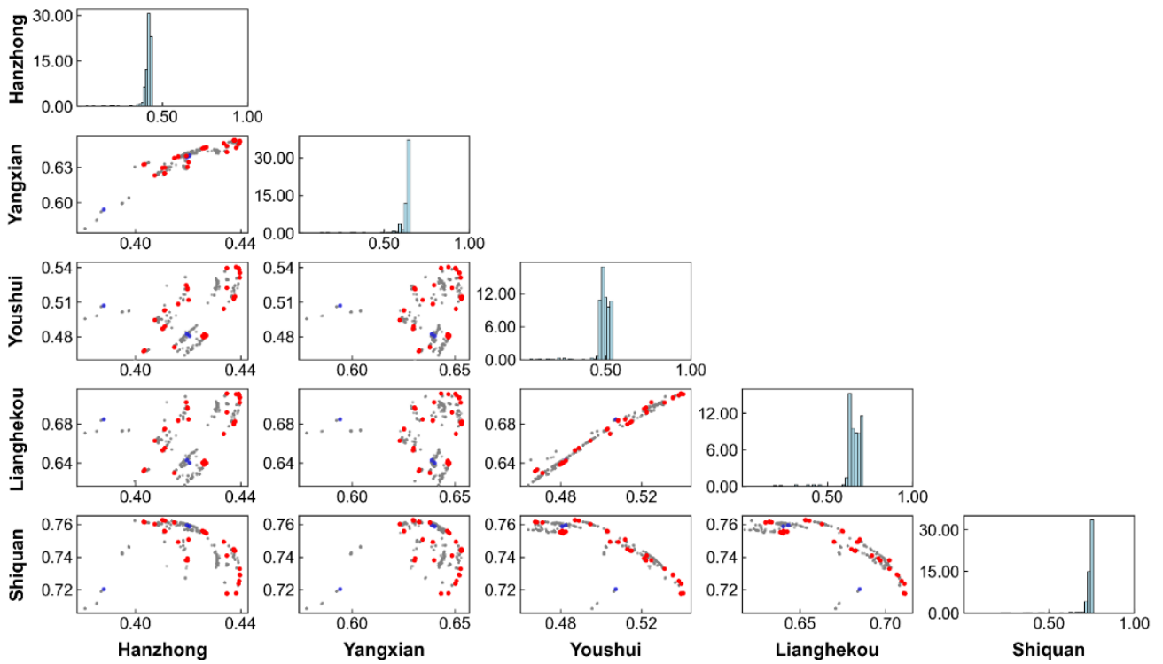
Figure 110. Objective space scatter plot matrix for Case 1. The matrix depicts the trade-offs between calibration objectives, where each axis corresponds to the Kling-Gupta Efficiency (KGE) of simulated streamflow for a sub-basin (gauge). Grey dots represent all candidate solutions from the calibration process. The initial and final Pareto fronts are highlighted in blue and red, respectively. Histograms along the diagonal show the distribution of the KGE for each individual objective.
