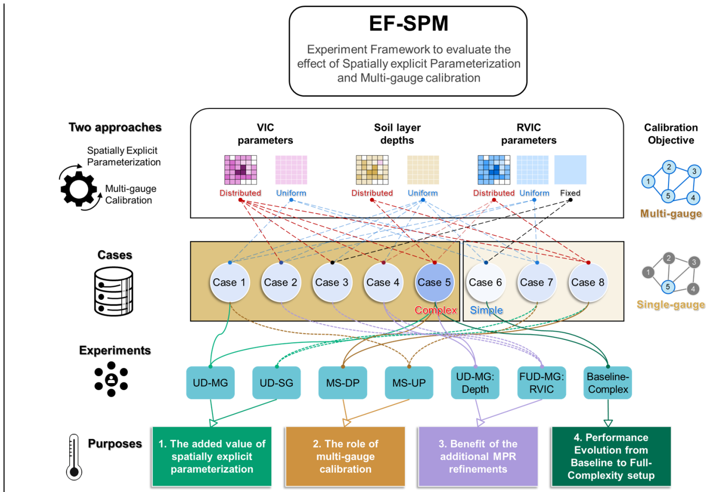
405 Figure 3. Schematic illustration of the Experiment Framework to evaluate the effect of Spatially explicit Parameterization and Multi-gauge calibration (EF-SPM).
