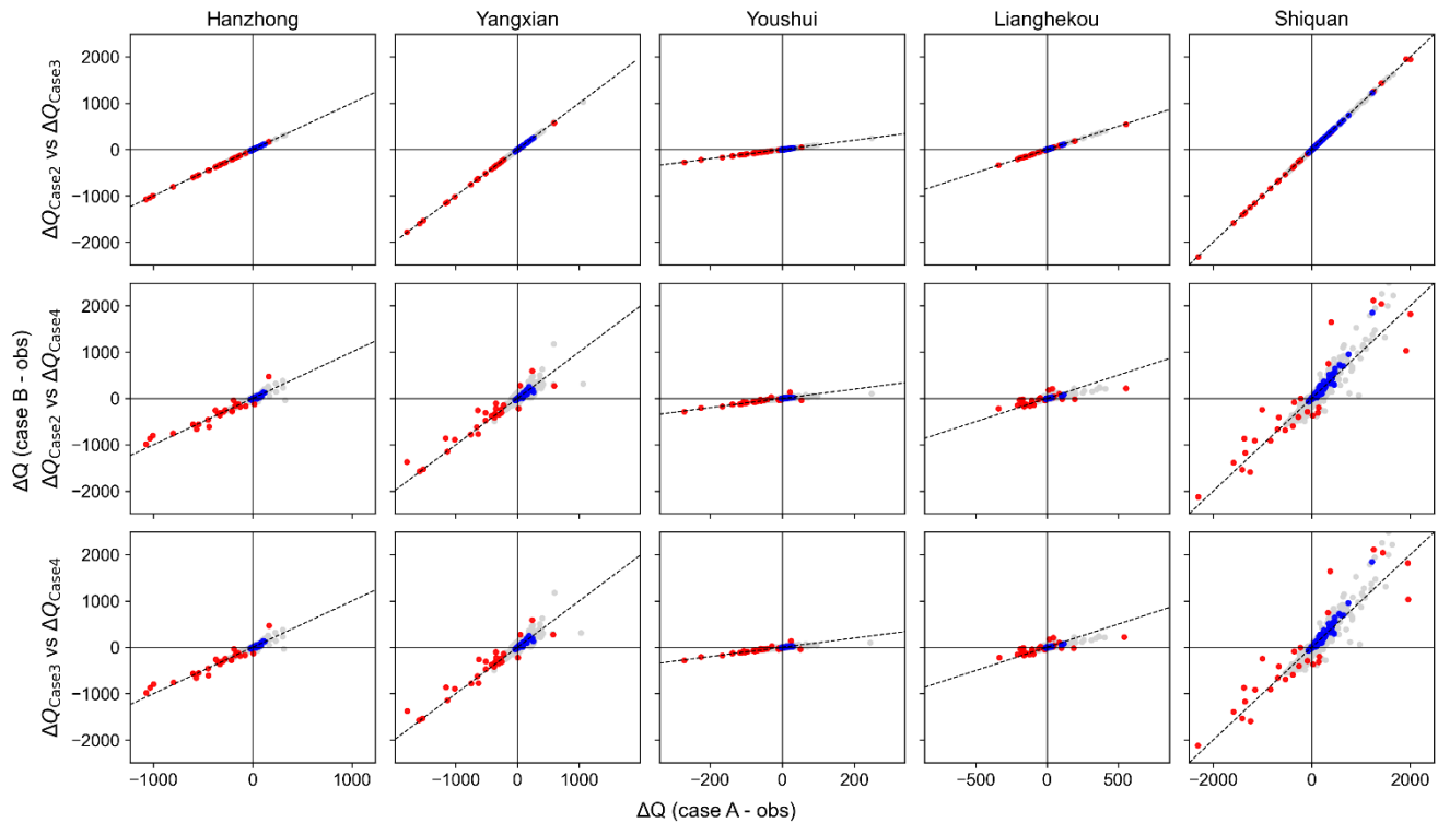
815 Figure 154. Scatter plots of simulated streamflow residuals ( \Delta Q ) for Cases 3, 2, and 4 during the validation period, using the runoff generation parameters from Case 3. Red and blue dots represent high flows (exceedance probability < 2%) and low flows (exceedance probability > 70%), respectively. The dashed line indicates the 1:1 line.
