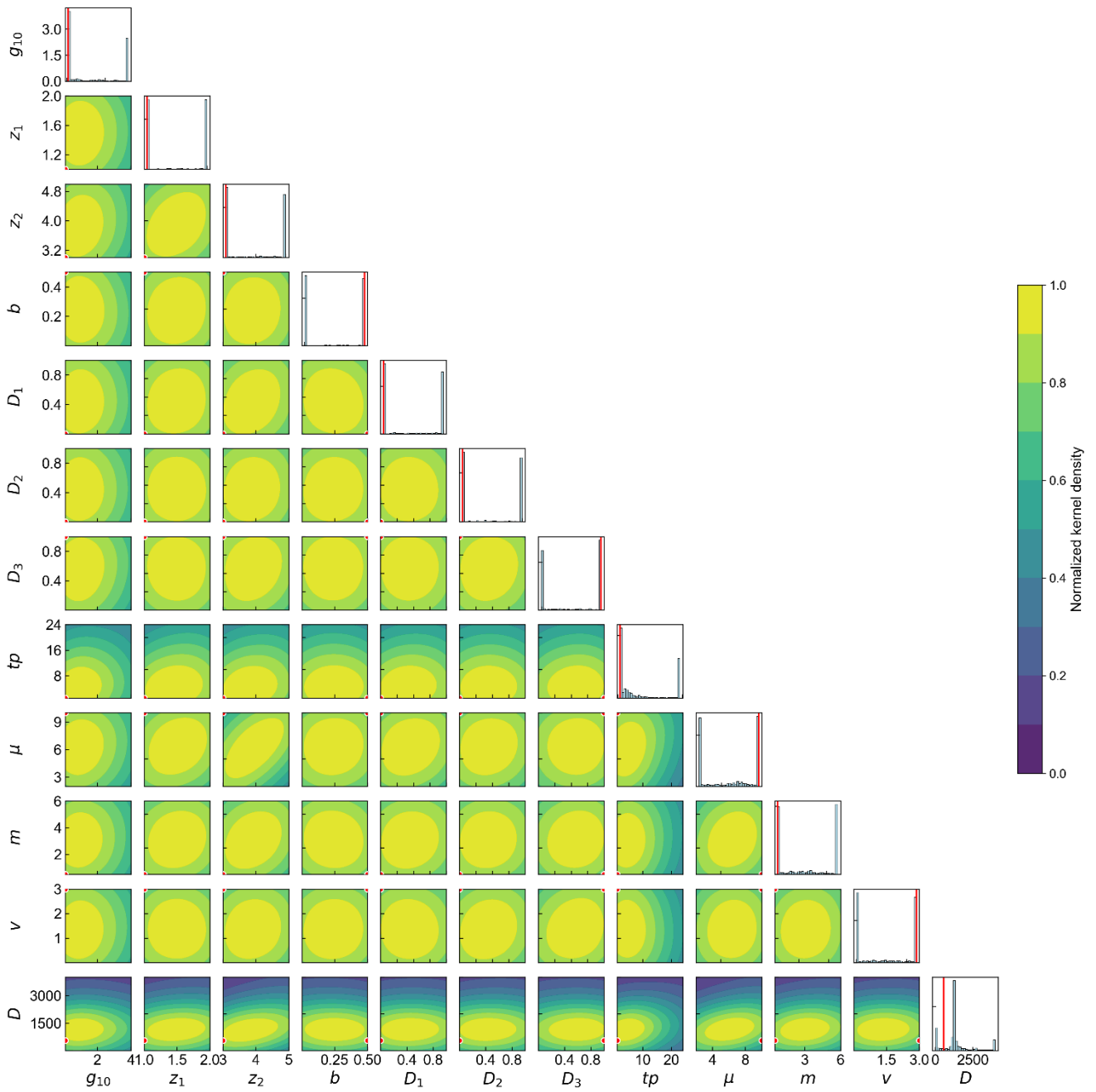
595 Figure 8. Post-calibration parameter distributions for Case 7. The optimal parameters are shown as red dots and lines. The background contours represent the standardized kernel density estimate derived from all candidate solutions, where yellow shading corresponds to high probability density regions. The histograms along the diagonal represent the marginal distribution of each individual parameter.
