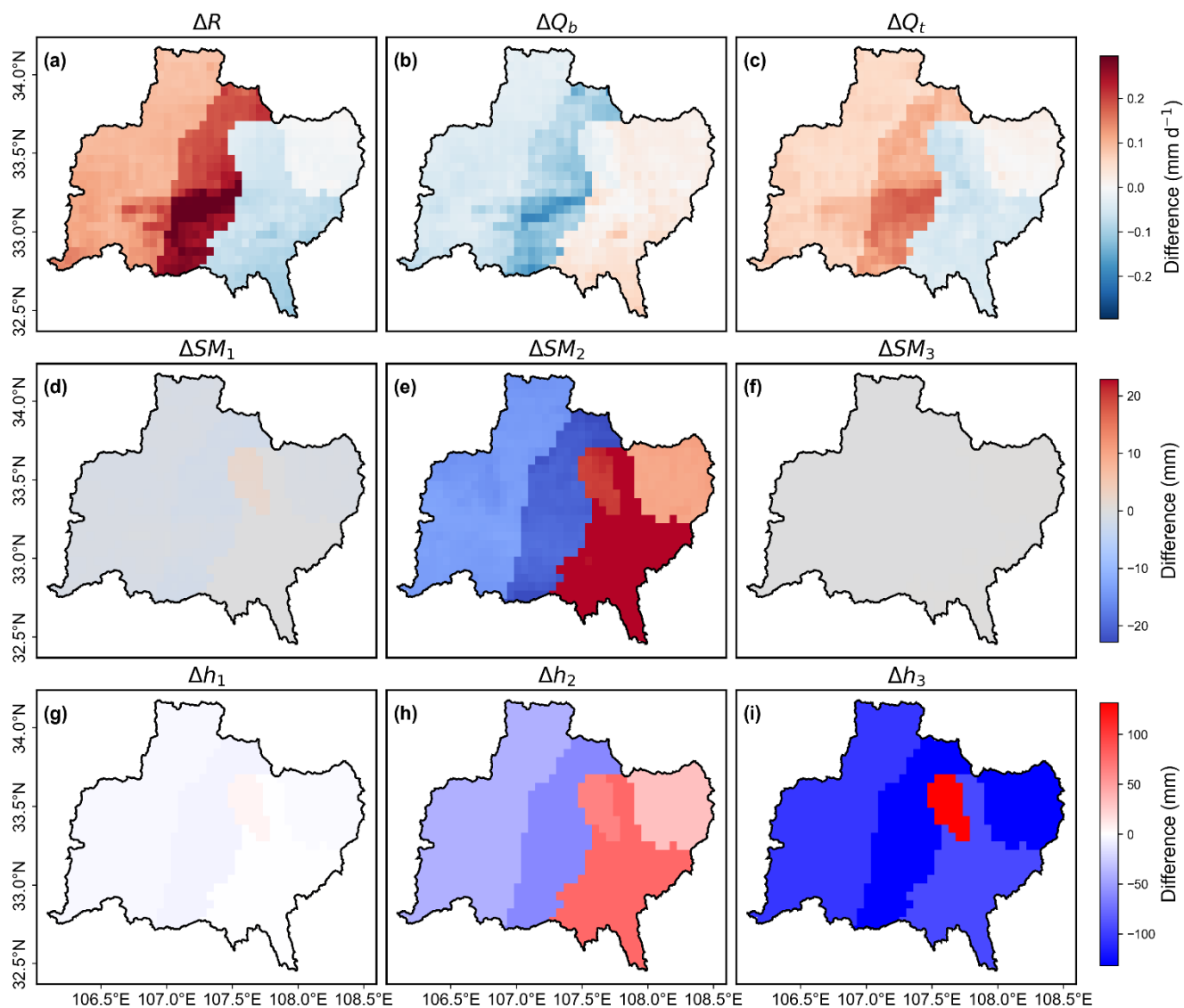
765 Figure 143. Spatial distribution of differences in long-term mean simulated variables during the validation period and soil layer depths between Case 4 and Case 5. Differences are shown for (a–c) surface runoff, baseflow, and total runoff, and (d–f) soil moisture in layers 1–3, respectively (variable definitions as in Fig. 132). The bottom row presents the corresponding differences in the calibrated soil layer depths: (g–i) Depths differences for soil layers 1-3 ( \Delta h_1 , \Delta h_2 , \Delta h_3 ). Positive values indicate higher magnitudes in Case 5 relative to Case 4.
