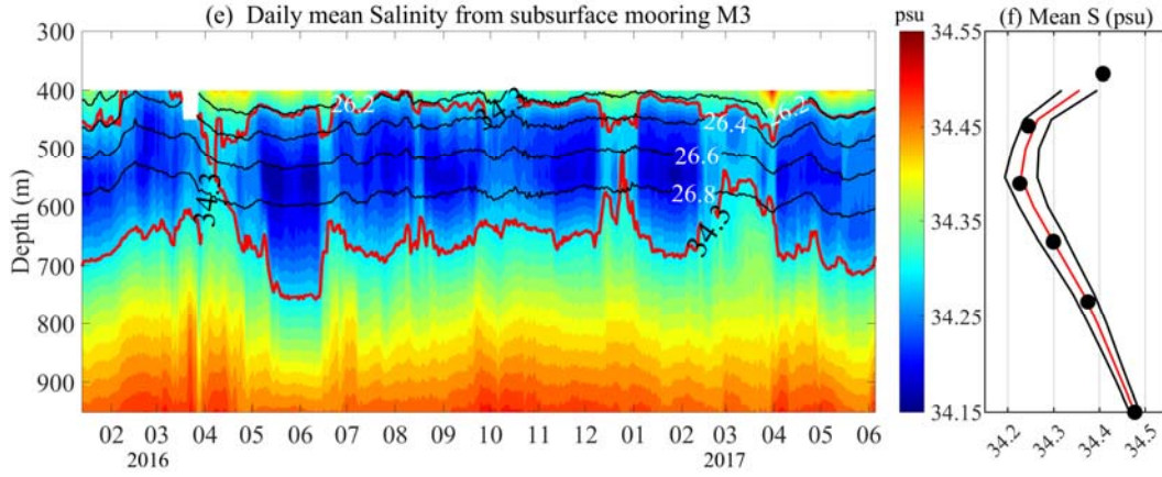
Figure 2. The observation of salinity from subsurface mooring. (a), (c) and (e) represent time series plots of salinity measured at different observation times for the three moorings, respectively. M1 is observed from April 2017-June 2018, M2 is observed from August 2019-December 2020 and M3 is observed from January 2016-June 2017. Color shading and the black lines represent the salinity and 26.2 to 27.0 \sigma_\theta isopycnal, and also red line represent the 34.3 psu in (a), (c) and (e), respectively. In (b), (d) and (f), the red line and black line represent the mean salinity and standard deviation of salinity over the observation period, respectively. The black circle in (b), (d) and (f) are represents the average depth of deployed CTDs in subsurface moorings.
