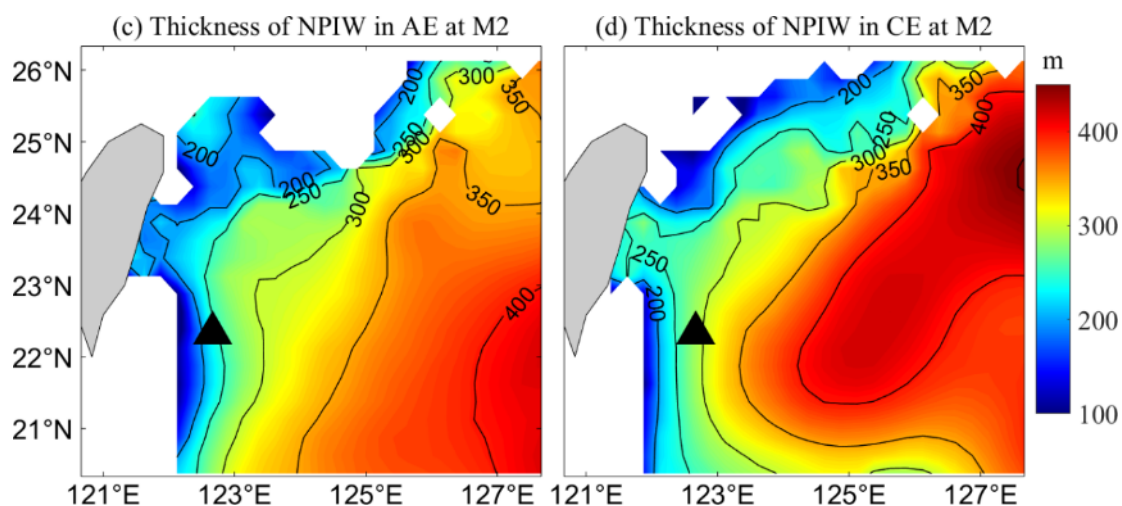
Figure 13. (a) Composite distribution of salinity (color shading) and current vectors (black arrows) averaged over the 500–800 m layer during high-salinity events generally associated with anticyclonic conditions near the M2 mooring site from CMEMS data. (b) Same as (a), but for low-salinity events generally associated with cyclonic conditions. (c) Composite thickness of the NPIW layer during high-salinity events, calculated from the 34.3 psu isohaline boundaries. (d) Same as (c), but for low-salinity events. Black triangles indicate the mooring locations.
