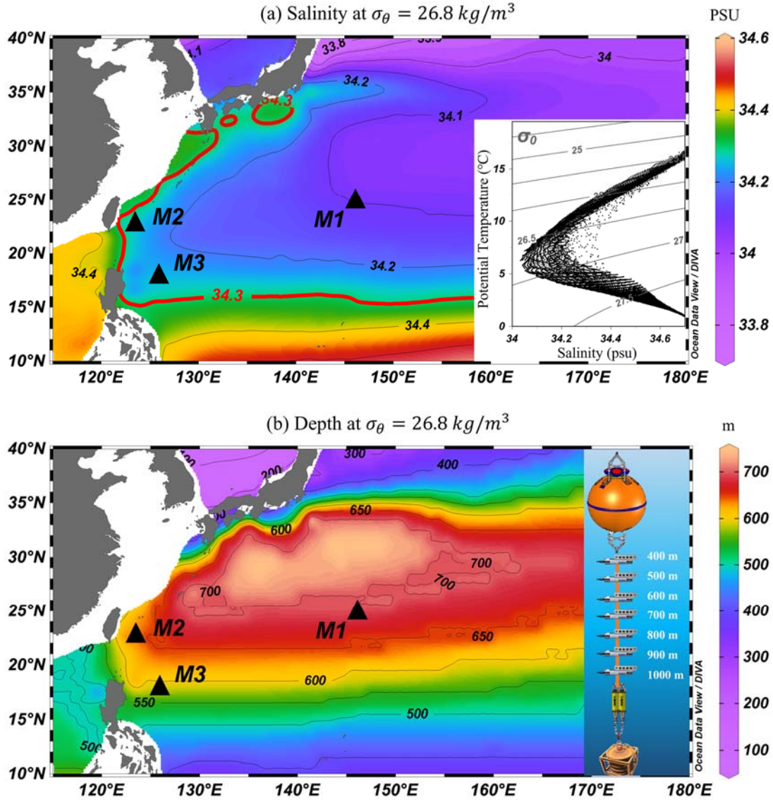
Figure 1. Distribution of salinity (a) and depth (b) along the 26.8\sigma_\theta isopycnals at Northwestern Pacific. The T-S scatter plot in the lower-right corner of (a) illustrates the vertical distribution of NPIW. The color shading and black line in (a) and (b) represent the salinity and depth, respectively. The right-hand side of (b) shows a schematic diagram of the CTD deployment with mooring. The red contours of 34.3 psu is represent the NPIW range from Talley et al. (1993) and You et al. (2003). The black triangle is the mooring location: Mooring 1 (M1), Mooring 2 (M2) and Mooring 3 (M3). Salinity and depth in the Fig. 1 are taken from climatological averaged data from World Ocean Atlas 2023 (WOA23) © NOAA National Centers for Environmental Information, and plot with Ocean Data View .
