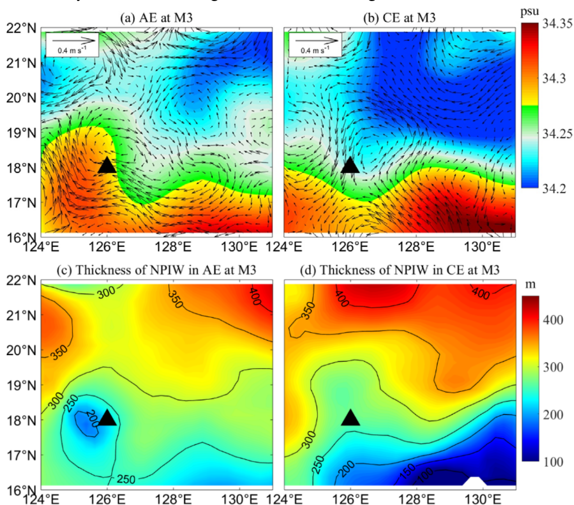
Figure 14. (a) Composite distribution of salinity (color shading) and current vectors
