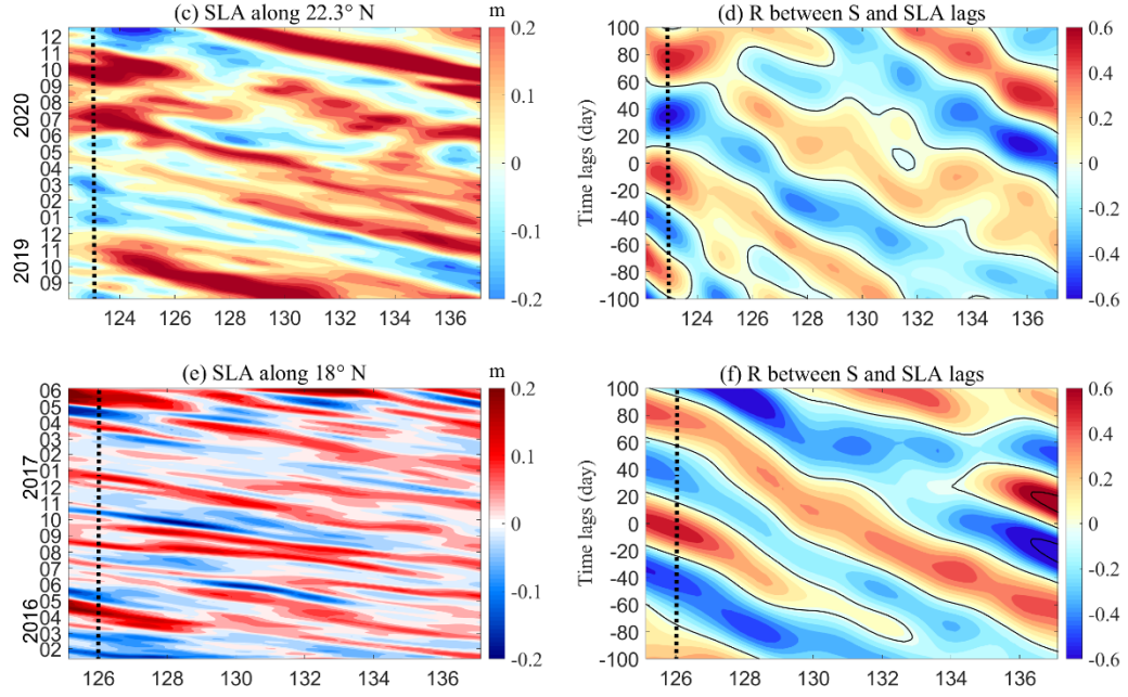
Figure 9. (a) Temporal evolution of sea level anomalies (SLAs) across longitudes at 25°N, as illustrated by the contour plots.; (b) The correlation coefficient between salinity at M1 and SLA at different time lags, the vertical coordinates -100 to 100 days in (b) represent SLA lagging salinity for 100 days and SLA exceeding salinity for 100 days, respectively. (c) and (e) are same as (a), but its along 22.3°N and 18°N, respectively. (d) and (f) are same as (b), but for salinity from M2 and M3, respectively. Black contours in Fig. 9b, 9d, and 9f represent the zero isolines. The black dash line represent the location of M1, M2 and M3, respectively. The SLA data shown in this figure were obtained from the CMEMS dataset introduced in the Methods section.
