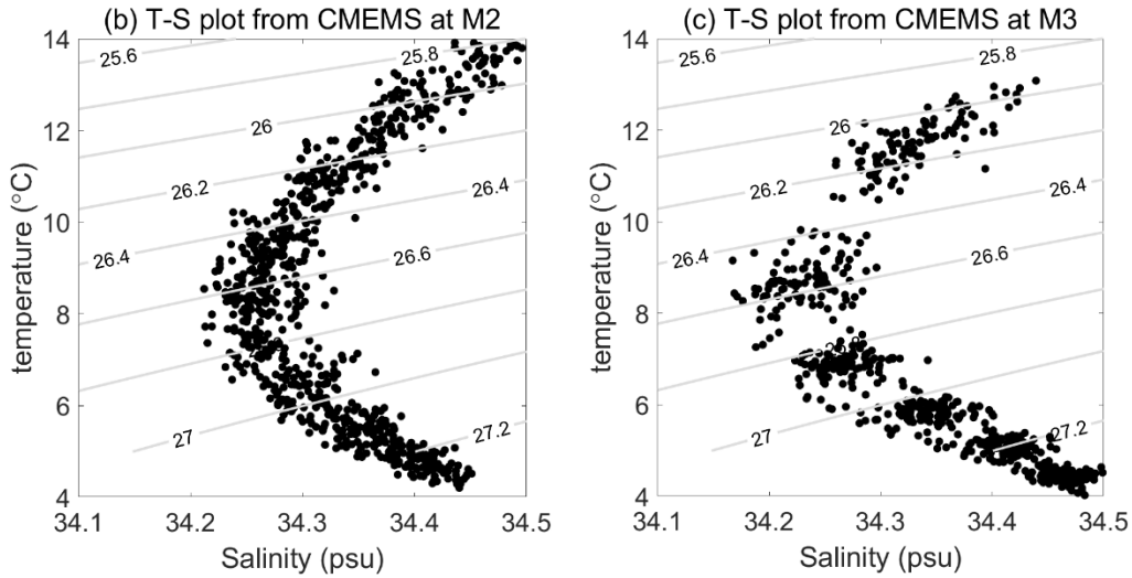
Figure. The T-S plot from CMEMS dataset at M2 and M3 mooring site.
