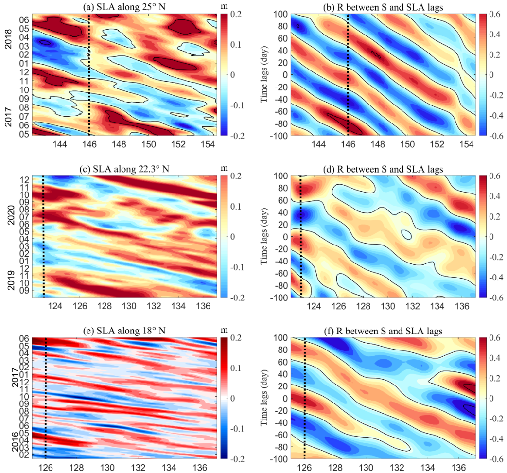
Figure 9. (a) Temporal evolution of sea level anomalies (SLAs) across longitudes at 25°N, as illustrated by the contour plots.; (b) The correlation coefficient between
