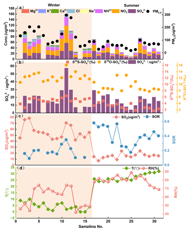
Figure 2. Time series of concentrations (values) of (a) \text{PM}_{2.5} and ions, (b) \text{SO}_4^{2-} and \delta^{34}\text{S}\text{-SO}_4^{2-} , \delta^{18}\text{O}\text{-SO}_4^{2-} , (c) \text{SO}_2 and SOR, and (d) ambient temperature ( T ) and RH.
