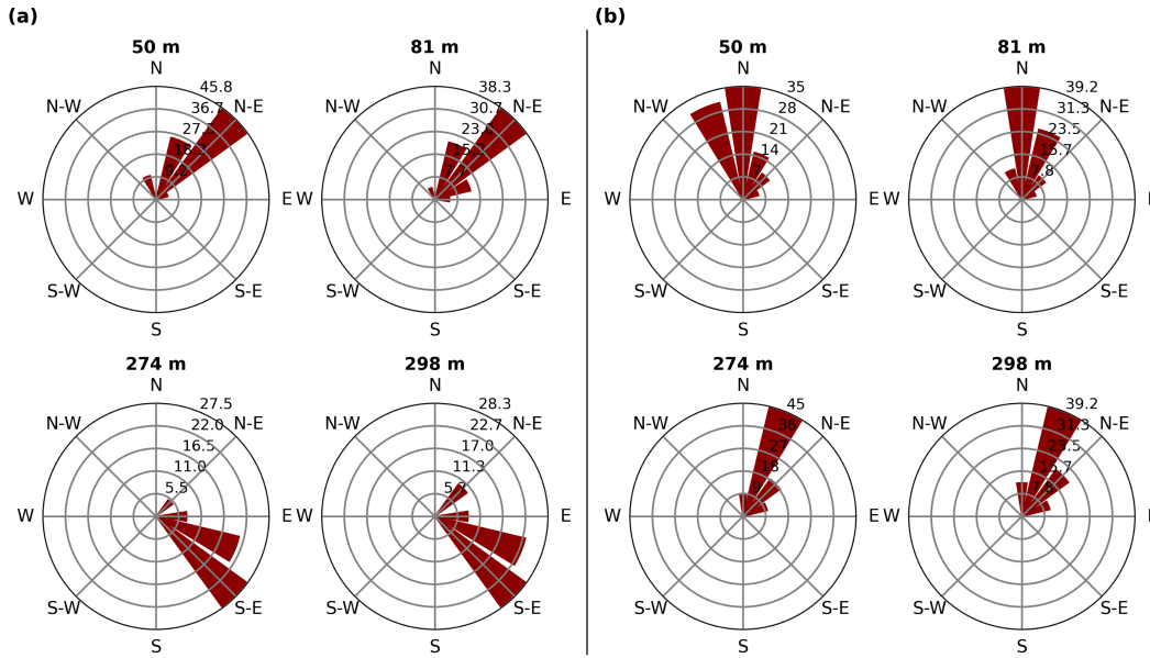
Figure 8. Wind direction at four distinct heights for a) 18/08/2022 18 August 2022 and b) 25/08/2022 25 August 2022.
