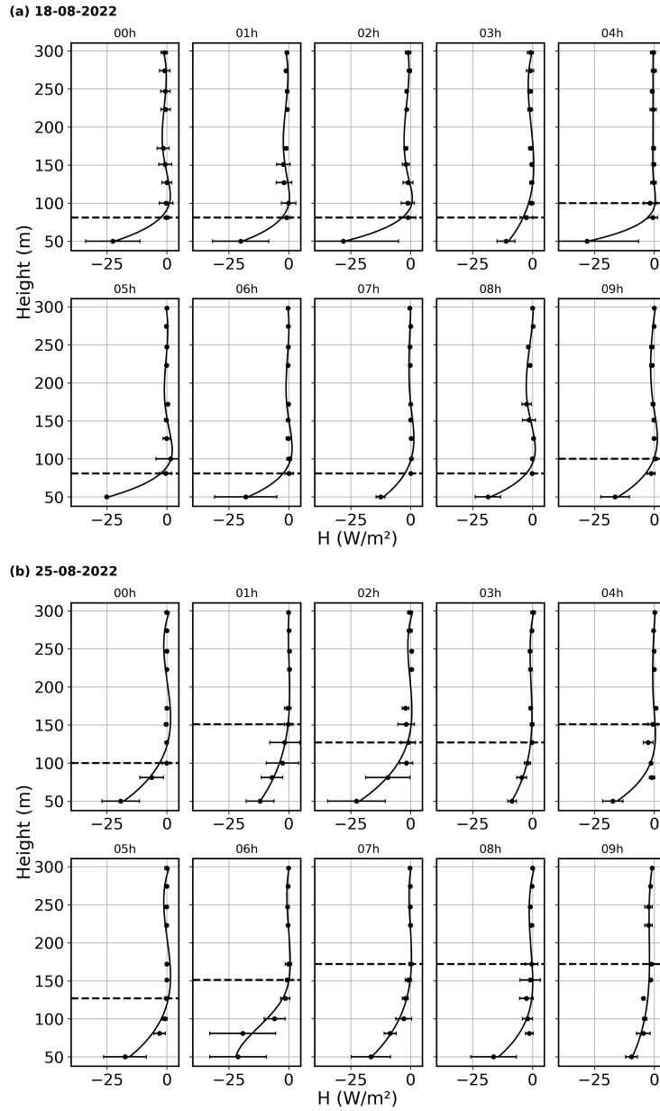
Figure 6. Hourly mean profiles of sensible heat flux (black curve), standard deviation, and the corresponding h_n (horizontal dotted lines) for a) 18/08/2022 18 August 2022 and b) 25/08/2022 25 August 2022.
