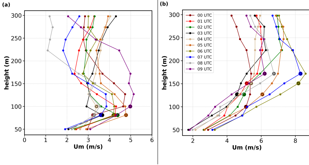
Figure 7. Hourly mean wind speed profiles for a) 18/08/2022 18 August 2022 and b) 25/08/2022 25 August 2022. The different colors indicate the different hours. The larger hollow circles mark the hourly estimates of the h_n , determined from the sensible heat flux profiles.
