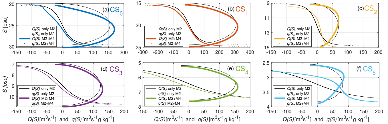
Figure 6. Volume transports Q(S) (solid curves) and exchange profiles (dotted curves) q(S) sorted by salinity classes are computed at cross-sections CS_i considering the superposition of the M2-M2 and M4-M4 constituents (colored curves) and the M2-M2 only, without the M4-M4 contribution (black curves).
