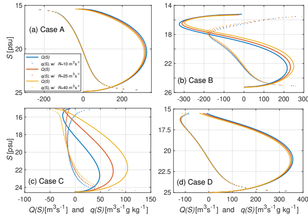
Figure 8. Volume transports Q(S) (solid curves) and exchange profiles q(S) (dotted curves) for cases A, B, C, and D marked with black circles in the parameter space in panels a1 ( R = 10 \text{ m}^3\text{s}^{-1} ), a2 ( R = 25 \text{ m}^3\text{s}^{-1} ), and a3 ( R = 40 \text{ m}^3\text{s}^{-1} ) of Figure 7. Legend is common to the four panels.
