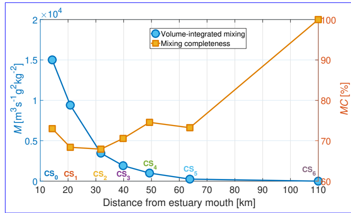
Figure 5. Volume-integrated mixing (left y-axis; dark blue curve, circles) and mixing completeness (inset right y-axis; dark yellow curve, squares).
