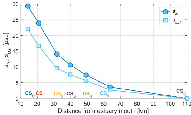
Figure 4. Knudsen consistent Knudsen consistent salinities for in- (dark blue curve, circles) and outflows (light blue curve, squares) at cross-sections along the estuary.
