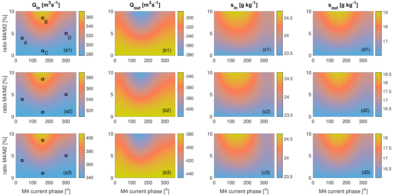
Figure 7. Sensitivity of Knudsen-consistent -incoming (panels a1, a2, and a3) and outgoing volume transports (panels b1, b2, and b3) and salinities for inflows (panels c1, c2, and c3) and outflows (panels d1, d2, and d3) to ratio between M4 and M2 current amplitudes ( u_b/u_a ) and to M4 current phase ( \varphi_b ). First, second and third row of panels correspond with R = 10\text{ m}^3\text{ s}^{-1} , R = 25\text{ m}^3\text{ s}^{-1} , and R = 40\text{ m}^3\text{ s}^{-1} , respectively. Black circles and capital letters indicate example cases in the parameter space shown in Fig. 8.
