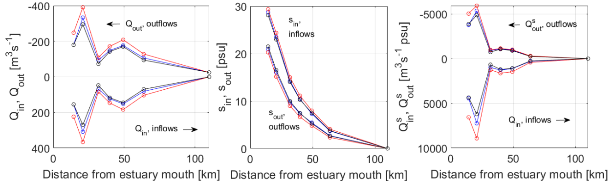
Figure 3: Left panel: Outgoing Q_{out} and incoming Q_{in} volume transports. Middle panel: Knudsen-consistent salinities for inflows, s_{in} , and outflows, s_{out} . Right panel: Incoming Q_{in}^s and outgoing Q_{out}^s salinity volume transports. Estimates at each cross-section CS_i at given during the whole analysis period (blue curves and circles), a spring tide (red curves and circles), and a neap tide (black curves and circles).
