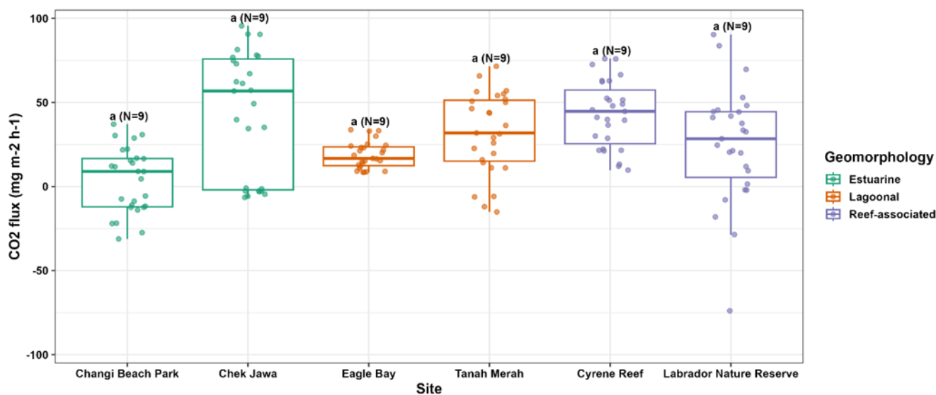
195 Figure 3. Sediment–air CO 2 flux (mg m -2 h -1 ) across sites during low-tide exposure (dark chambers). Boxplots show chamber-level flux distributions; points show individual chambers, coloured by geomorphology. The y-axis limits are symmetric ( \pm \max(|\text{CO}_2|) ) across all chambers) to aid cross-site comparison. Letters above sites indicate Tukey-adjusted differences in site estimated marginal means from the site mixed model (emmeans; \alpha = 0.05 ); sites sharing a letter are not significantly different. N indicates the number of plots contributing flux measurements at each site. 200
