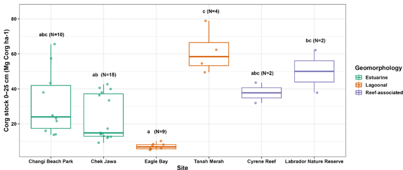
190 Figure 2. Measured only 0–25 cm soil organic carbon stocks (Mg C org ha -1 ) across sites, restricted to 0-25 cores (cores reaching \geq 25 cm depth). Boxplots show medians and interquartile ranges; points show individual cores, coloured by geomorphology. Letters above sites indicate Tukey-adjusted differences in site estimated marginal means (emmeans; \alpha = 0.05 ); sites sharing a letter are not significantly different. N indicates the number of 0-25 cm cores per site.
