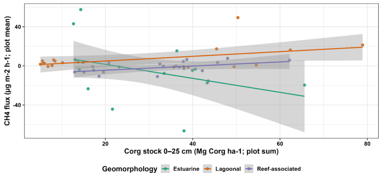
Figure 5. Plot-level relationships between measured 0–25 cm C org stocks (plot-summed) and plot-mean greenhouse gas fluxes. Panel (A) shows CO 2 versus 0–25 cm C org stock; panel (B) shows CH 4 versus 0–25 cm C org stock. Points represent plots coloured by geomorphology; lines show linear fits with 95% confidence bands. Statistical inference is based on mixed-effects models that included geomorphology as a fixed effect and a random intercept for site.
