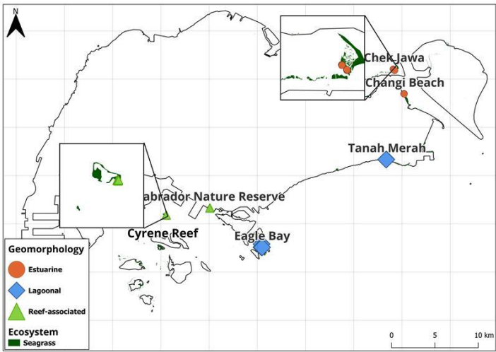
80 Figure 1: Singapore seagrass extent map (Tan et al., 2022) and study sites locations of intertidal seagrass meadows across estuarine, lagoonal and reef-associated geomorphic settings. Two sites with the largest seagrass extent among the studied sites are zoomed in.
