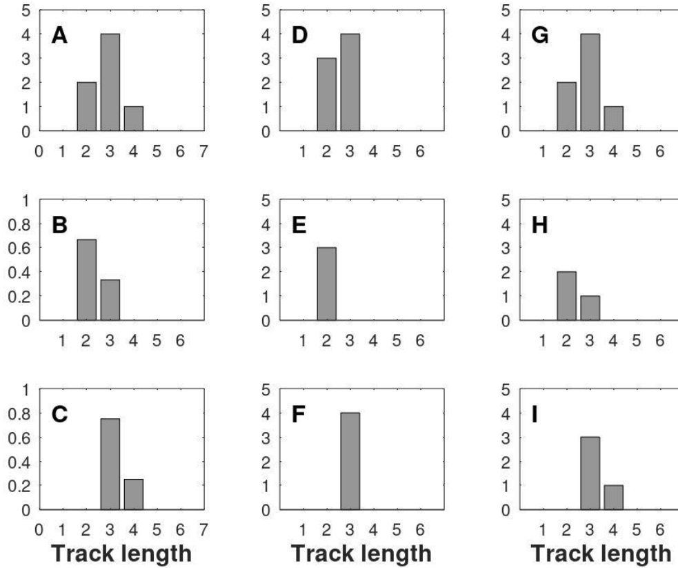
Fig. 1. Illustration of deconvolution. A. A synthetic histogram. B. A synthetic normalized histograms of tracks generated in a short time interval and then annealed. C. A histogram like the one in A but annealed less. E and F. Columns representing factors. H and I. Histograms derived from the histograms in B and C by multiplication by the factors shown in E and F. G. Histogram constructed by addition of the histograms in H and I. Histogram G is equal to histogram A since the factors E and F are chosen correctly. D. This histogram is the deconvolution of histogram A. It is derived by summation of histogram E and F.
