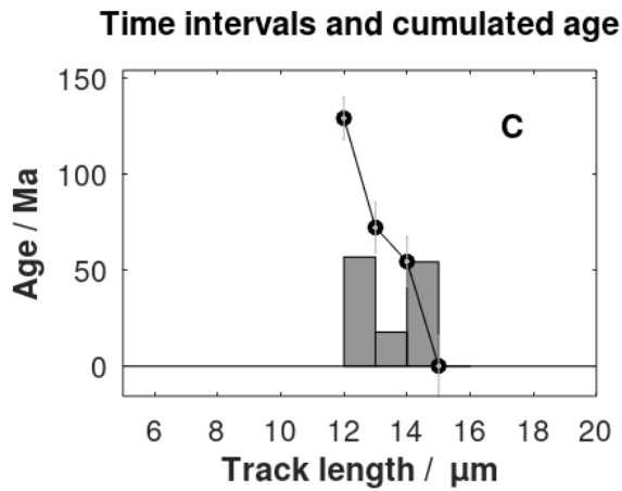
270 Figure 6: A. c-axis projected track histogram of the gneiss sample GRÖ21 (Spiegel et al. 2023b) and the calculated distribution. B. Deconvolution. C. Histogram of time intervals and cumulated track ages. The age nodes (black dots) are the y-values plotted as a function of the c-axis projected track lengths and tabulated in Table 1.
