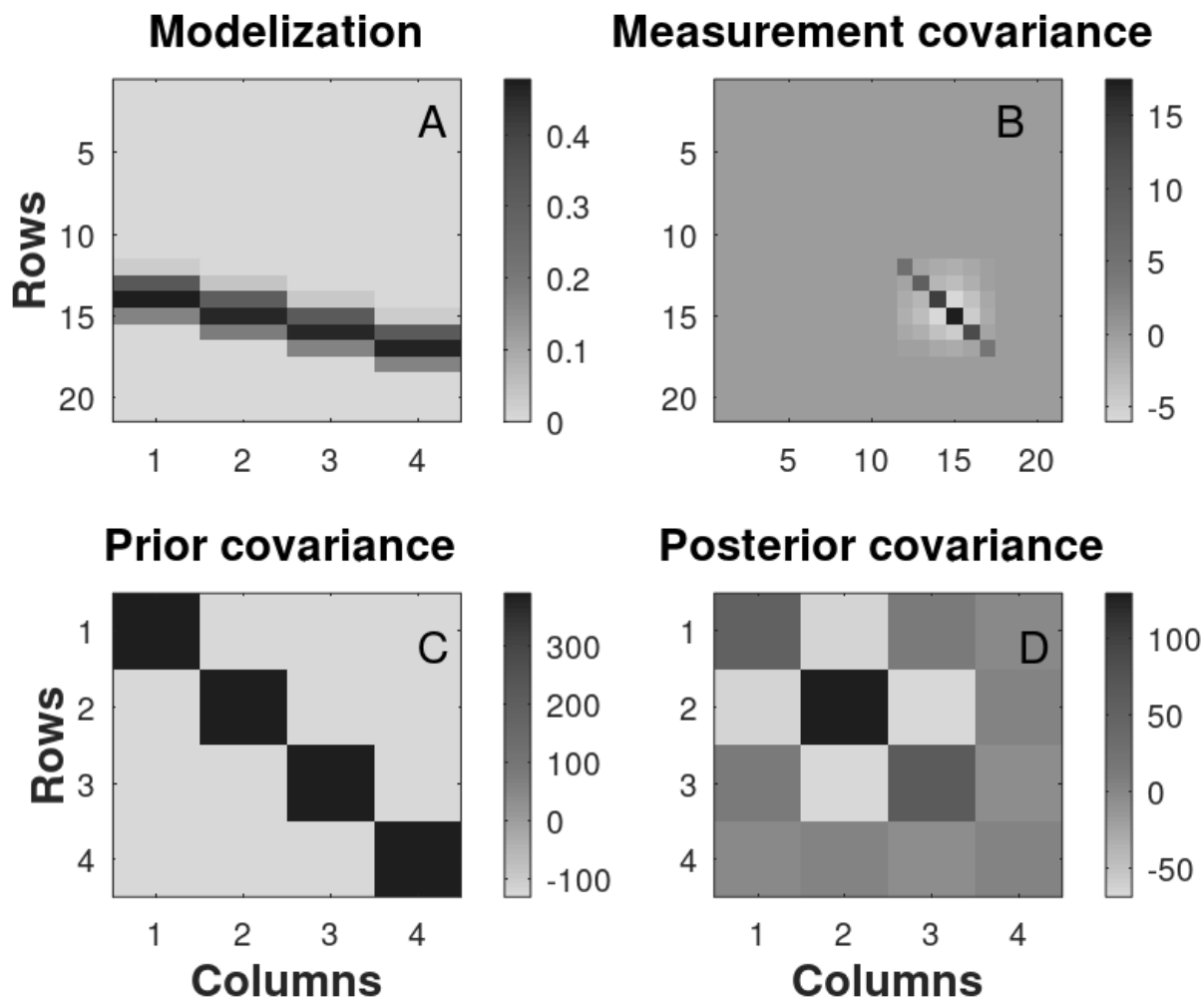
170 Figure 3: Maps of matrixes in Eq. (9). The scale shows the number of tracks. A. The columns of matrix G are normalized histograms derived by interpolating among track length distributions of radiated samples. The track lengths are increasing with row number. The mean value of the c-axis projected tracks is increasing with column number. B. Variance-covariance matrix C_D of the data. The diagonal values are the variances of the measurements calculated by Eq. (D1). The off-diagonal values are covariances of the measurements calculated by Eq. (D2). C. The prior variance-covariance values C_M are calculated by Eq. (D3) and Eq. (D4). D. The variance-covariance of the deconvolved tracks \hat{m} .
