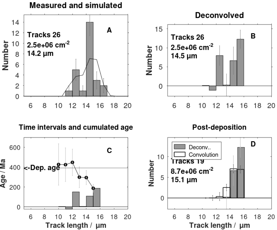
280 Figure 7: A. c-axis projected track histogram of the sandstone sample CXII-48 (Spiegel et al. 2023b) showing a poor simulation match to data probably caused by erroneous data. B. The deconvolution of the histogram shown in A. C. Time intervals and cumulated track ages, showing the presence of inherited tracks.
