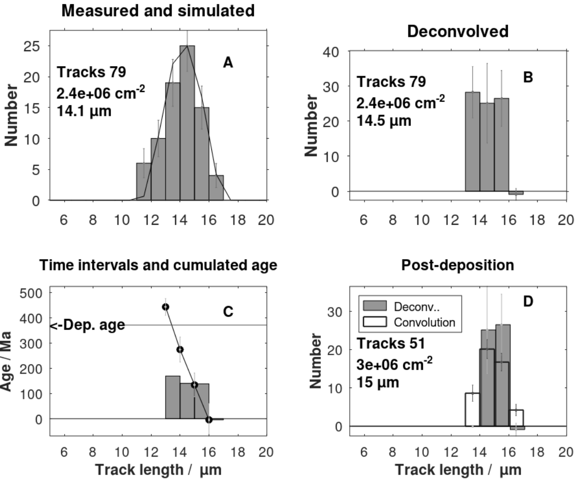
245 Figure 4: A. c-axis projected track histogram of a sandstone sample CXII-46, Spiegel et al. (2023b) together with the simulated distribution. B. Deconvolution of the histogram in A. C. Histogram of time intervals and cumulated track ages. The age nodes (black dots) are the y-values plotted as a function of the c-axis projected track lengths and tabulated in Table 1. D. Deconvolved post-sedimentary tracks and the convolution.
