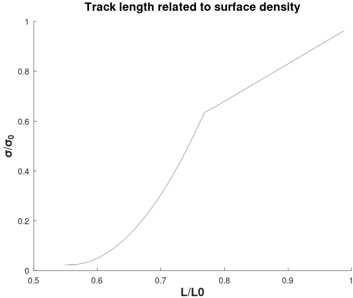
Figure B1: Reduced surface track density \frac{\sigma^i}{\sigma_0^i} as a function of the reduced c-axis projected track length \frac{l^i}{L_0} . The track lengths are c-axis projected. The relations Eq. (B2) and (B3) are approximations to the relation given by Donelick (2026, pers. Comm.).
