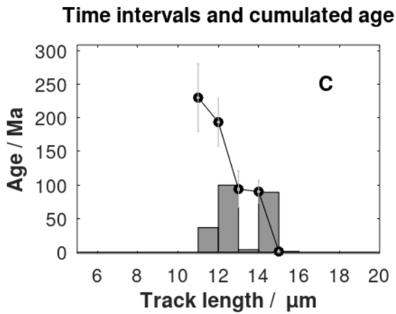
260 Figure 5: A. c-axis projected track histogram for sample GRÖ64 (Spiegel et al., 2023b) and the calculated distribution. B. 265 Deconvolution of the c-axis projected tracks. C. Histogram of time intervals and cumulated track ages. The age nodes (black dots) are the y-values plotted as a function of the c-axis projected track lengths and tabulated in Table 1.
