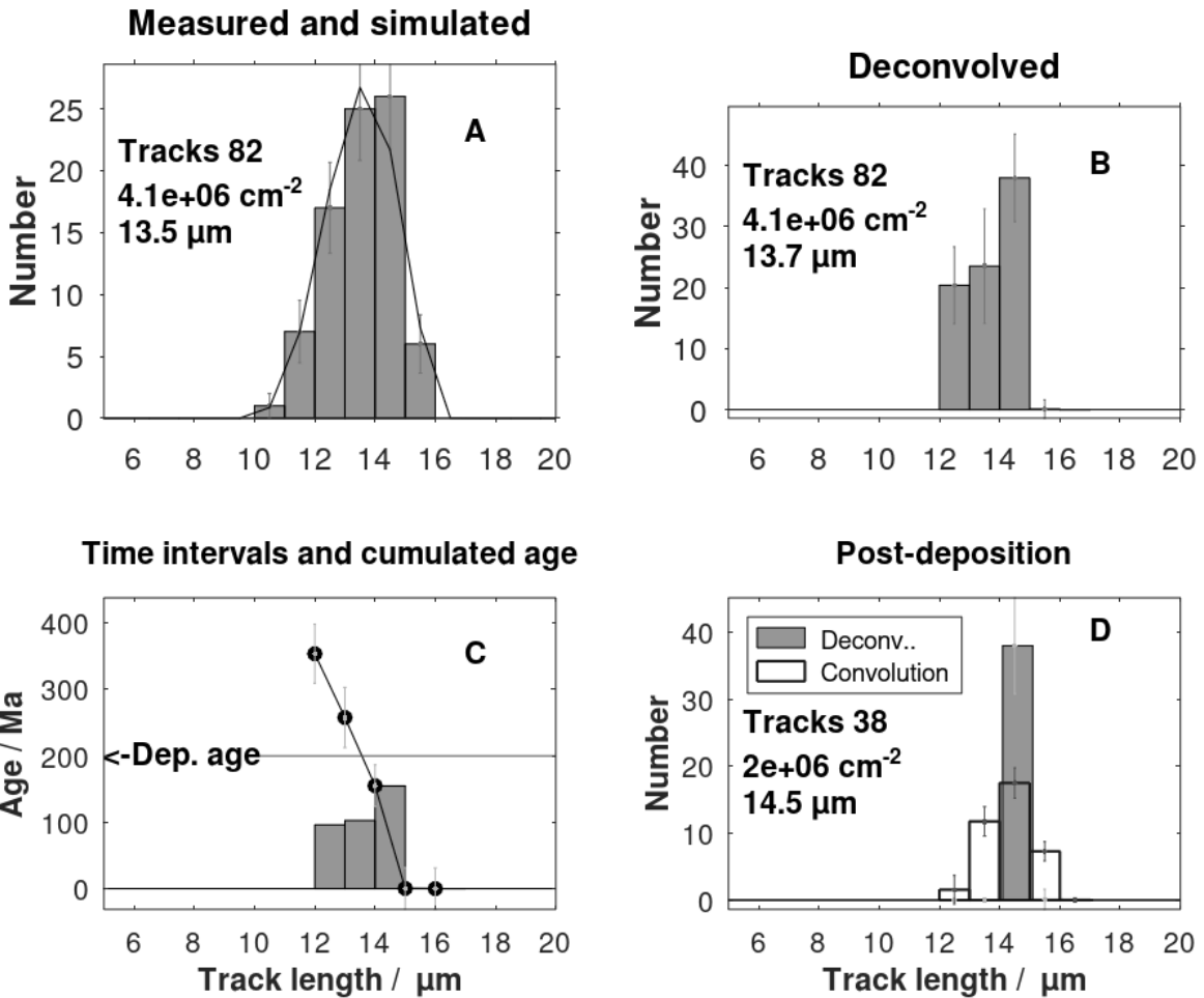
290 Figure 8. A. A skewed data c- axis projected track length histogram sample CXII-42 (Spiegel et al. 2023b). B. The deconvolved track length histogram. C. The sandstone deposition age is used to extract the post-depositional tracks shown in D. D. The deconvolved tracks together with the convolution.
