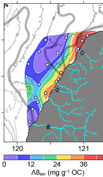
Figure C4: Spatial distribution of \Delta 8_{terr} in seabed sediments of the northeastern Taiwan Strait. White dots mark marine sediment sampling sites, and riverine TSM data (stars) are also shown with colors matching the legend. The thick gray line denotes the boundary (mean grain size = 63 \mu m ; Fig. 1b) of mud belts. Data from Lin et al. (2025a).
