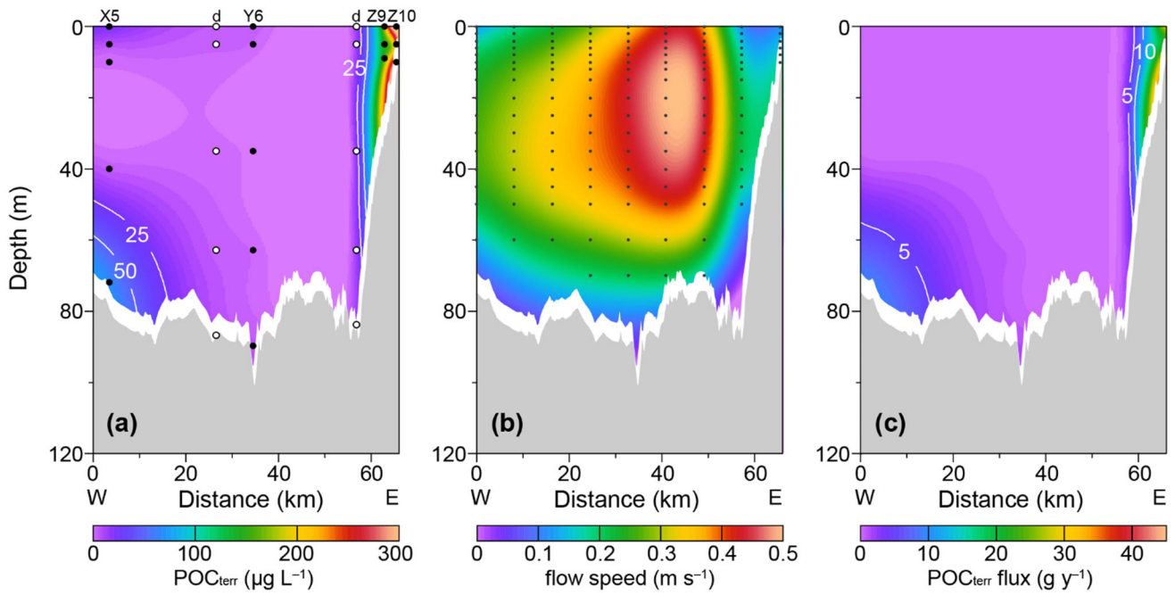
670 Figure C5: Data used for estimating the POC_{terr} export flux. (a) POC_{terr} concentration. Black and white dots are CTD samples and dummy (labeled with d above the frame) stations, respectively. (b) Annual mean flow speed, with black dots marking HYCOM grid points. (c) Calculated POC_{terr} export flux from the northeastern Taiwan Strait. The bottommost 5 m of the water column were excluded from the calculation.
