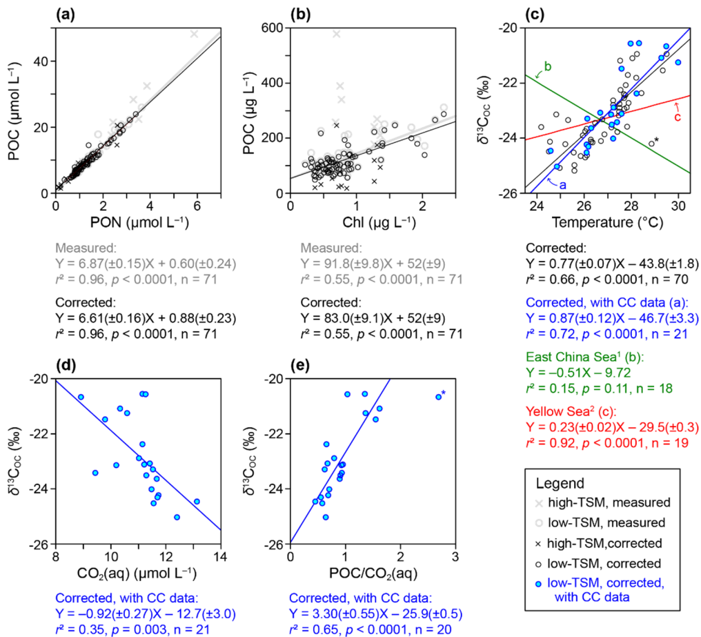
425 Figure 6: Characteristics of marine POM. (a) Relationship between POC and PON. (b) Relationship between POC and Chl. (c) Relationship between \delta^{13}C_{oc} and temperature. (d) Relationship between \delta^{13}C_{oc} and CO_2(aq) . (e) Relationship between \delta^{13}C_{oc} and POC/CO_2(aq) (both in \mu mol L^{-1} ). Linear regressions are based on low-TSM samples only. * denotes data excluded from the regression. References: 1 = Liu et al., 2018a; 2 = Liu et al., 2022.
