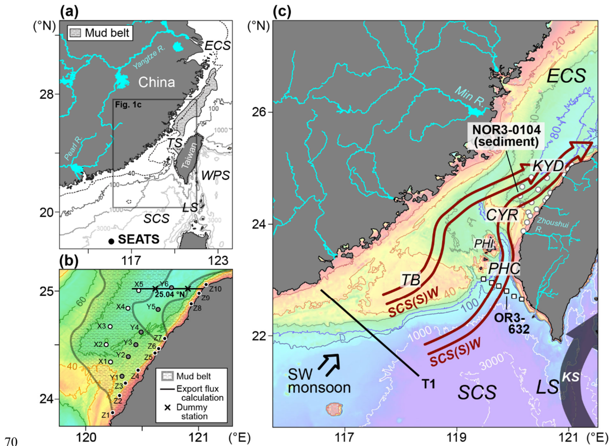
Figure 1: Study area and sampling sites. (a) Study area relative to China and Taiwan. The SEATS station (Liu et al., 2007) is also shown. ECS, East China Sea; LS, Luzon Strait; SCS, South China Sea; TS, Taiwan Strait; WPS, West Philippine Sea. (b) Seawater sampling sites from the cruise NOR3-0104. The extent of mud belts (mean grain size <math>< 63 \mu\text{m}</math>) was based on the isosurface map of sediment grain size (Lin et al., 2025a). (c) Bathymetry and summer flow field (redrawn from Jan et al., 2010). Also shown are seabed sediment sampling sites from cruise NOR3-0104 (Lin et al., 2025a), legacy stations from cruise OR3-632 (Ocean Data Bank, 2025), and Transect T1 from Wong et al. (2015). Bathymetric features: Changyun Rise (CYR), Kuanyin Depression (KYD), Penghu Channel (PHC), Penghu Islands (PHI), and Taiwan Bank (TB), and Wuchiu Depression (WCD) . Currents or water masses: KS, Kuroshio; SCS(S)W, South China Sea (Surface) Water.
