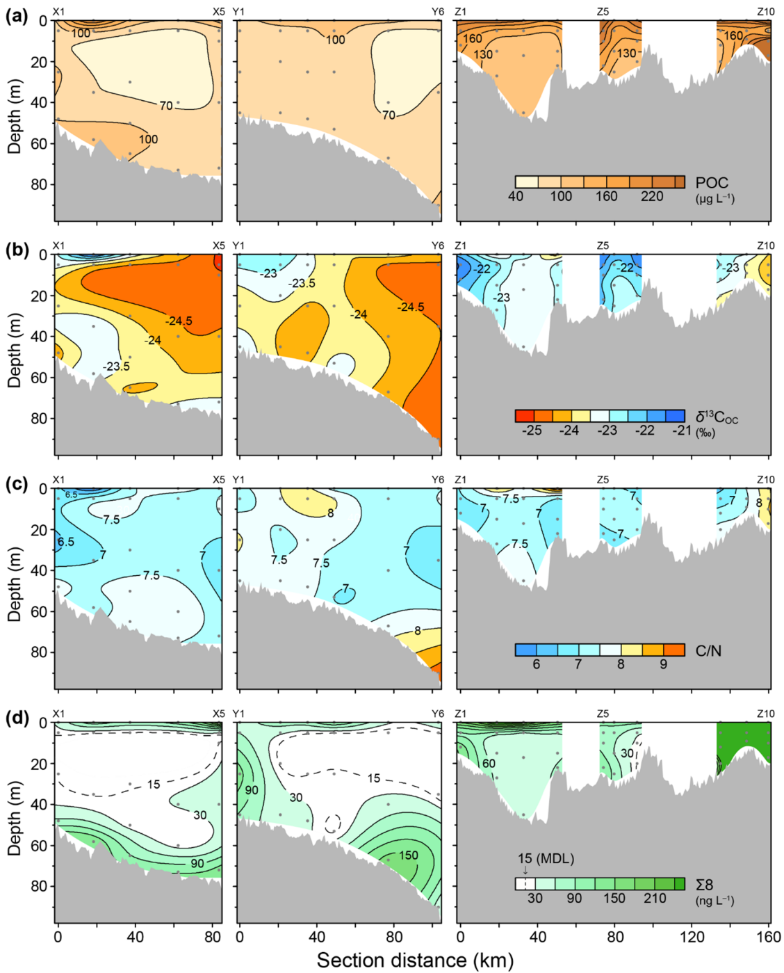
290 Figure 4: POM characteristics along the three transects in the northeastern Taiwan Strait during summer 2022. (a) POC concentrations. (b) \delta^{13}\text{C}_{\text{OC}} values. (c) Atomic C/N ratios. (d) \Sigma 8 concentrations. Grey dots indicate depths for discrete water sampling. MDL, method detection limit.
