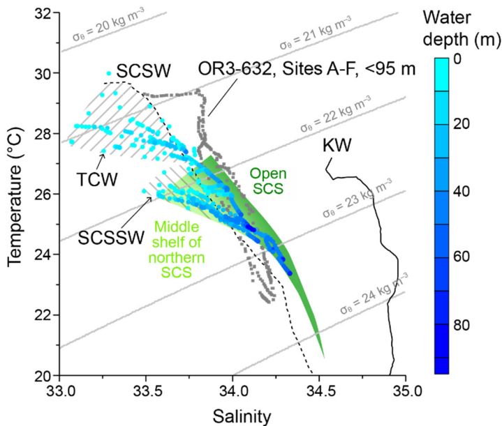
655 Figure C2: Depth-referenced T-S diagram for the NOR3-0104 sampling sites in the northeastern Taiwan Strait. Characteristic summer T-S properties of South China Sea Water (SCSW) and Kuroshio Water (KW) were digitized from Jan et al. (2010). For comparison, T-S properties from Sites A to F of cruise OR3-632 and from Transect T1 (green shade; Wong et al., 2015) are also shown. Light green indicates water properties characteristic of middle-shelf stations in the northern South China Sea (SCS), whereas dark green represents those of open SCS. Samples with salinity lower than typical SCSW values were divided into two groups, one referred to as the Taiwan Coastal Water (TCW) and the other associated with the characteristics of South China Sea Surface Water (SCSSW).
