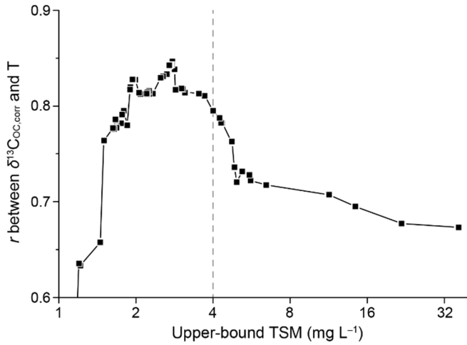
650 Figure C1: Correlation between \delta^{13}\text{C}_{\text{OC,corr}} (from Step 1) and temperature (T) versus the upper-bound TSM in each data subset. The correlation coefficient declined sharply when TSM exceeded 4 \text{ mg L}^{-1} , so this value (dashed gray line) was used to separate low- and high-TSM samples.
