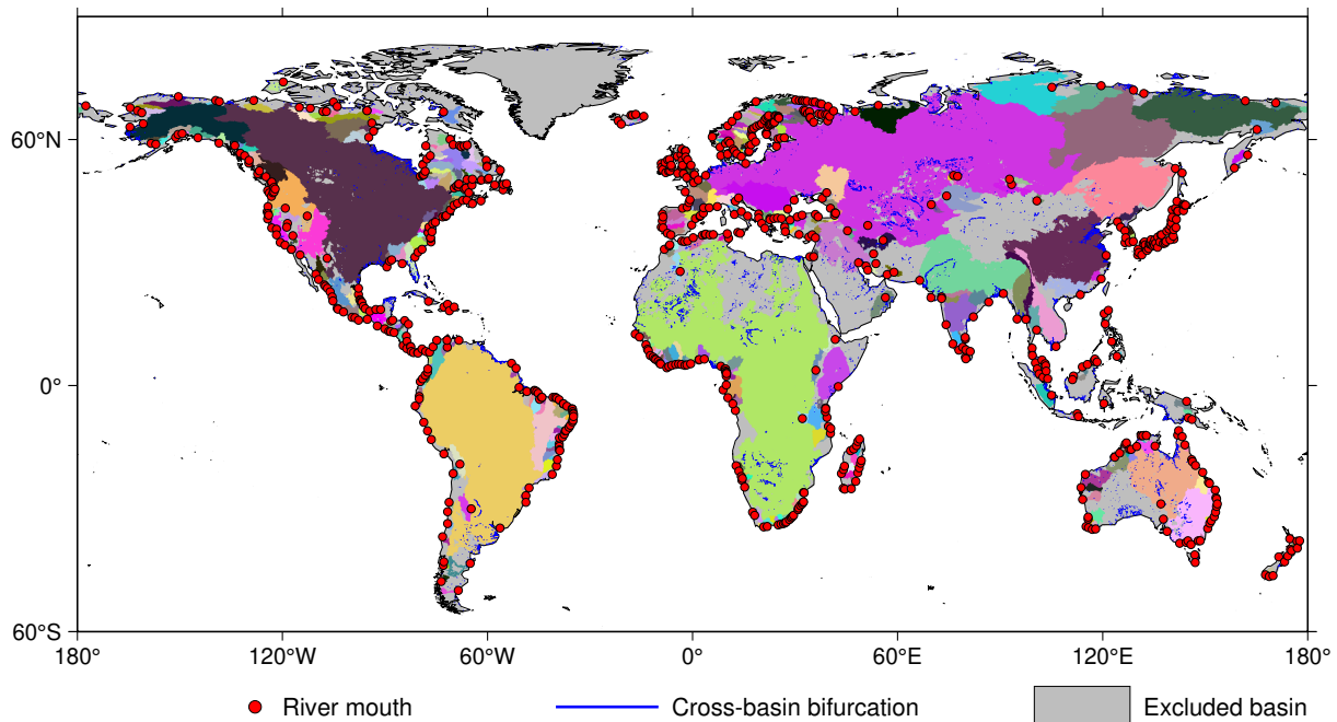
Figure 6. Example of a customized simulation domain constructed from bifurcation-formed basins after the point-of-interest filtering and domain-decomposition-step basin-group domain decomposition. Each The unit-catchment is the computational element; primitive basins are collections of unit-catchments draining to the same river mouth before cross-basin bifurcations are considered. Coloured patches denote retained basin contains-groups, each containing the upstream unit-catchments needed for at least one point of interest. Coloured patches denote the retained basins, while grey areas mark basins excluded from the selected domain; markers basin groups. Some retained patches are spatially large because a downstream point of interest can require preserving an entire upstream primitive basin, and cross-basin bifurcation links can merge several primitive basins into one basin group. Markers indicate river-mouth locations and blue lines denote cross-basin bifurcation links.
