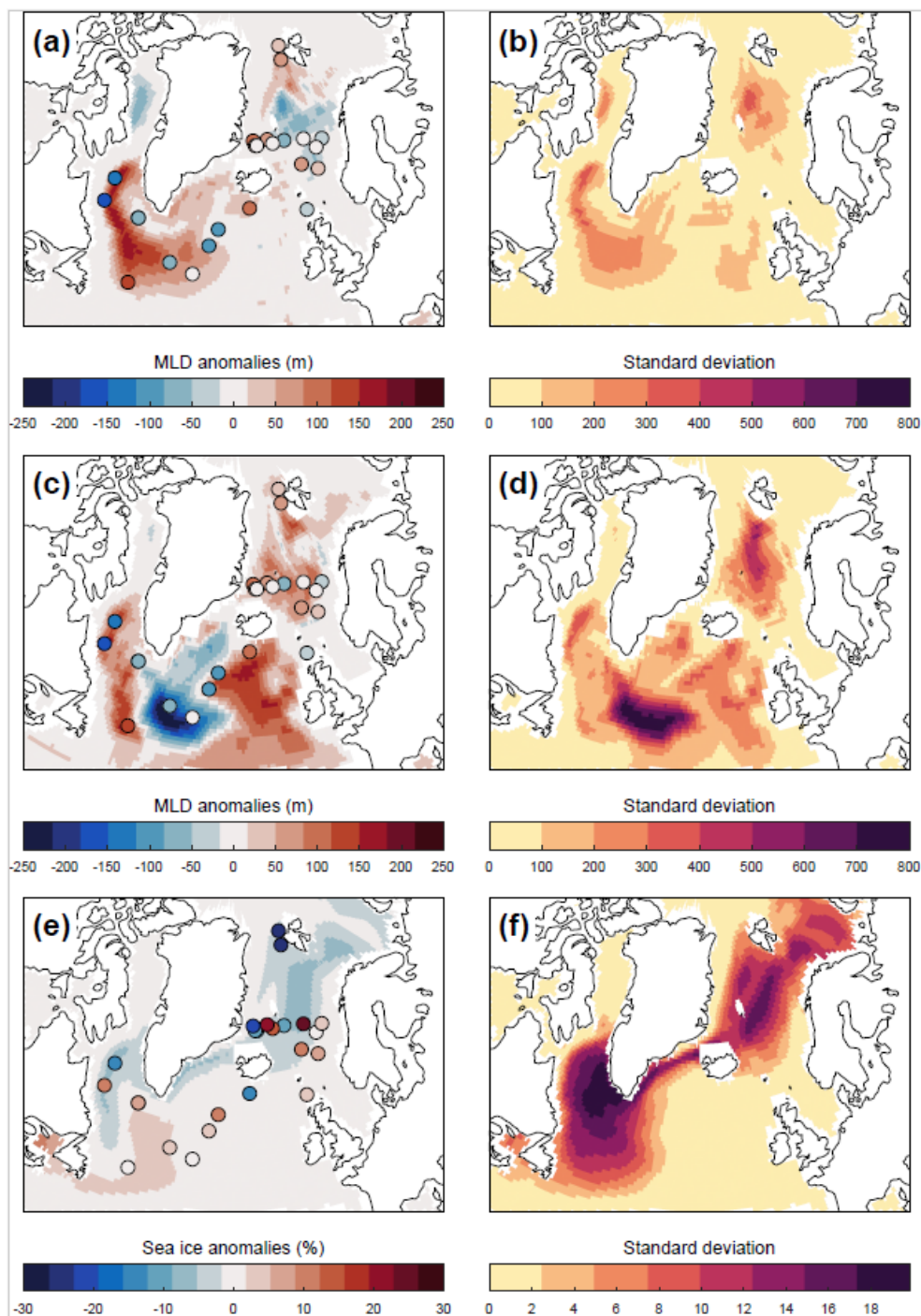
220 Figure 5. Winter (Jan-Mar) MLD anomalies (MH-PI) from the PMIP4 (a) and PMIP3 (c) model ensemble mean (background) versus proxy data (dots). Note that two of the four sites in the Labrador Sea are located very close to each other and hence superimposed in the figure. The inter-model spread is defined as the standard deviation across the PMIP4 (b) and PMIP3 (d) ensembles. (e, f) Winter (Jan-Mar) sea ice anomalies (MH-PI) from the PMIP4 ensemble mean versus proxy data and the inter-model spread.
