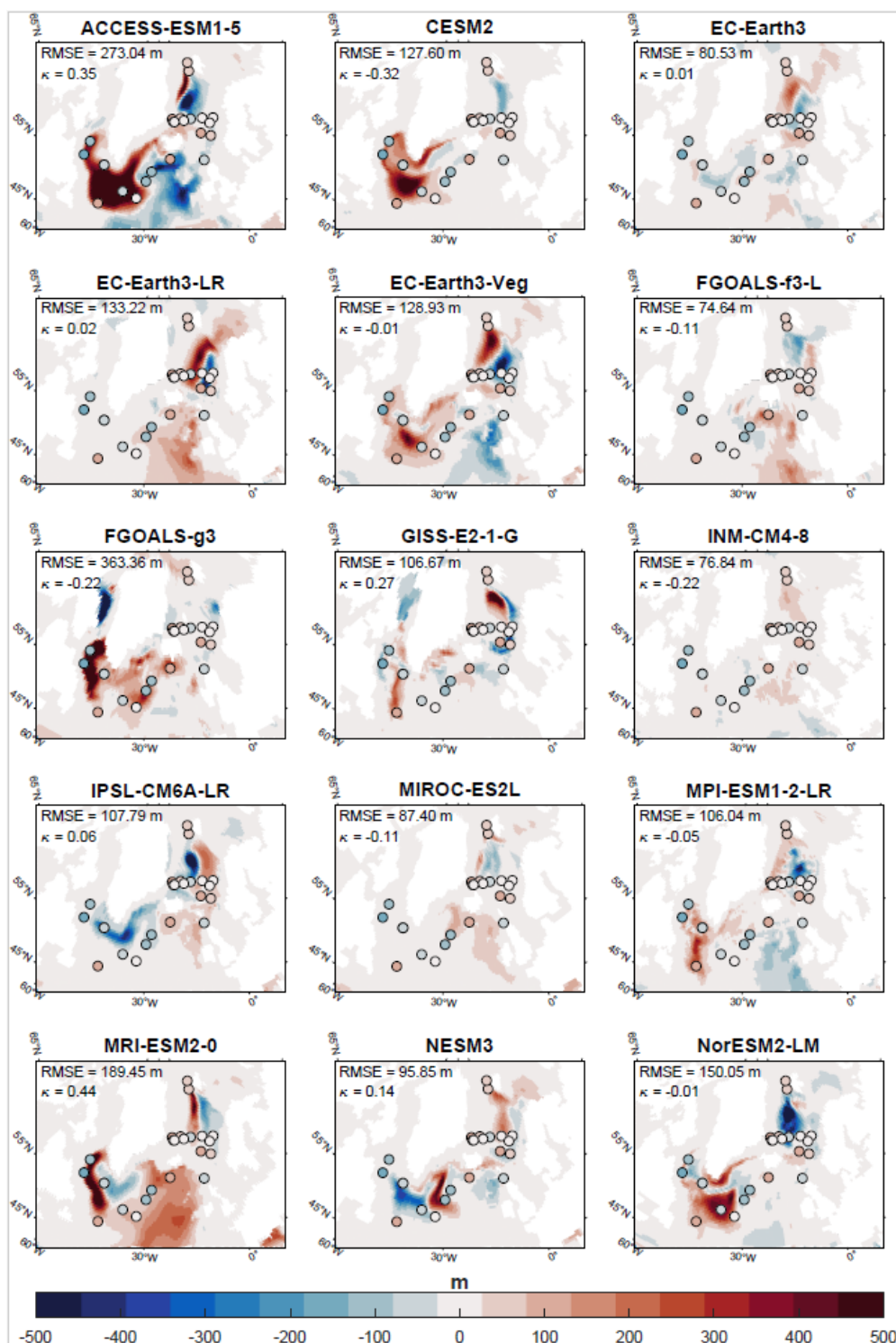
170 Figure 1. Winter MLD anomalies (MH-PI) as the average of January to March in the North Atlantic from the PMIP4 ensemble (background) versus proxy data (dots).
