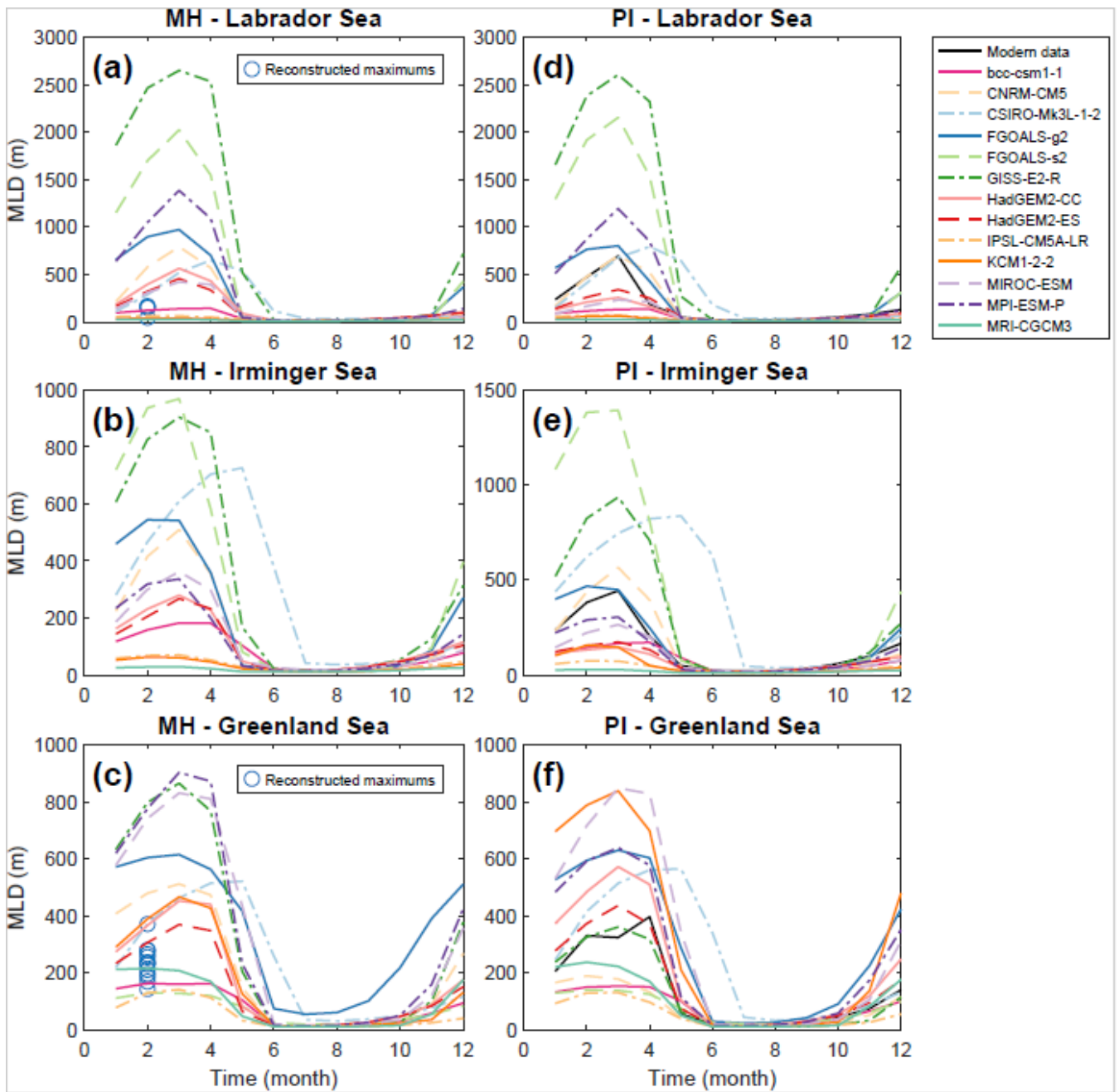
175 Figure 4. Seasonal cycle of MLD in three deep-water formation regions from the modern climatology of de Boyer Montégut (2023) and PMIP3 model simulations of MH (a-c) and PI (d-f). The reconstructed maximums in the MH panel correspond to the maximum winter (Jan-Mar) MLD reconstructed over the MH interval in nearby dinocyst records, where available. For a map of the three regions as defined by Treguier et al. (2023), see Fig. S1.
