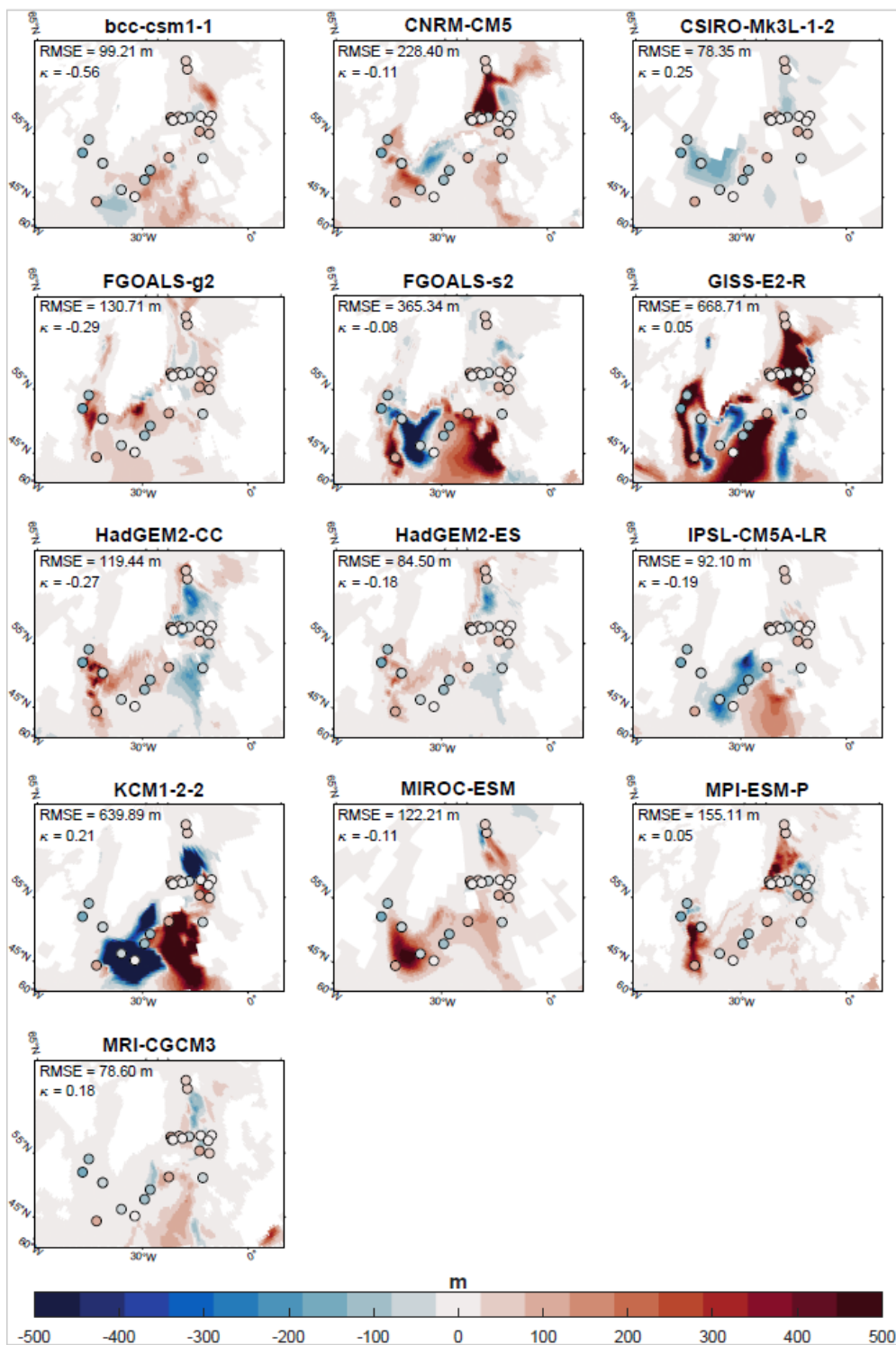
175 Figure 2. Winter MLD anomalies (MH-PI) as the average of January to March in the North Atlantic from the PMIP3 ensemble (background) versus proxy data (dots).
