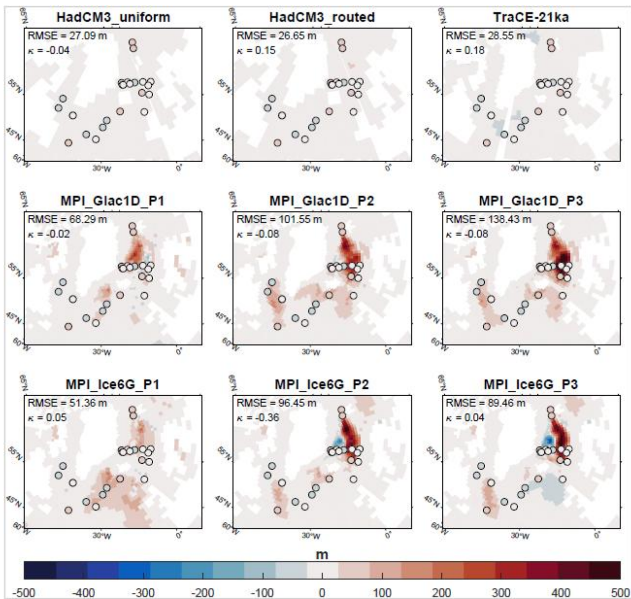
Figure 7. Annual MLD anomalies (MH-PD) in the North Atlantic from the PMIP4 last deglaciation simulations (background) versus proxy data (dots).
