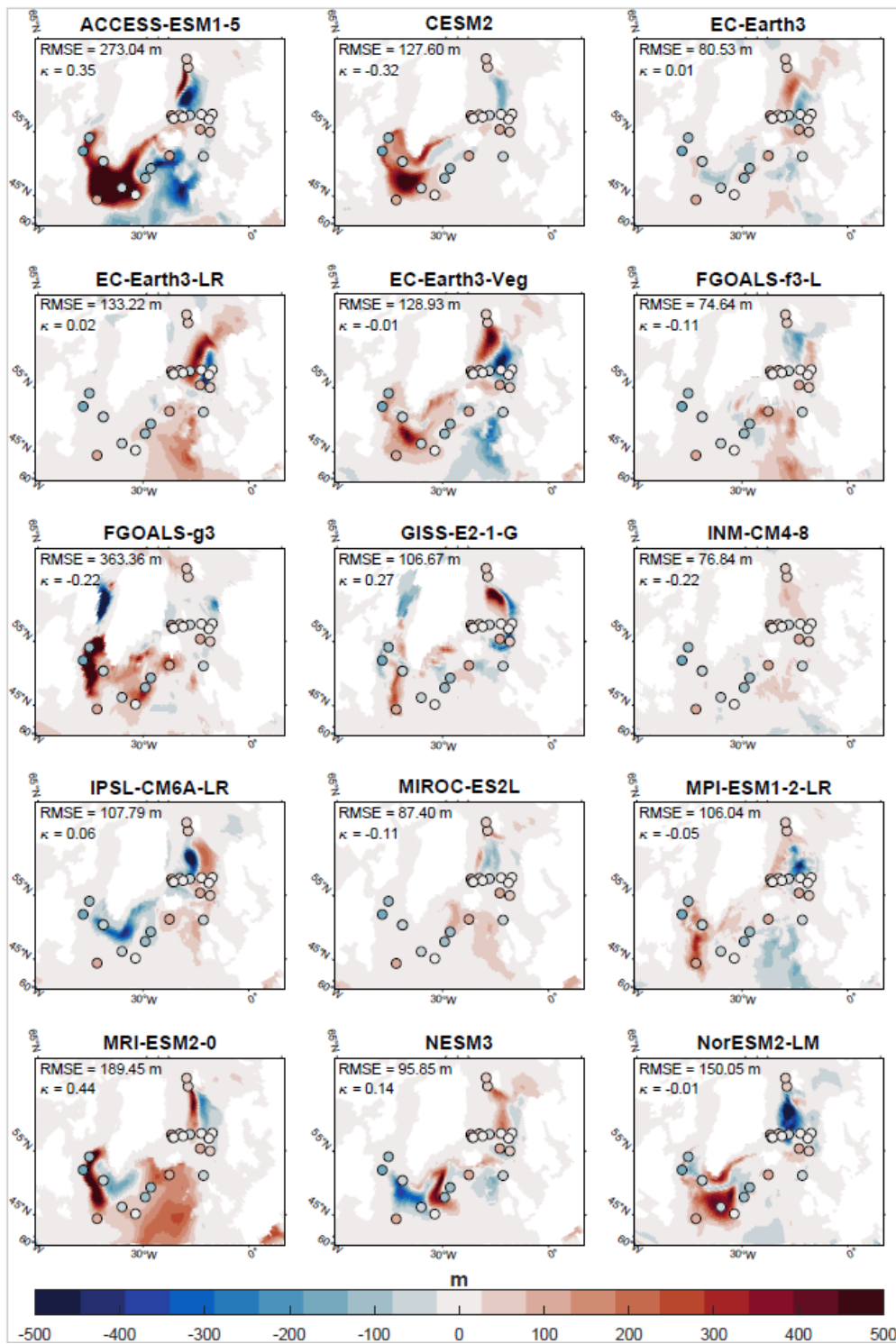
Figure 1. Winter MLD anomalies (MH-PI) as the average of January to March in the Northern Hemisphere and the average of July to September in the Southern Hemisphere North Atlantic from the PMIP4 ensemble (background) versus proxy data (dots).
