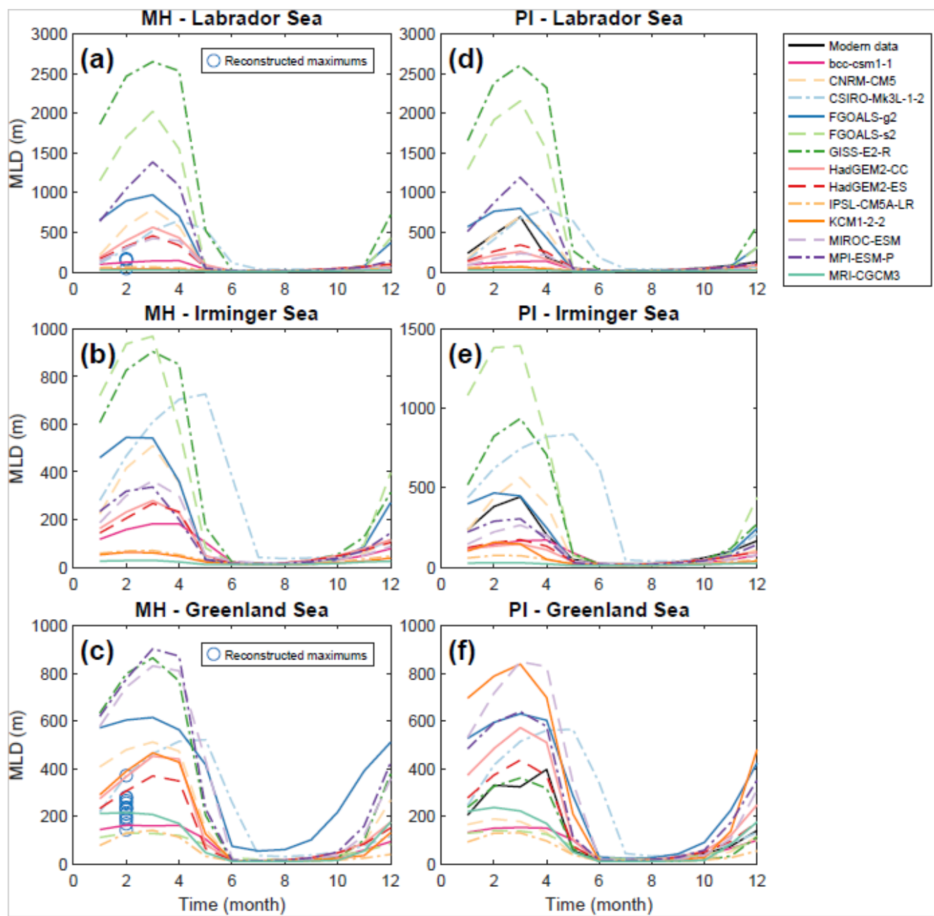
185 Figure 4. Seasonal cycle of MLD in three deep-water formation regions from the modern climatology of de Boyer Montégut (2023) and PMIP3 model simulations of MH (a-c) and PI (d-f). The reconstructed maximums in the MH panel correspond to the maximum winter (Jan-Mar) MLD reconstructed over the MH interval in nearby dinocyst records, where available. For a map of the three regions as defined by Treguier et al. (2023), see Fig. S1.
