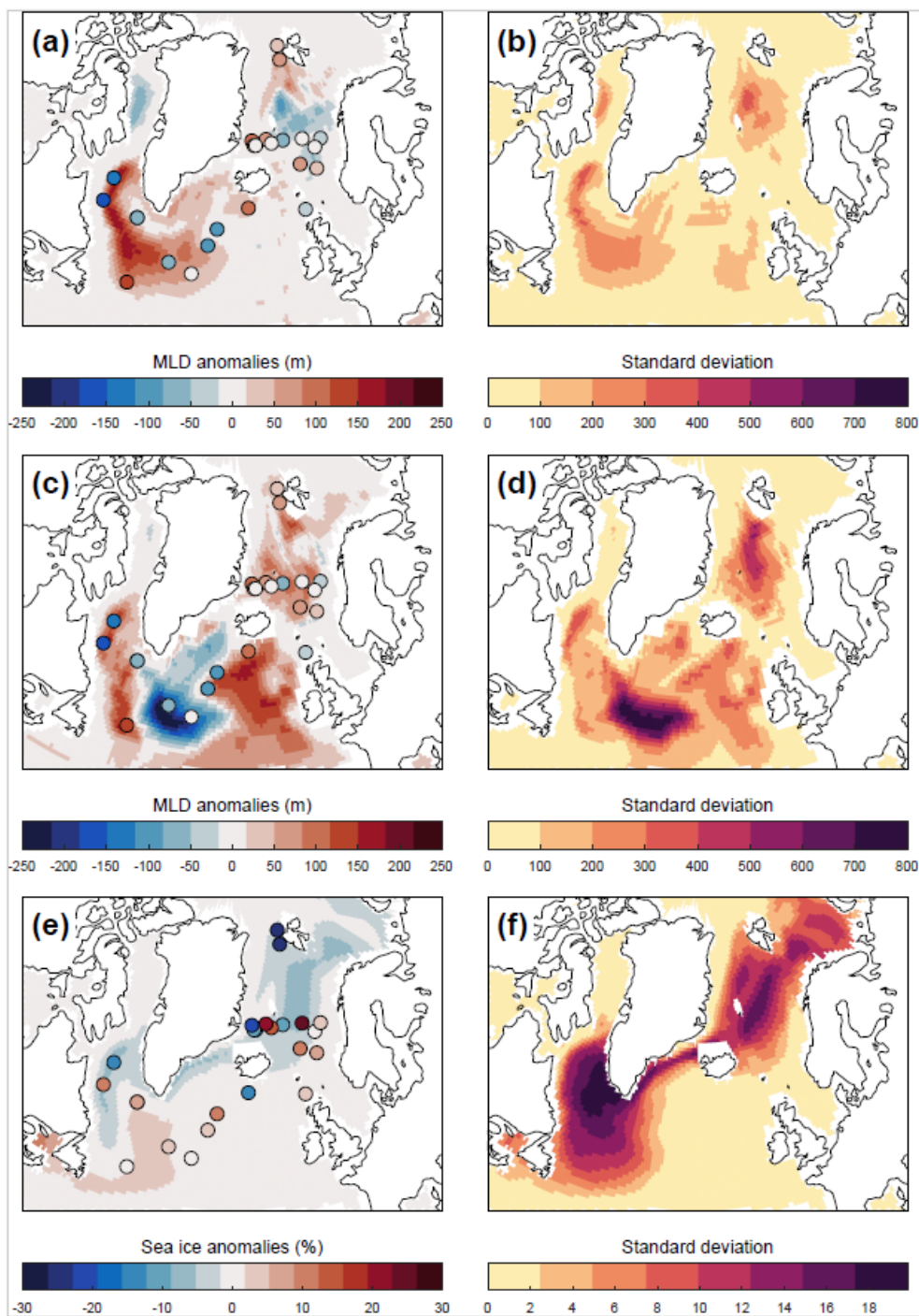
Figure 35. (a) Winter (January to March) MLD anomalies (MH-PI) from the PMIP4 (a) and PMIP3 (c) model ensemble mean (background) versus proxy data (dots). Note that two of the four sites in the Labrador Sea are located very close to each other and hence superimposed in the figure. (b) The inter-model spread is defined as the standard deviation across the PMIP4 (b) and PMIP3 (d) ensembles. (e, f) Winter (Jan-Mar) sea ice anomalies (MH-PI) from the PMIP4 ensemble mean versus proxy data and the inter-model spread.
