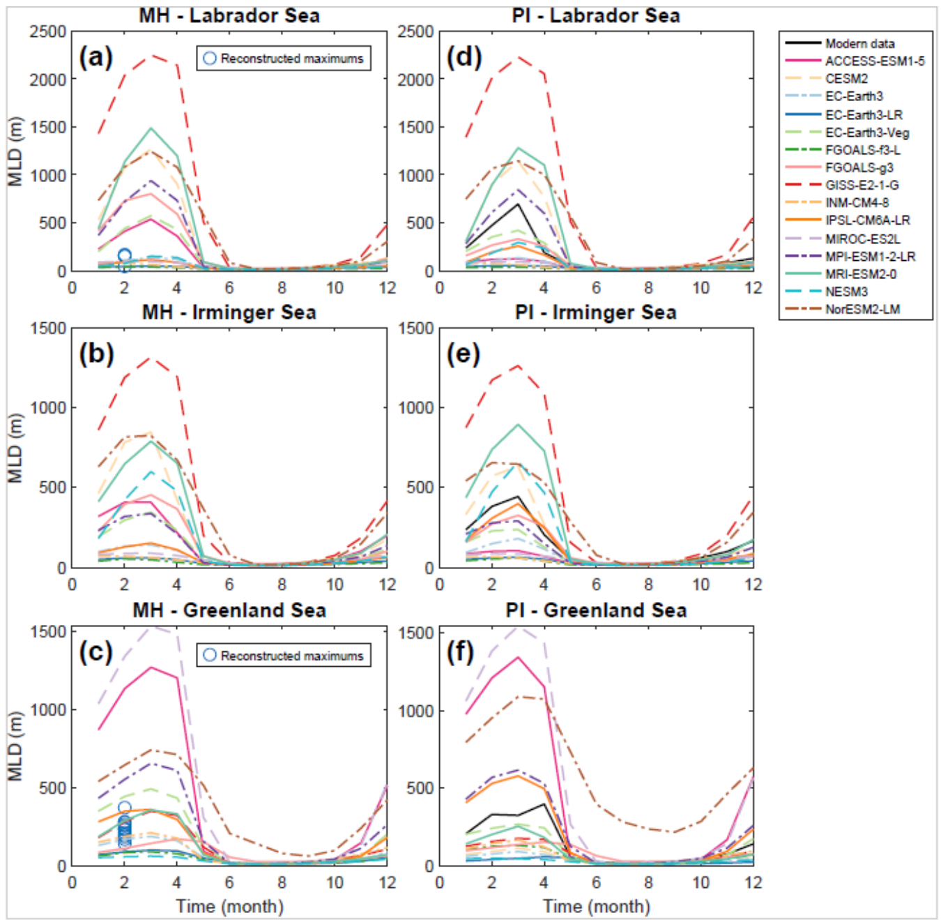
Figure 23. Seasonal cycle of MLD in three deep-water formation regions from the modern climatology of de Boyer Montégut (2023) and PMIP4 model simulations of MH (a-c) and PI (d-f). The reconstructed maximums in the MH panel correspond to the maximum winter (Jan-Mar) MLD reconstructed over the MH interval in nearby dinocyst records, where available. For a map of the three regions as defined by Treguier et al. (2023), see Fig. S1.
