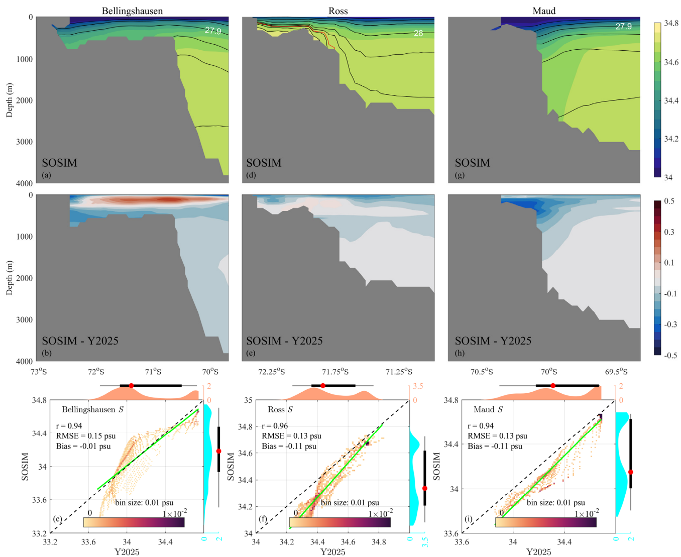
Figure 20. As in Fig. 19, but for S (psu), with the red line denoting the \gamma^m contour of 28.27 \text{ kg m}^{-3} .
