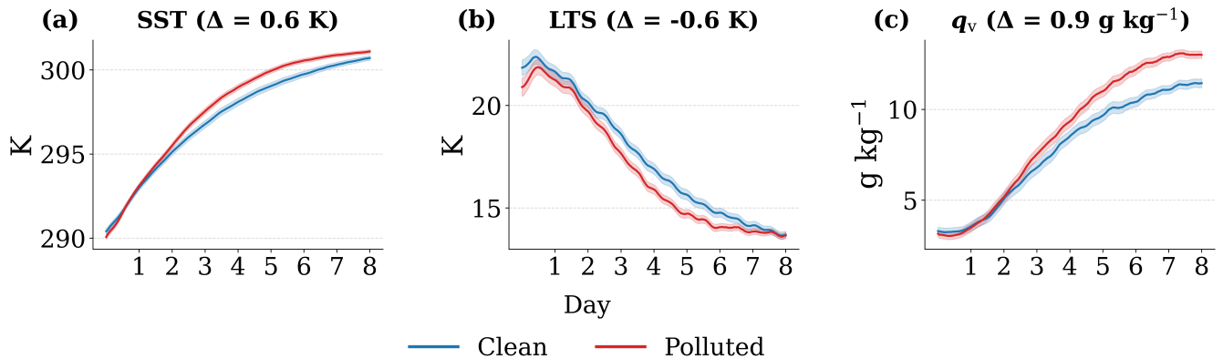
Figure 3. Hourly mean evolution of environmental variables from MERRA-2 reanalysis data along Lagrangian trajectories for the NEP1 initial location (starting from 34.0^{\circ}\text{N} , 125.0^{\circ}\text{W} ), separated into clean (blue) and polluted (red) groups. Shown are: (a) sea surface temperature (SST), (b) lower-tropospheric stability (LTS), and (c) specific humidity at 850 hPa ( q_v , 850 hPa). Solid lines represent group means, shaded regions represent two-sided 95% confidence intervals for the mean, computed as \text{mean} \pm 1.96 \times \text{SEM} (standard error of the mean) across trajectories at each hour. The time-mean differences between the polluted and clean trajectories are shown in parentheses above each panel. The rest of the initial locations are presented in Figures S2-S9, SI.
