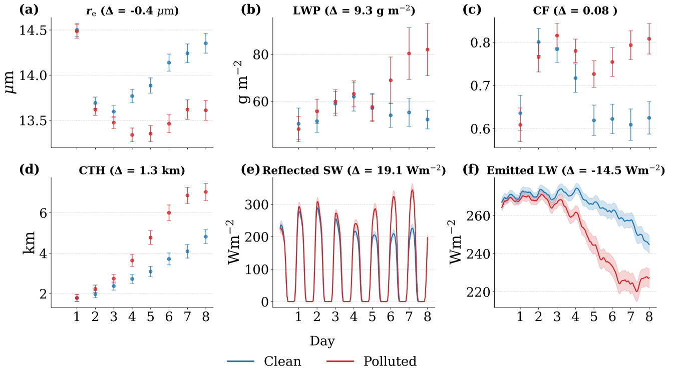
Figure 4. Mean evolution of cloud and radiation properties along Lagrangian trajectories for the NEP1 initial location (starting from 34.0^{\circ}\text{N} , 125.0^{\circ}\text{W} ), separated into clean (blue) and polluted (red) groups. Panels (a–d) show daily means; panels (e–f) show hourly values. Shown are: (a) cloud droplet effective radius ( r_e ), (b) liquid water path (LWP), (c) total cloud fraction (CF), (d) cloud top height (CTH), (e) reflected short-wave radiation at Top-Of-Atmosphere top of atmosphere (FOA; Reflected SW; TOA), and (f) emitted longwave radiation at TOA (Emitted LW). Panels a, e-f are based on CERES data, while panels b-d are based on MODIS data. Solid lines represent group means, shaded regions and error bars represent two-sided 95% confidence intervals for the mean, computed as \text{mean} \pm 1.96 \times \text{SEM} (standard error of the mean) across trajectories at each point in time. The time-mean differences between the polluted and clean trajectories are shown in parentheses above each panel. The rest of the initial locations are presented in Figures S10-S17, SI.
