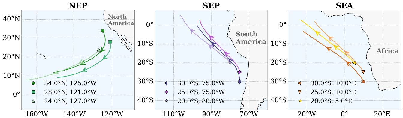
Figure 1. Mean trajectory paths across the three ocean basins: (a) Northeast Pacific (NEP), (b) Southeast Pacific (SEP), and (c) Southeast Atlantic (SEA). Each colored line represents the average trajectory path initiated from a distinct starting point, marked by a unique symbol, with arrows indicating the direction of propagation with the trade winds.
