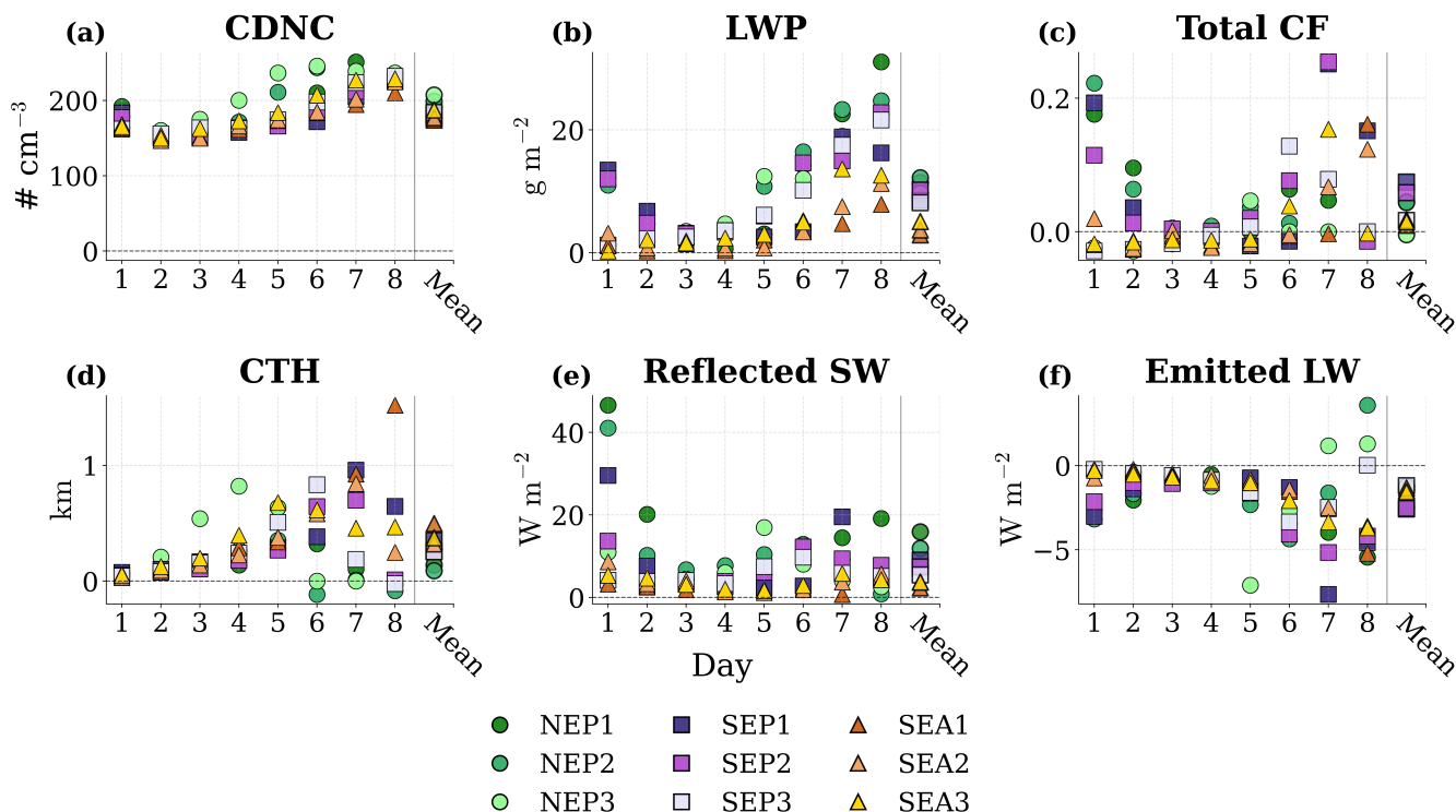
Figure 8. Daily mean differences between polluted and clean trajectory groups for all nine initiation locations (NEP1–NEP3, SEP1–SEP3, SEA1–SEA3) from model simulations. Panels show: (a) Domain-domain mean cloud droplet number concentration ( N_d ) (b) liquid water path (LWP), (c) total cloud fraction (CF), (d) cloud top height (CTH), (e) reflected shortwave radiation at FOA-top of atmosphere (Reflected SW; TOA ), and (f) emitted longwave radiation at TOA (Emitted LW). Marker shapes and colors indicate the location: circles (NEP), squares (SEP), and triangles (SEA). The “Mean” column indicate the time-mean difference across all days.
