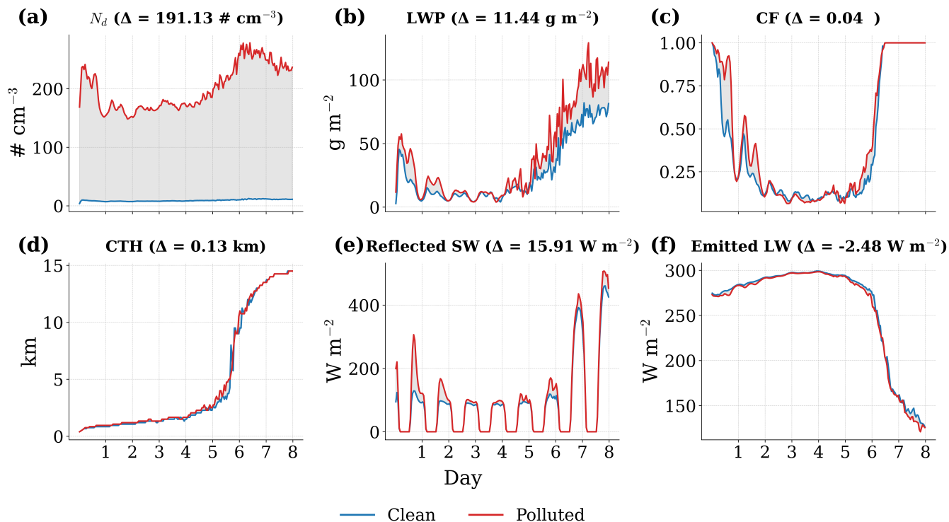
Figure 7. Hourly mean evolution of cloud and radiation variables from the model simulations for the NEPI initial location as an example, separated into clean (blue, 20 \text{ cm}^{-3} ) and polluted (red, 800 \text{ cm}^{-3} ) simulations. Panels show: (a) Domain mean cloud droplet number concentration ( N_d ), (b) liquid water path (LWP), (c) total cloud fraction (CF), (d) cloud top height (CTH), (e) reflected shortwave radiation at Top-Of-Atmosphere top of atmosphere (TOA) (Reflected SW; TOA), and (f) emitted longwave radiation at TOA (Emitted LW). The time-mean differences between the polluted and clean simulations are shown in parentheses above each panel. The rest of the initial locations are presented in Figures S44-S51, SI.
