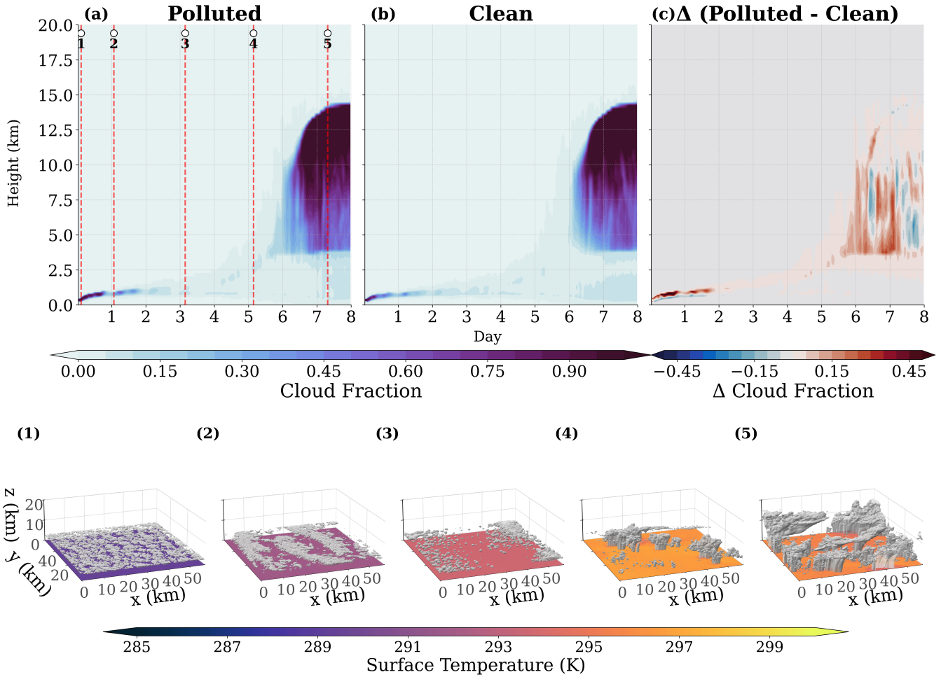
Figure 6. Hovmöller diagrams of cloud fraction evolution from model simulations for the NEPI initial location, for the different simulated cases: (a) polluted simulation, (b) clean simulation, and (c) the difference between them (polluted — clean). Panels (a) and (b) show cloud fraction as a function of height and time for the polluted and clean simulations, respectively , while panel (c) shows the corresponding difference field , with red indicating higher cloud fraction in the polluted case and blue indicating higher cloud fraction in the clean case between them . Color scales are shown below each set of panels. The bottom row (1–5) shows 3D cloud fields at selected timesteps corresponding to markers in panel (a), illustrating the temporal evolution of cloud structure from early development to mature convection. Color scales for cloud fraction and surface temperature are shown alongside each plot. The rest of the initial locations are presented in Figures S35–S42 S36–S43 , SI.
