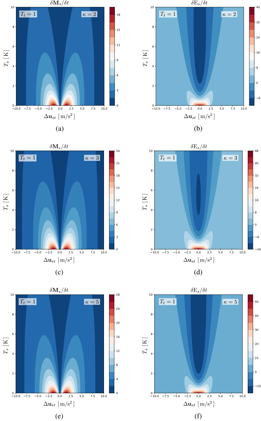
Figure 6. (a, c, e) The momentum collision term in units of [\text{N}/\text{m}^3] , and (b, d, f) the energy collision term in units of [\text{W}/\text{m}^3] for the standard Kappa velocity distribution in the case of Coulomb collisions at different values of \kappa : 2, 3, and 5.
