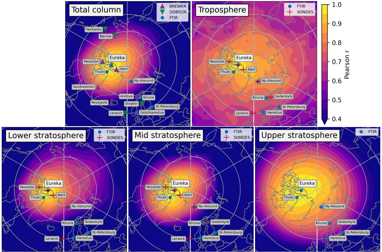
Figure 10. Correlation of CAMS deseasonalized anomalies at the location of the Eureka station with CAMS anomalies in the rest of the Arctic. Stations where a ground-based instrument is used in the corresponding partial column are indicated.
