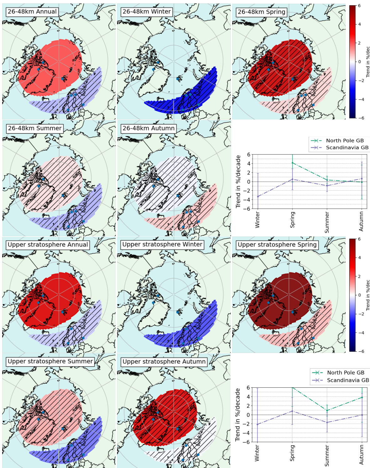
Figure 17. Same as Figure 14 for the upper stratospheric columns ozone trends. Exact trend values and their 2\sigma uncertainties are displayed in the Appendix in Table D3.
