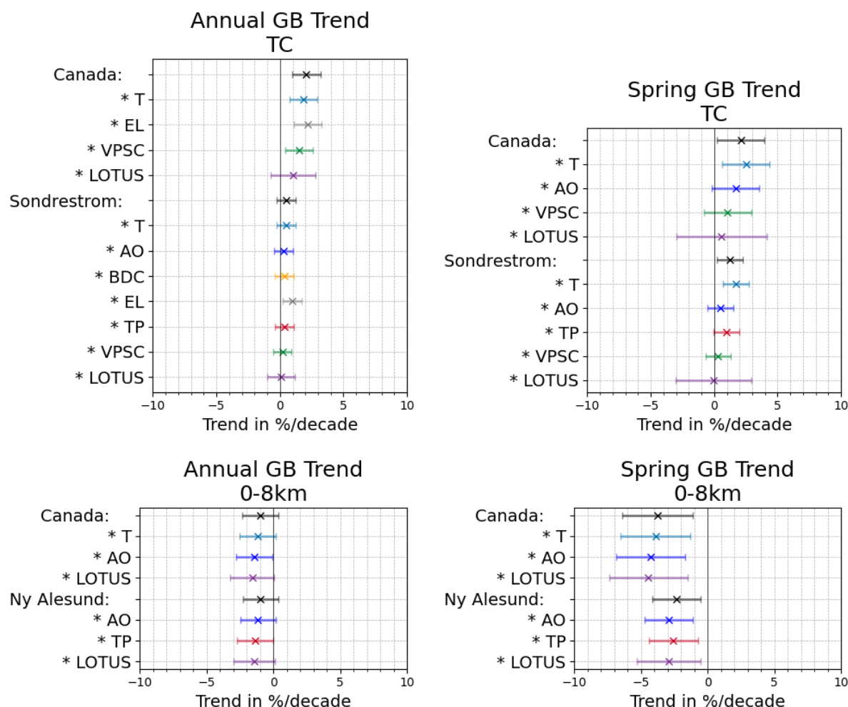
Figure C1. Effect of detrending each non-LOTUS proxies on trends in Canada (a region with many merged instruments), in Sondrestrom for the total column and in Ny-Ålesund for partial columns, two single-site regions. Shown here for the total column and the troposphere. Stratospheric partial column trends are in the next figure. For each column and annual/Spring trends, we only show the detrending of proxies that are effectively contributing, to avoid unnecessary clutter. For comparison, we also show the LOTUS proxies-only trends, which always have a larger uncertainty since less variability is explained, leading to non-significant trends everywhere.
