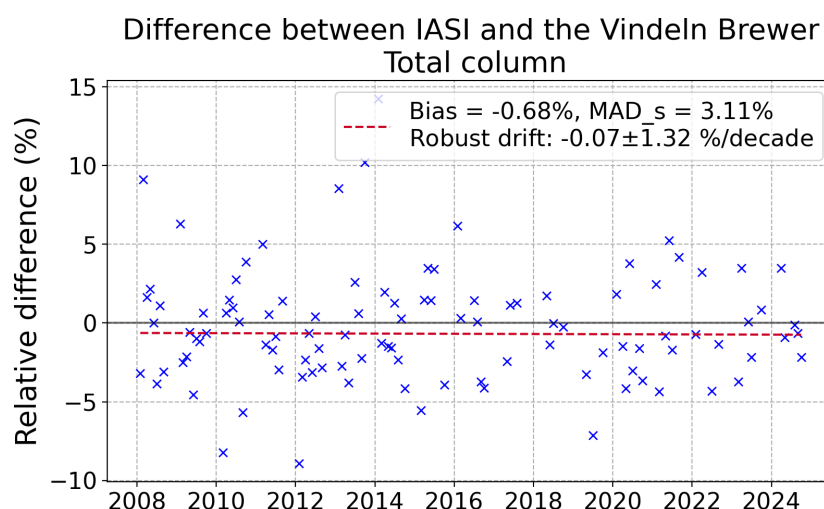
Figure 2. Difference of relative anomalies in percent \text{diff}_{\text{sat-GB}}^i (4) between the Vindeln Brewer total column and the IASI-CDR total column in Vindeln with associated bias, \text{MAD}_s and drift with 2\sigma -error. The presence of several strong outliers requires the use of a robust regression method, here the Theil-Sen method.
