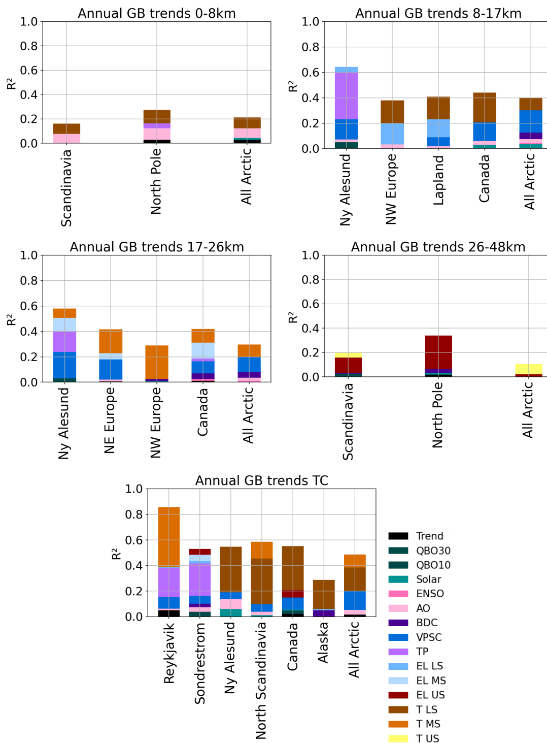
Figure 13. R^2 with individual contributions of proxies for all annual trends of ground-based instruments merged anomalies data sets for partial and total columns of ozone.
