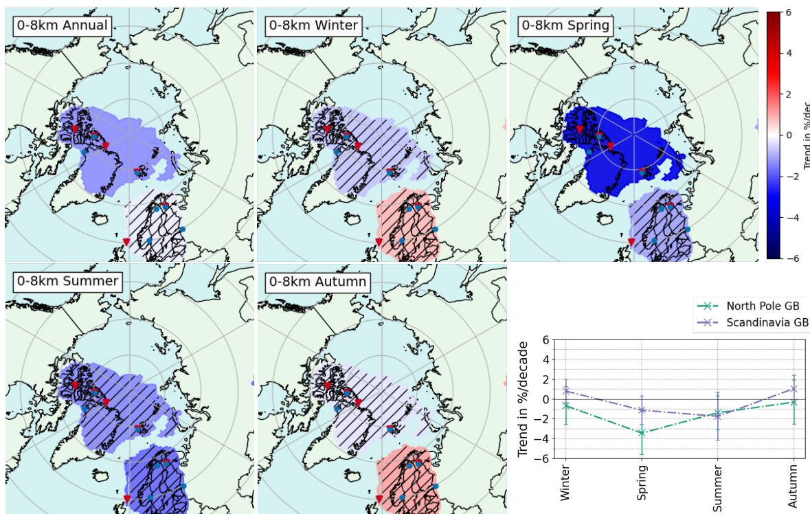
Figure 18. Same as Figure 14 for the tropospheric ozone trends. Exact trend values and their 2\sigma uncertainties are displayed in the Appendix in Table D2.
