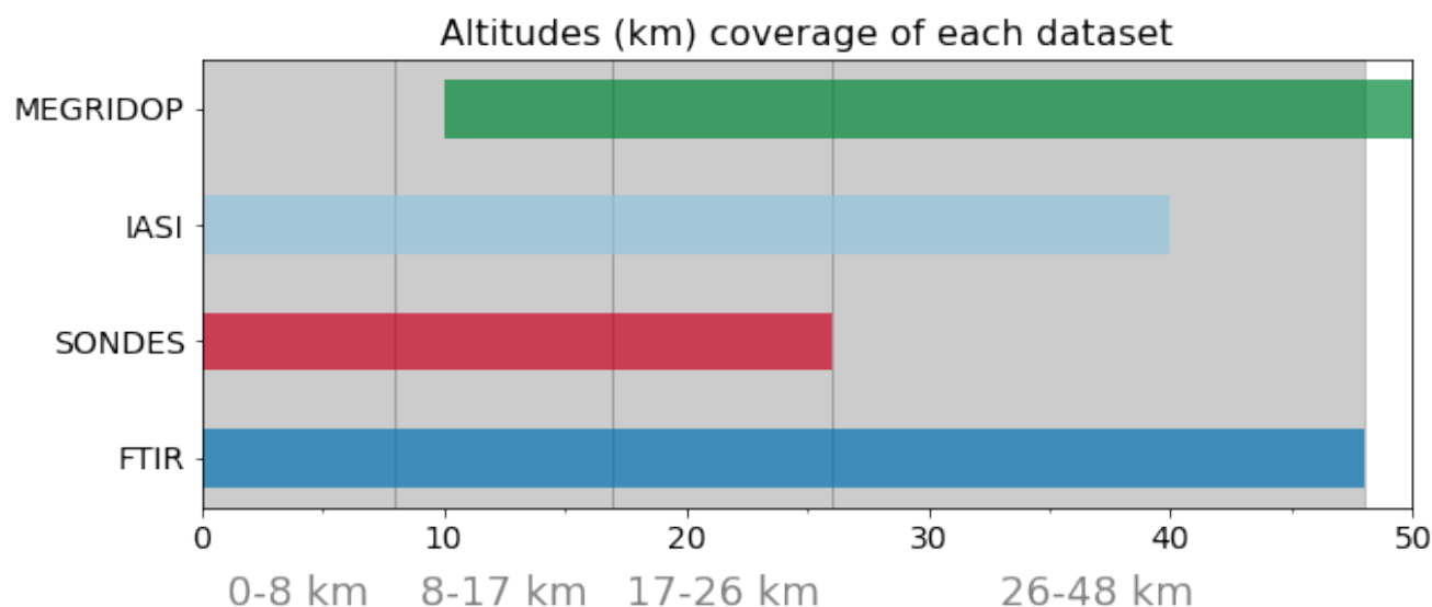
Figure 3. Vertical coverage of each profile data sets used in this study against our choice for partial columns altitude boundaries. This choice is explained in section 2.4.
