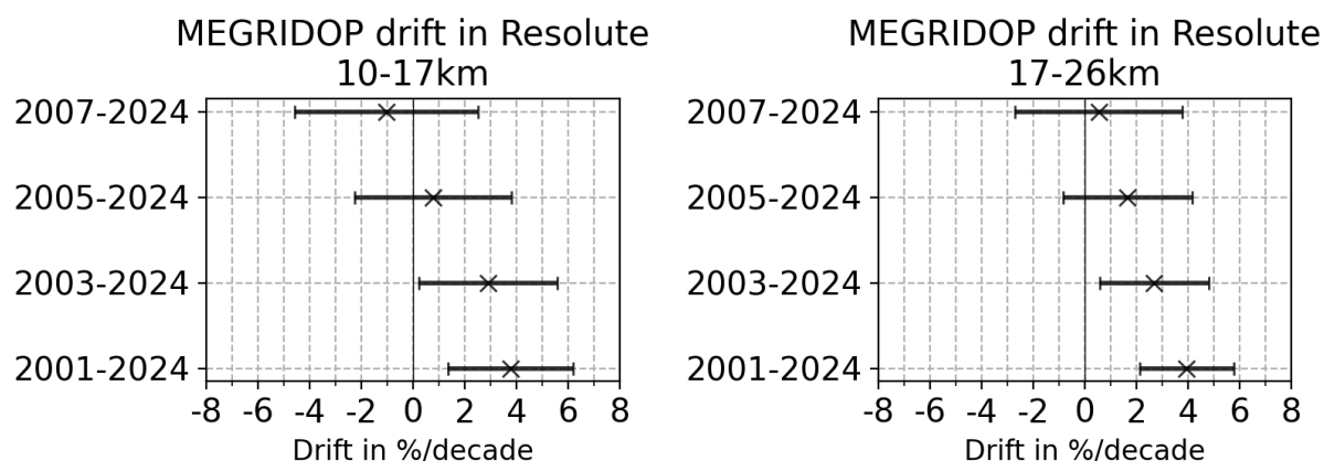
Figure 7. Variation of the drift of MEGRIDOP with respect to the Resolute sonde in lower and mid-stratosphere depending on the starting date of comparison.
