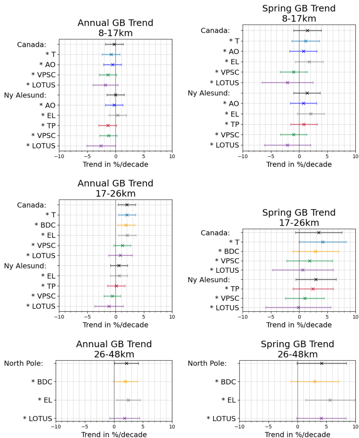
Figure C2. Same as C1 for middle and upper stratospheric columns.
