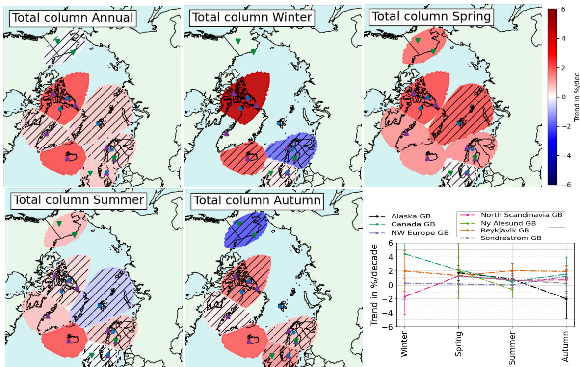
Figure 14. Annual and seasonal regional trends maps for the total column of ozone. Black hatches mean the trends are not significant. Exact trend values and their 2\sigma uncertainties are displayed in the Appendix in Table D1.
