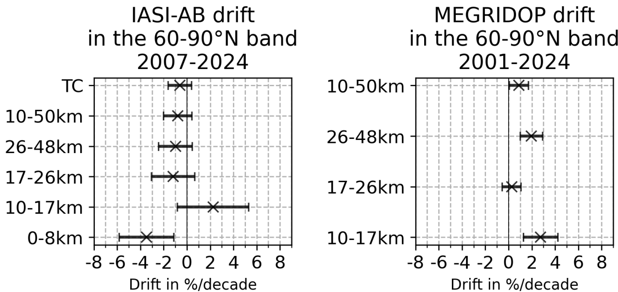
Figure 9. Drifts of satellites with respect to the zonal (weighted) means of all ground-based instruments in each column. Problematic ground-based instruments (Scoresbysund sonde, Resolute sonde before 2005) are not included in the means.
