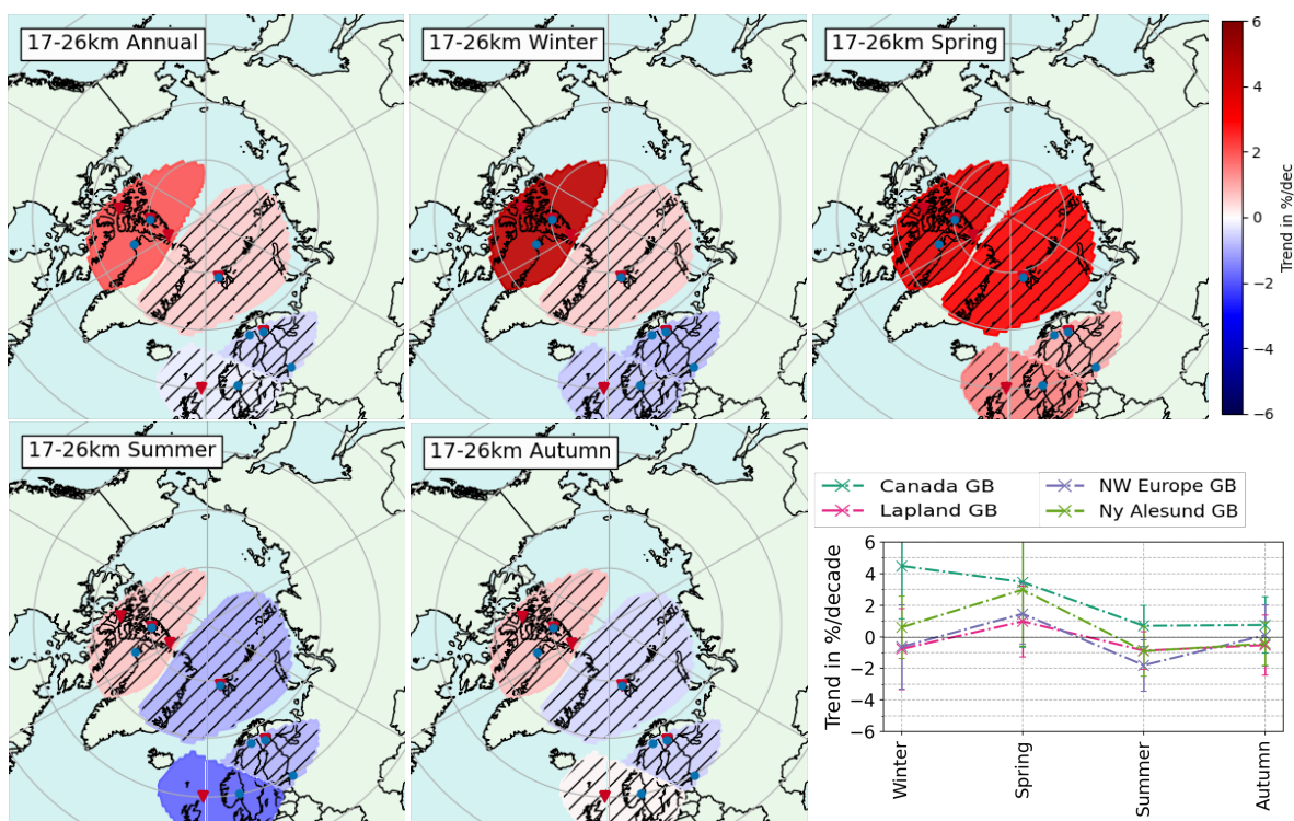
Figure 16. Same as Figure 14 for the mid-stratospheric column (17 – 26 km) ozone trends. Exact trend values and their 2\sigma uncertainties are displayed in the Appendix in Table D2.
