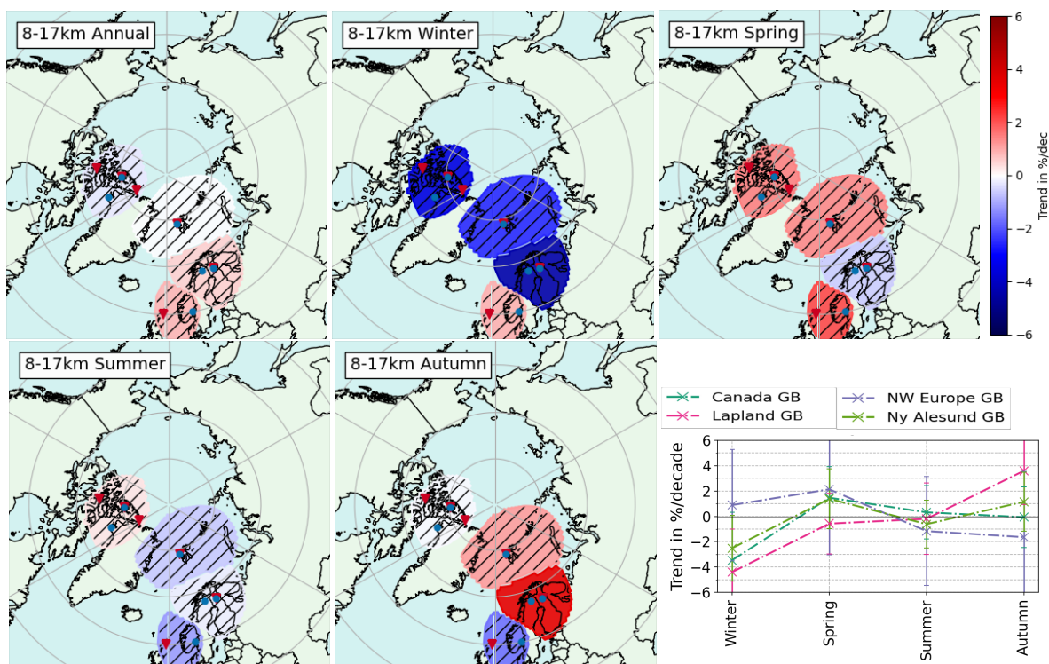
Figure 15. Same as Figure 14 for the lower stratospheric column (8 – 17 km) ozone trends. Exact trend values and their 2\sigma uncertainties are displayed in the Appendix in Table D2.
