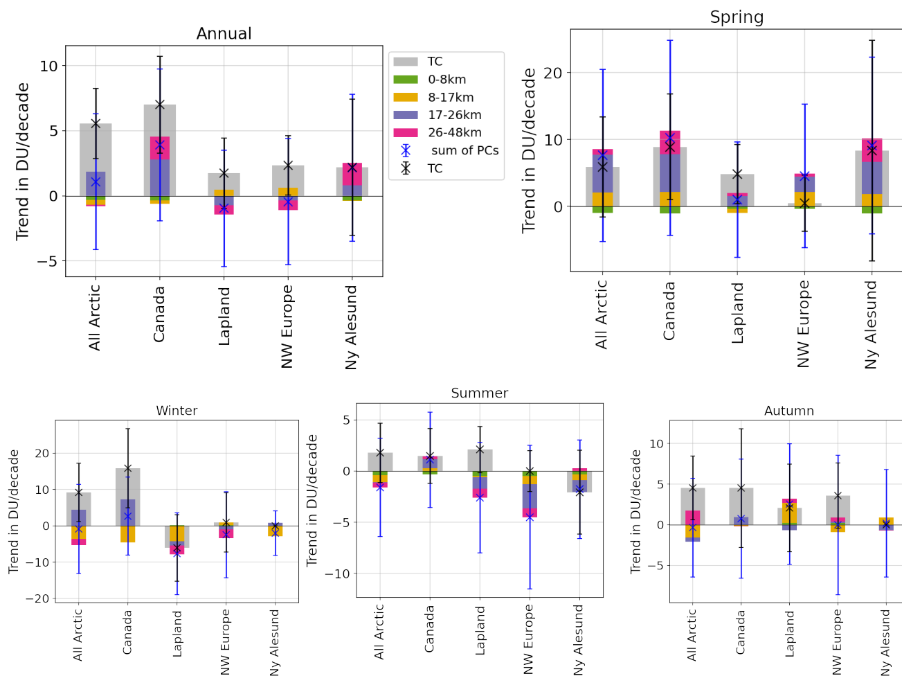
Figure 19. Sums of all partial columns trends compared to total column trends in DU per decade for annual and seasonal trends. The groups are not always the same across the different layers, therefore we calculate sums for the smallest represented regions, i.e., the regions of the lower stratosphere (8-17 km). As shown in Table 4, we have for instance: Canada (TC) = North Pole (0-8 km) + Canada (8-17 km) + Canada (17-26 km) + North Pole (26-48 km) and North Scandinavia (TC) = Scandinavia (0-8 km) + Lapland (8-17 km) + North-East Europe (17-26 km) + Scandinavia (26-48 km).
