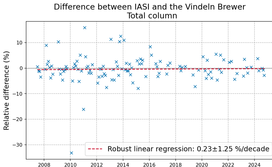
Figure 2. Difference of relative anomalies in percent \text{diff}_{\text{sat-GB}}^i (4) between the Vindeln Brewer total column and the IASI-CDR-IASI-A+B total column in Vindeln with associated bias, \text{MAD}_s . The trend of this difference is represented by the red dashed line and corresponds to the drift, given in legend with its 2\sigma -error. The presence of several strong outliers requires the use of a robust regression method, here the Theil-Sen method.
