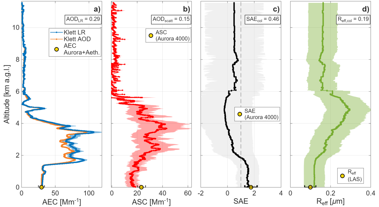
Figure 11. Results of the measurements on 29th August 2025, 15:20-16:30 UTC. Same variables as in Fig.8.
