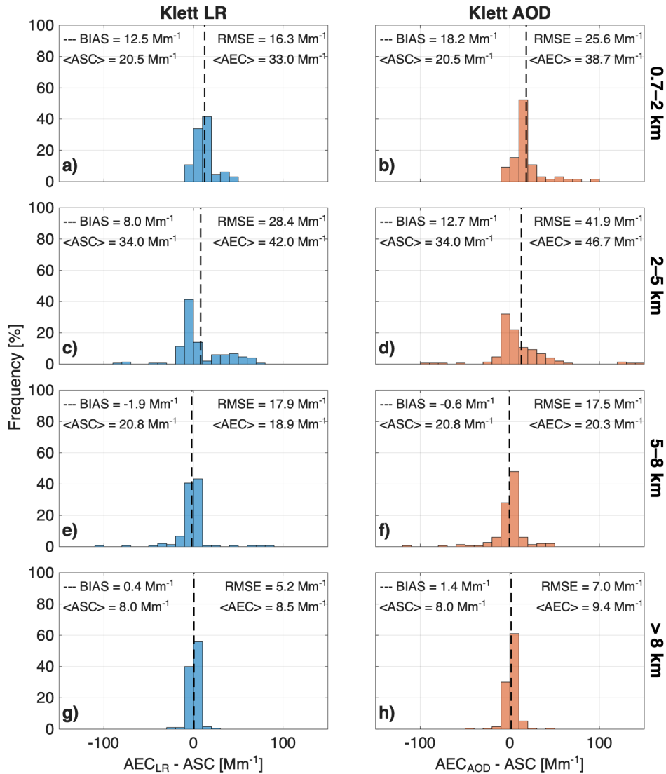
Figure 5. Frequency distributions of the difference between the aerosol extinction coefficient at 532 nm (AEC) retrieved from lidar and the aerosol scattering coefficient at 525 nm (ASC) measured by the AeroSonde, using all data collected during the measurement campaigns. Columns correspond to the two lidar retrievals (Klett LR, blue; Klett AOD, orange) and rows to four altitude ranges, as indicated on the right-hand side. The dashed vertical line marks the mean bias (BIAS). Each panel also gives the root-mean-square error (RMSE) and the layer-mean values of ASC and AEC.
