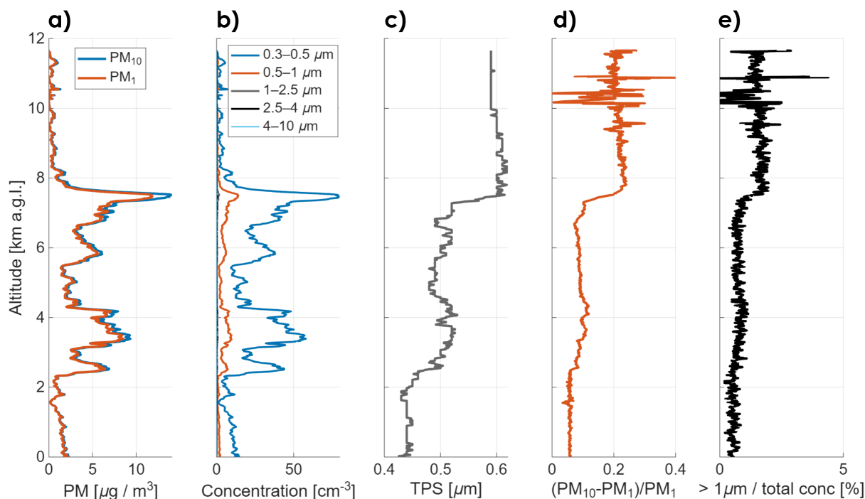
Figure 7. Vertical profiles of raw data obtained by AeroSonde during measurements on 7th August 2025, 15:20-16:30 UTC. Panel (a) shows mass concentrations of \text{PM}_{10} and \text{PM}_1 . Panel (b) presents particle number concentrations for selected size ranges (0.3-0.5, 0.5-1, 1-2.5, 2.5-4, and 4-10 \mu\text{m} ). Panel (c) shows the typical particles size parameter (TPS). Panel (d) displays the coarse-to-fine mass ratio expressed as (\text{PM}_{10} - \text{PM}_1)/\text{PM}_1 . Panel (e) presents the contribution of particles larger than 1 \mu\text{m} to the total number concentration.
