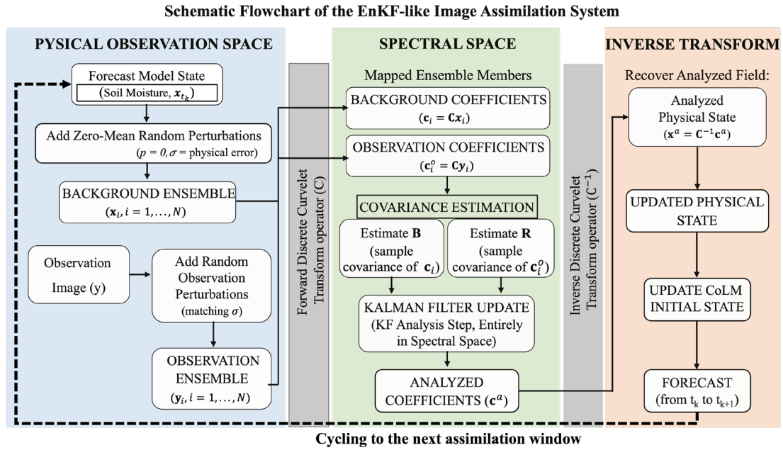
280 Figure 2: Schematic Flowchart of the EnKF-like Image Assimilation System.
