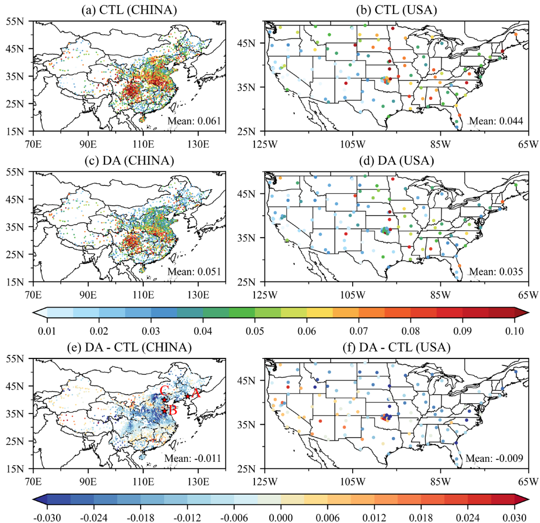
505 Figure 10: Spatial distribution of ubRMSE between 10 cm soil moisture from in-situ data and model simulations during the assimilation period. Figures (a) and (b) show results from the CTL experiment over the China and United States domains. Figures (c) and (d) show results from the image assimilation experiment over the same regions. Figures (e) and (f) present the differences between the image assimilation and CTL experiments. The average ubRMSE is provided in the lower-right corner of each panel. Red pentagons in Figure (e) indicate the locations of typical vegetation-type stations.
