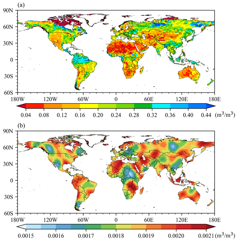
Figure 3: (a) Soil moisture background field and (b) difference between the background field and the reconstructed field after adding background error perturbations and applying first-mode curvelet inverse transformation.
