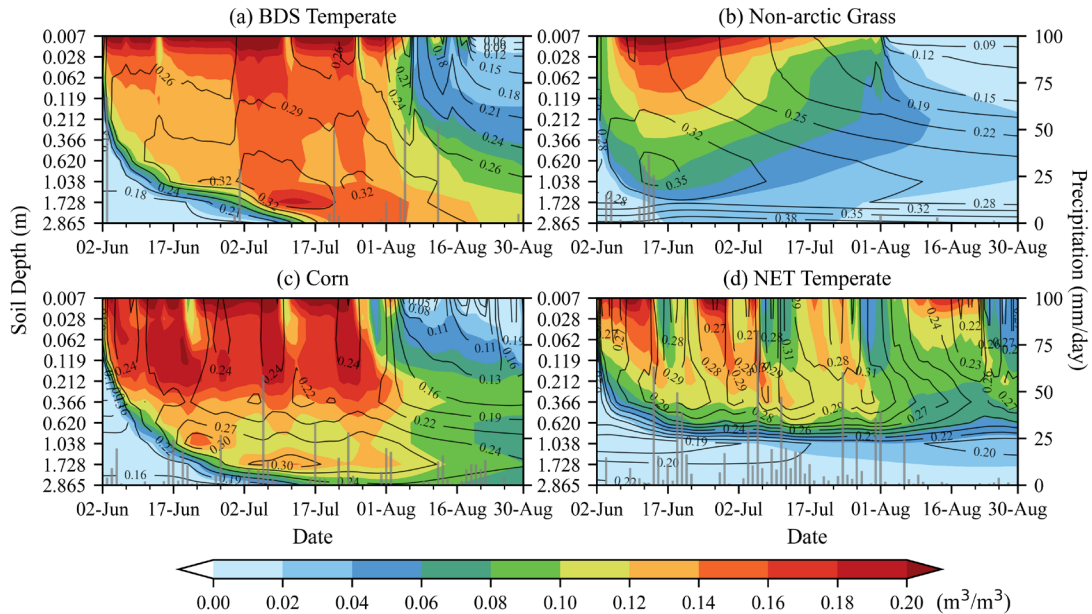
430 Figure 7: Temporal evolution of soil moisture differences between the image assimilation experiment and the CTL experiment (shading), along with the soil moisture profiles from the assimilation experiment (contours), for different vegetation types. Gray bars indicate precipitation. The locations correspond to the red pentagon markers in Figure 6f.
