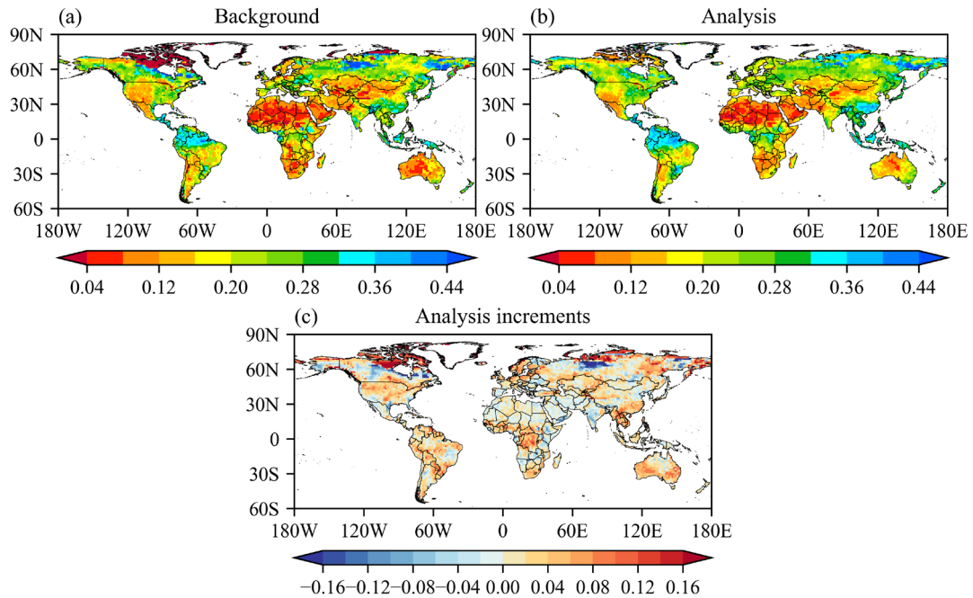
330 Figure 4: Spatial distribution of the instantaneous surface soil moisture at 0600 UTC on 2 June 2022. (a) Background field; (b) Analysis field; (c) Analysis increment.
