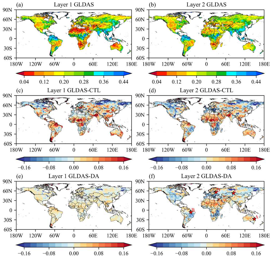
380 Figure 6: Spatial distribution of the instantaneous soil moisture at 0000 UTC on 1 August 2022. Figures (a) and (b) show the GLDAS reanalysis data for the 0–10 cm surface layer and the 10–40 cm subsurface layer. Figures (c) and (d) show the differences between GLDAS and the CTL experiment for the two layers. Figures (e) and (f) show the differences between GLDAS and the image assimilation experiment. The pentagons in figure (f) mark the locations of typical vegetation types selected for further analysis.
