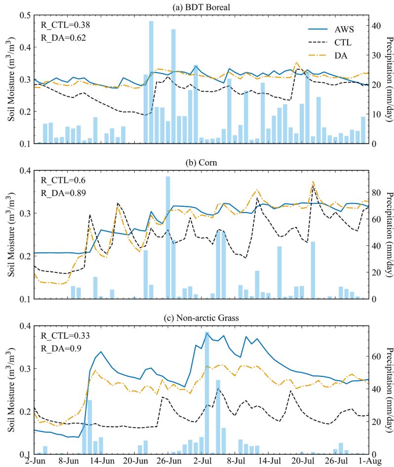
525 Figure 11: Time series of 10 cm soil moisture at representative in-situ stations during the assimilation period (June 2 to August 1, 2022). Station locations are indicated by red pentagons in Figure 10e. Black lines represent the CTL experiment, yellow lines indicate the image assimilation experiment, blue lines show in-situ observations at 10 cm depth, and blue bars represent precipitation. Correlation coefficients between each experiment and the in-situ observations are provided in the top-left corner of each panel.
