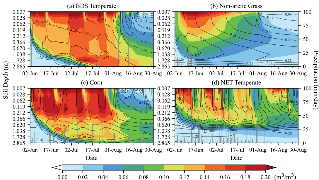
Figure 7: Temporal evolution of soil moisture differences between the image assimilation experiment and the CTL experiment (shading), along with the soil moisture profiles from the assimilation experiment (contours), for different vegetation types. Gray bars indicate precipitation. The locations correspond to the red pentagon markers in Figure 6f.
