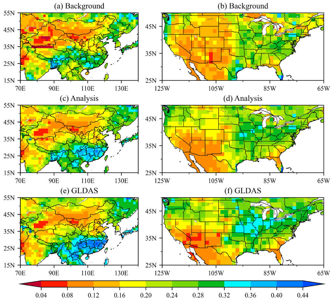
355 Figure 5: Spatial distribution of the instantaneous surface soil moisture over two typical terrain regions at 0600 UTC on 2 June 2022. Figures (a) and (b) show the background field, (c) and (d) show the analysis field, and (e) and (f) show the GLDAS reanalysis data.
