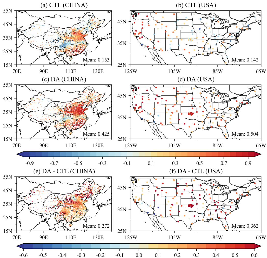
485 Figure 9: Spatial distribution of correlation coefficients between 10 cm soil moisture from in-situ data and model simulations during the assimilation period. Figures (a) and (b) show results from the CTL experiment over the China and United States domains. Figures (c) and (d) show results from the image assimilation experiment over the same regions. Figures (e) and (f) present the differences between the image assimilation and CTL experiments. The average correlation coefficient is provided in the lower-right corner of each panel.
