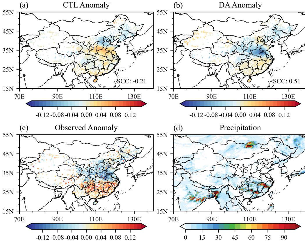
545 Figure 12: Spatial distribution of soil moisture anomalies on June 18, 2022, from (a) the CTL experiment, (b) the image assimilation experiment, and (c) in-situ observations. Figure (d) shows precipitation on the same date.
