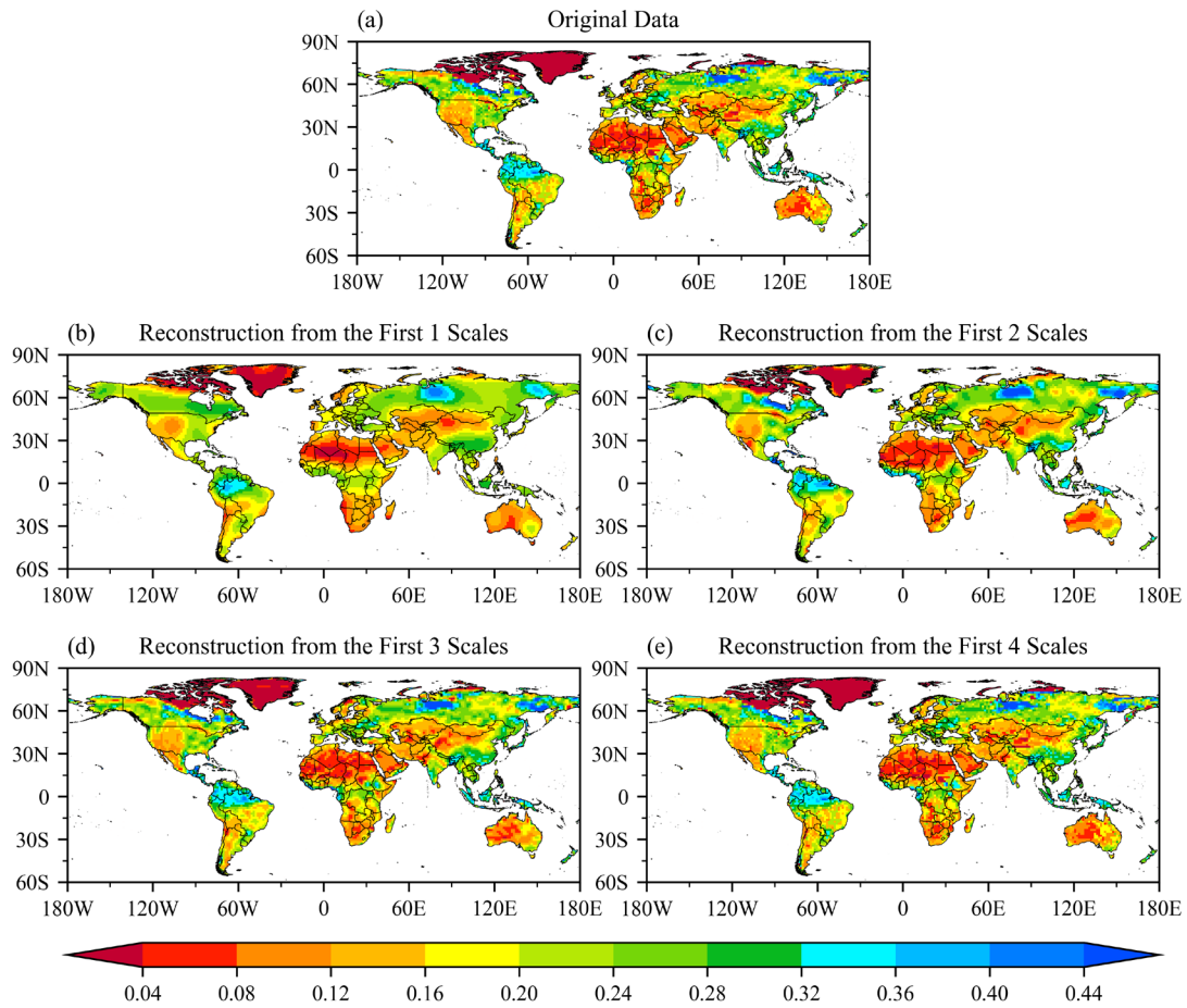
210 Figure 1: Spatial distribution of soil moisture from (a) the original image and reconstructed fields based on different curvelet coefficient modes: (b) the first mode, (c) the first two modes, (d) the first three modes, and (e) the first four modes on June 2, 2022.
