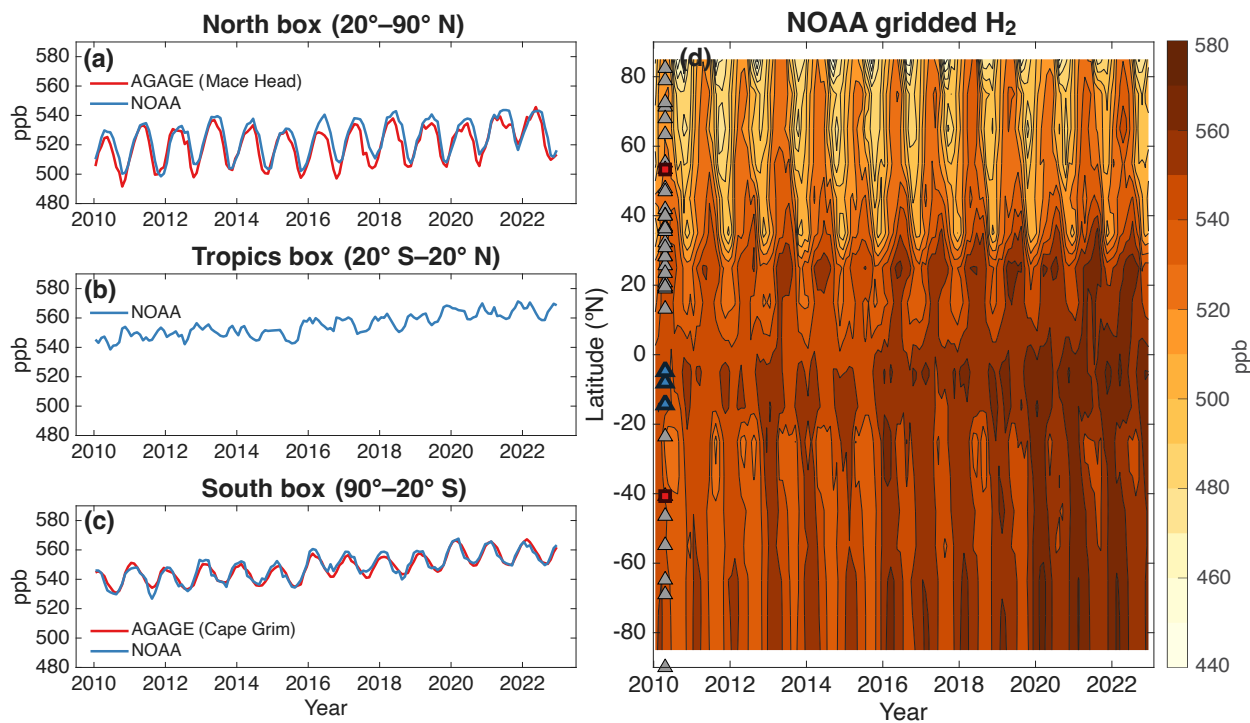
Figure S1. Comparison of (a) Mace Head and (c) Kennaook/Cape Grim H 2 data with North and South box NOAA flask data over 2010–2022. Average Tropics box NOAA data is shown in (b) based on stations at the blue triangles in (d). A linearly filled latitude-time NOAA dataset is shown in (d). Gray triangles show the latitudes of NOAA sites ( https://gml.noaa.gov/dv/site/?program=ccgg ). Red squares show the location of Mace Head and Cape Grim AGAGE sites.
