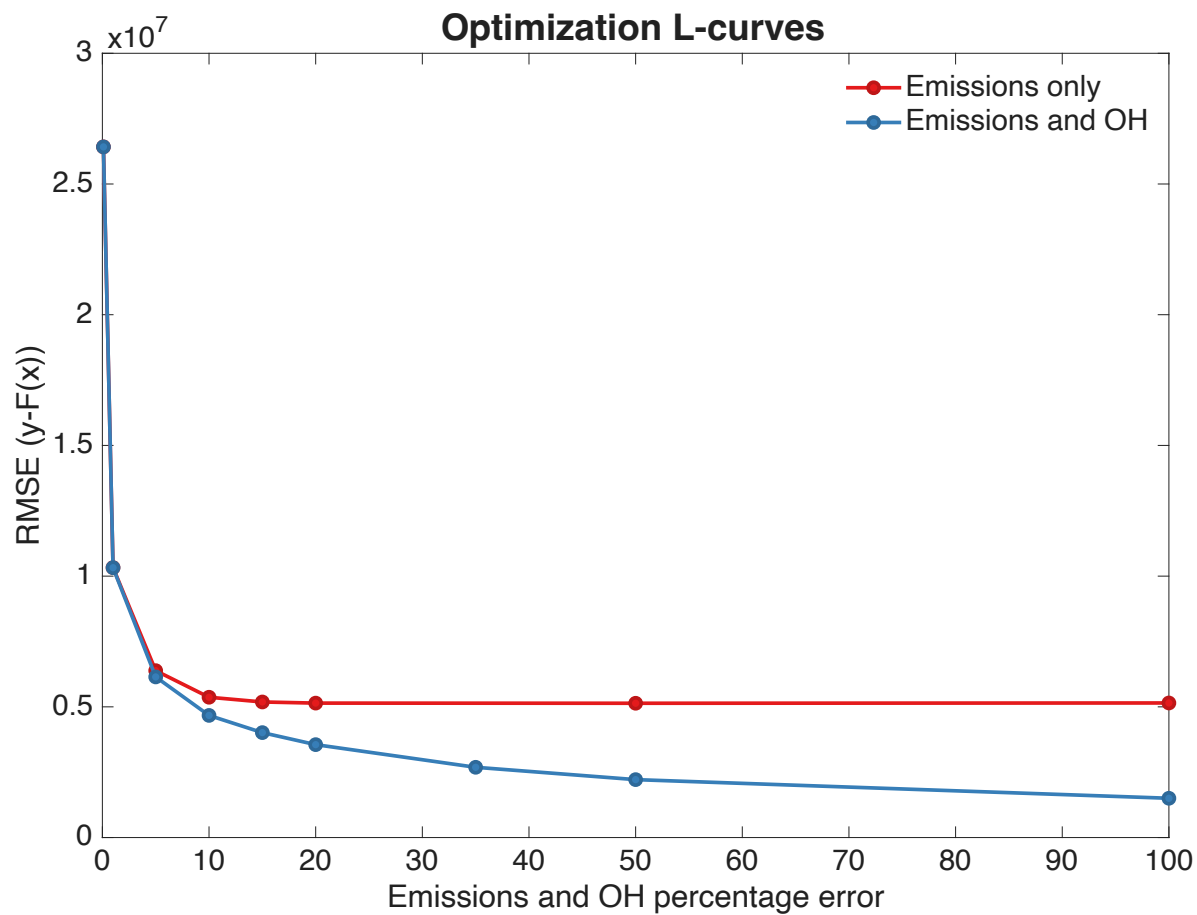
Figure S4. Optimization L-curves for the prior error covariance matrices of HFC-152a. For emissions only, OH error was set constant at .1%. For emissions and OH, both emissions and OH varied together.
