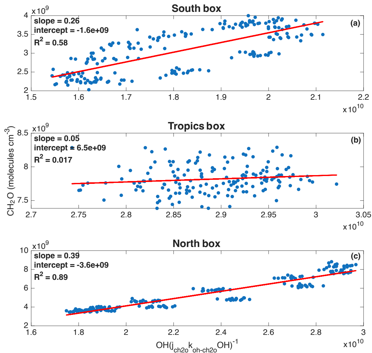
Figure S3. Model and TROPESS reanalysis derived slope and intercept terms for the (a) South box, (b) Tropics box, and (c) North box for the \text{CH}_2\text{O} derived from OH case following Eq. 1 in the main text.
