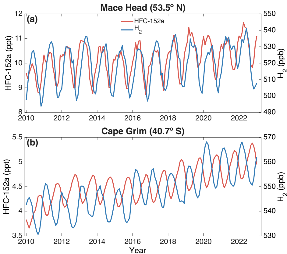
Figure 1. Comparison of HFC-152a and H 2 AGAGE times series at (a) Mace Head and (b) Cape Grim highlighting the different seasonal cycles and interhemispheric gradients.
