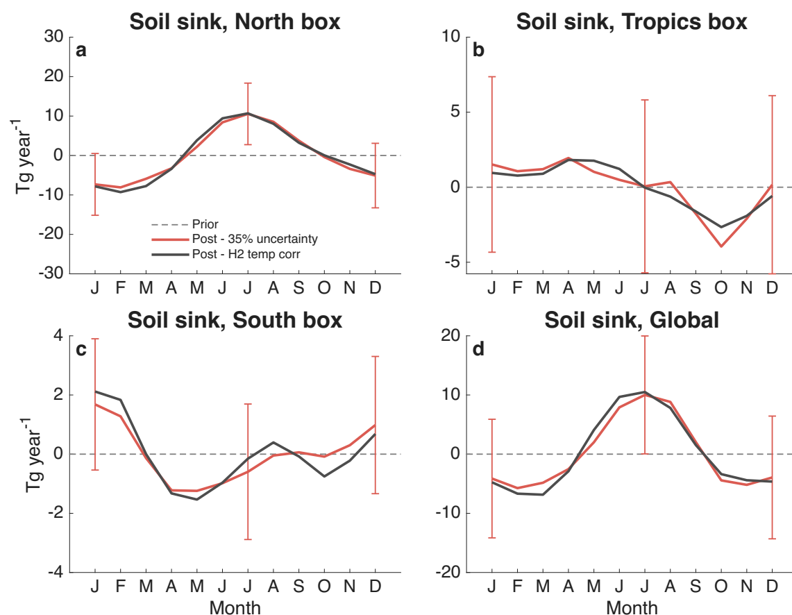
Figure R6. Comparison of no temporal correlation and a 6-month temporal correlation for the H_2 soil sink.
