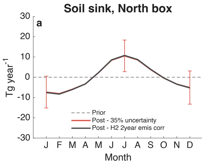
Figure R5. Results of doubling the correlation length for H 2 emissions for the North box
