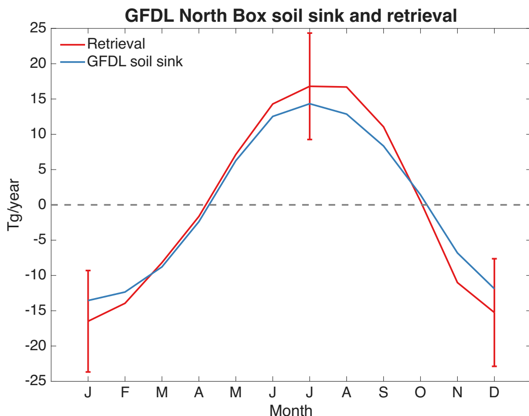
Figure R3. North box soil sink retrieved values compared to actual GFDL model values.
