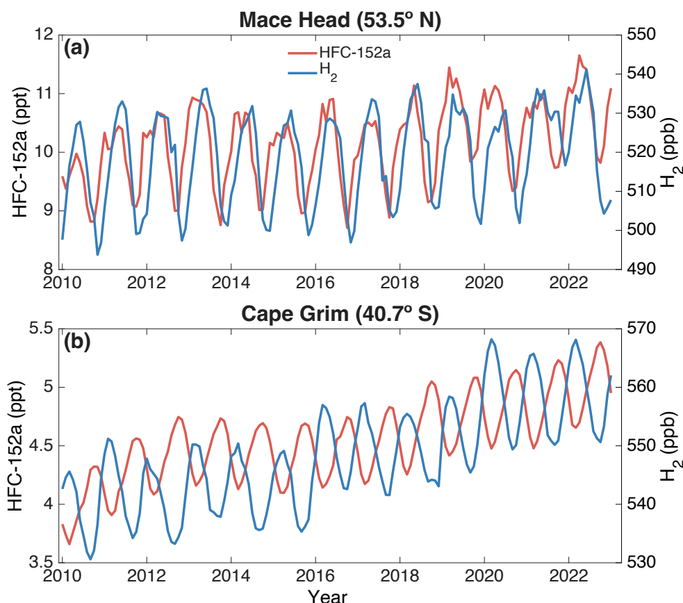
Figure R1. New Figure 1. Comparison of HFC-152a and H 2 AGAGE times series at (a) Mace Head and (b) Cape Grim highlighting the different seasonal cycles and hemispheric gradients.
