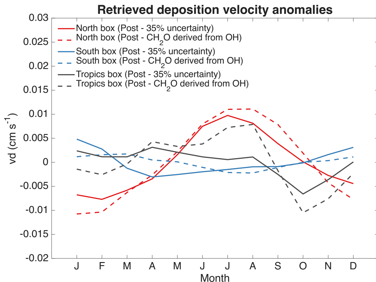
Figure R4. Estimated box average deposition velocity anomalies for two retrievals.
