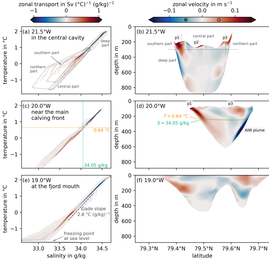
Figure 8. Overturning circulation in the 79NG fjord in temperature–salinity coordinates at three meridional transects: in the central cavity (a,b) and near the main calving front, inside (c,d) and outside (e,f) the cavity. The left column shows the zonal volume transport binned in temperature- and salinity-classes, the right column shows the corresponding zonal velocities in physical coordinates with positive velocities in the out-of-screen direction. The parts of the T – S diagram annotated in (a) correspond approximately to the areas marked in (b). The dividing salinity and temperature marked in (c) correspond to the isohaline and isotherm drawn in (d). The dotted line in (e) shows the freezing temperature at sea level pressure; note that lower temperatures can exist under the ice (e.g., in panel c) due to higher pressure. The labels p1–p3 mark the subglacial plumes annotated in Fig. 4.
