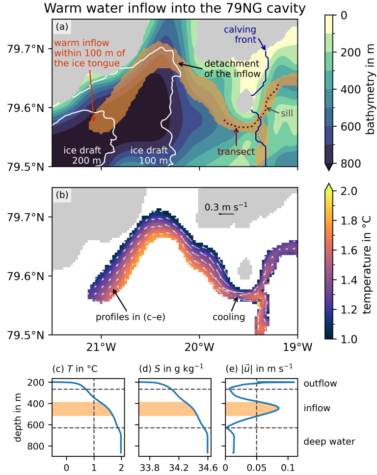
Figure 5. (a) Path of warm AIW flowing into the 79NG cavity (orange overlay) and (b) its vertically averaged velocity (little arrows) and temperature (color shading). (c–e) Vertical profiles of temperature, salinity and speed at the location marked in (b). Orange shadings in (c–e) highlight the part of the water column satisfying the criteria used in (a–b) with dashed vertical lines marking the thresholds at T = 1^{\circ}\text{C} in (c) and |\vec{u}| = 0.05 \text{ m s}^{-1} in (e). Dashed horizontal lines in (c–e) mark the velocity minima with water in the top layer flowing outward/eastward, including the melt water plume, in the middle layer flowing southwestward, and in the deep layer flowing northeastward with very low velocities. The dotted line in (a) marks the transect passing over the sill shown in Fig. 6.
