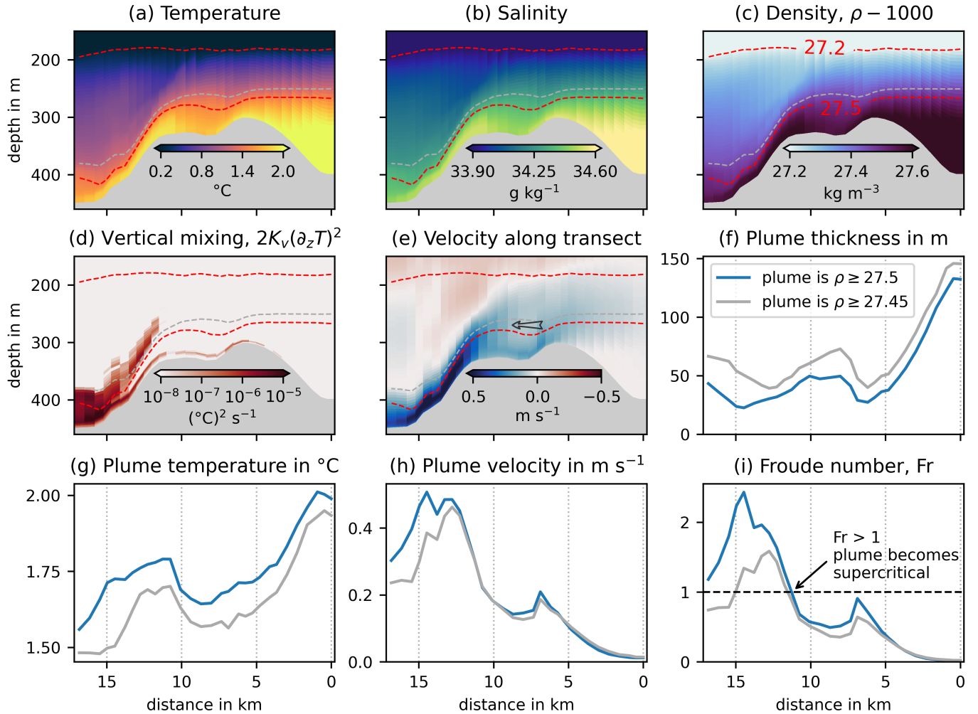
Figure 6. Properties of the inflow into the 79NG fjord along the transect marked in Fig. 5a. Panels (a–e) show vertical profiles of temperature (a), salinity (b), density anomaly (c), vertical turbulent mixing of temperature on a log scale (d), and flow velocity in the along-transect direction (e); red dashed lines mark the 27.2- and 27.5-isopycnals used to define the layers of ambient and plume water, see Sect. 2.4. Blue graphs in panels (f–i) show bulk properties of the plume: plume thickness (f), vertically averaged temperature (g), vertically averaged velocity (h), and Froude number (i). The sensitivity of the plume properties to the chosen plume interface is shown in gray, corresponding to the 27.45-isopycnal marked as gray dashed lines in panels (a–e). The x -axes of all panels show distance along the transect in the direction of the inflow, which is from right to left. Accordingly, positive velocities are also from right to left, as indicated by the arrow in (e). The sawtooth-like pattern visible in the first row is a visual artifact, because each grid cell is colored according to the value at the cell center, but model layers are tilted over sloping topography, resulting in visible differences between adjacent cells.
