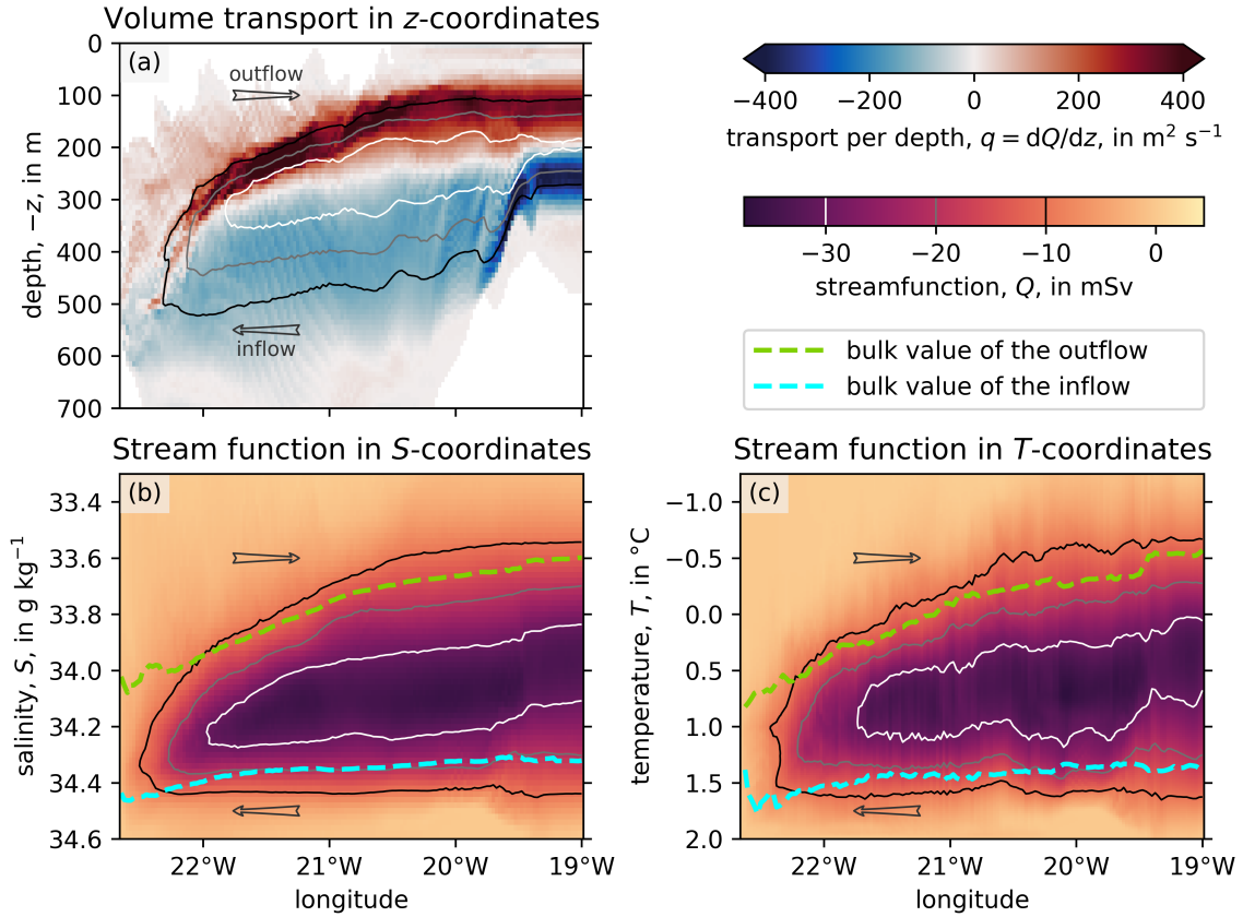
Figure 7. Zonal overturning circulation in the 79NG fjord in z -, S -, and T -coordinates. Panel (a) shows the volume transport per meter depth integrated across the fjord, with a westward propagating inflow (blue) below an eastward propagating outflow (red). Panels (b) and (c) show the overturning stream function with a vertical coordinate of salinity and temperature, respectively; dashed lines are the bulk salinities/temperatures of the in- and outflow. Note that the y-axes of all three panels increase downward to have the inflow below the outflow, as it is in reality. Thin contours in all panels mark the streamlines for Q = -10 \text{ mSv} , -20 \text{ mSv} , -30 \text{ mSv} .
