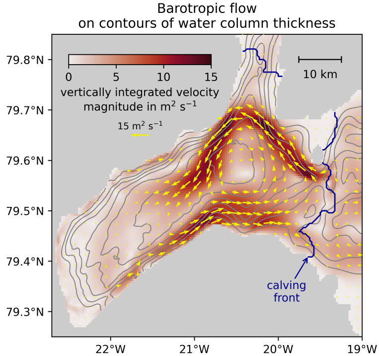
Figure 2. Intensity of the barotropic (i.e., vertically integrated) flow in the 79NG fjord shown in shades of red and the transport direction indicated by yellow arrows. Gray lines are the 100 m, 200 m, . . . , 700 m isolines of the water column thickness, i.e., the depth of the seafloor minus the ice draft; the outermost contour corresponds to 100 m, the closed contour near the center to 700 m.
