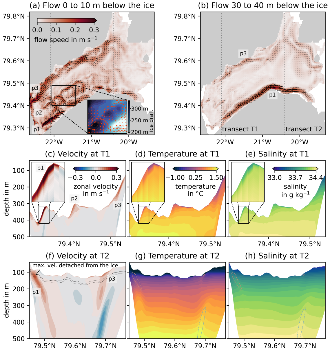
Figure 4. Details of the subglacial meltwater plumes below the 79NG ice tongue: the southern (p1), central (p2) and northern plume (p3). (a) Velocity of the flow averaged over the 10 m directly below the ice tongue; panel (b) is the same for the range of 30 m to 40 m below the ice. The inset in (a) shows how the flow turns around cone-like features in the ice topography; the area shown in the inset is about 13\text{ km} \times 10\text{ km} wide. For the transect T1 marked in (a) and (b), vertical profiles are shown in (c,d,e) for zonal velocity, temperature and salinity, respectively; panels (f–h) are analogous for transect T2. Zoomed insets in (c–e) show the fine vertical model resolution in the plume. Dotted lines in (f) mark the 30–40 m-range shown in (b). The \pm 0.1\text{ m s}^{-1} velocity contours are shown in (g) and (h) for orientation.
