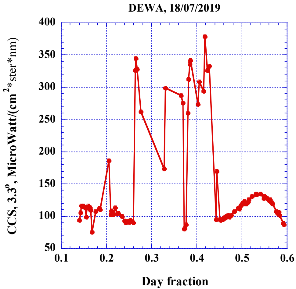
Figure 5. Temporal dependence of CCS (3.3) measured at DEWA AERONET site on July 18, 2019.
