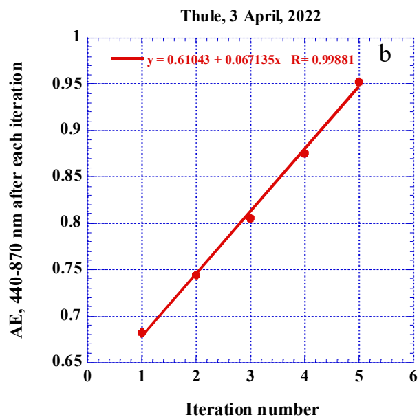
845 Figure 17. The dependence of net change in AE on the iteration number at a) Capo Verde AERONET site on April 2, 2022, b) 850 Thule AERONET site on April 3, 2022.
