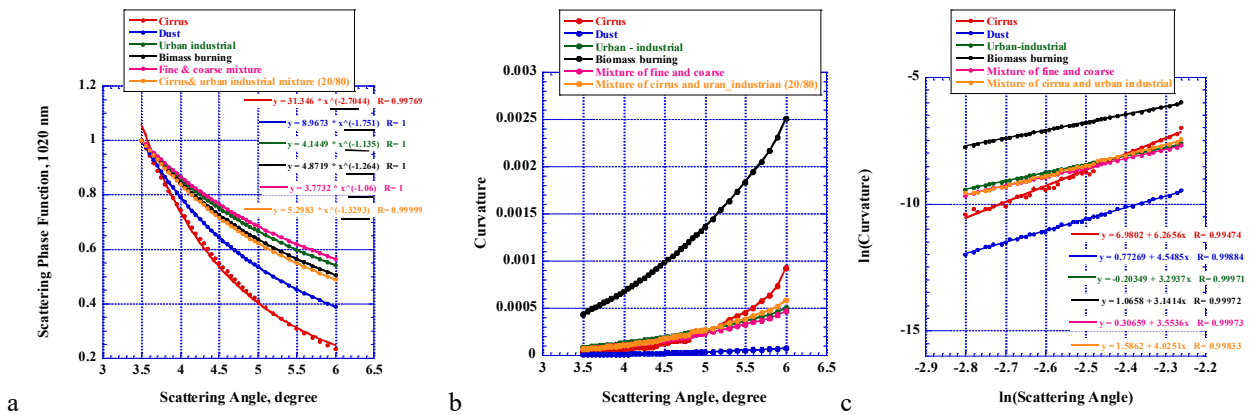
Figure 1. Scattering phase function calculated for different atmospheric particulates. Solid lines represent power law fit (a), Dependence of the curvature on the scattering angle in aureole calculated for three typical fine and coarse mode dominated aerosols, fine-coarse aerosols and aerosol-cirrus mixtures (b), Slope of the curvature in aureole estimated for three typical fine and coarse mode dominated aerosols, fine-coarse aerosols and aerosol-cirrus clouds mixtures (c).
