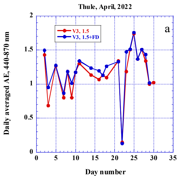
Figure 11. Daily averaged AE as function of day number for Thule AERONET site in April 2022. Red line corresponds to V3 level 1.5 and blue line after FD algorithm was applied: a) daily averaged AE, b) number of observations.
