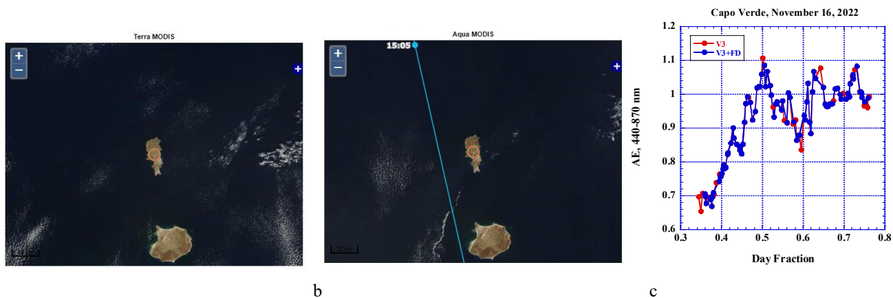
Figure 21. MODIS images of the area in vicinity of the Capo Verde AERONET site on November 16, 2022: Terra (a), Aqua (b), time series of AE, red and blue lines depict V3 and V3 after application of the FD algorithm respectively. On the Aqua image, blue line shows the Aqua MODIS satellite track.
