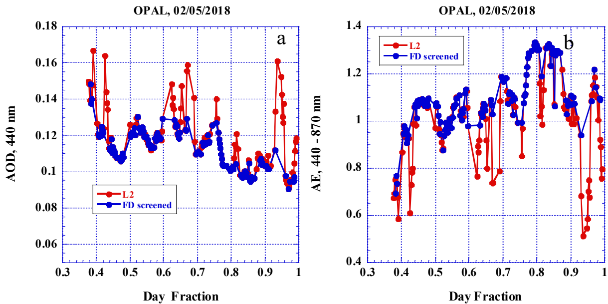
Figure 9. Results of applying of FD algorithm at OPAL AERONET site on May 2, 2018: a)AOD, b) AE (440-870).
