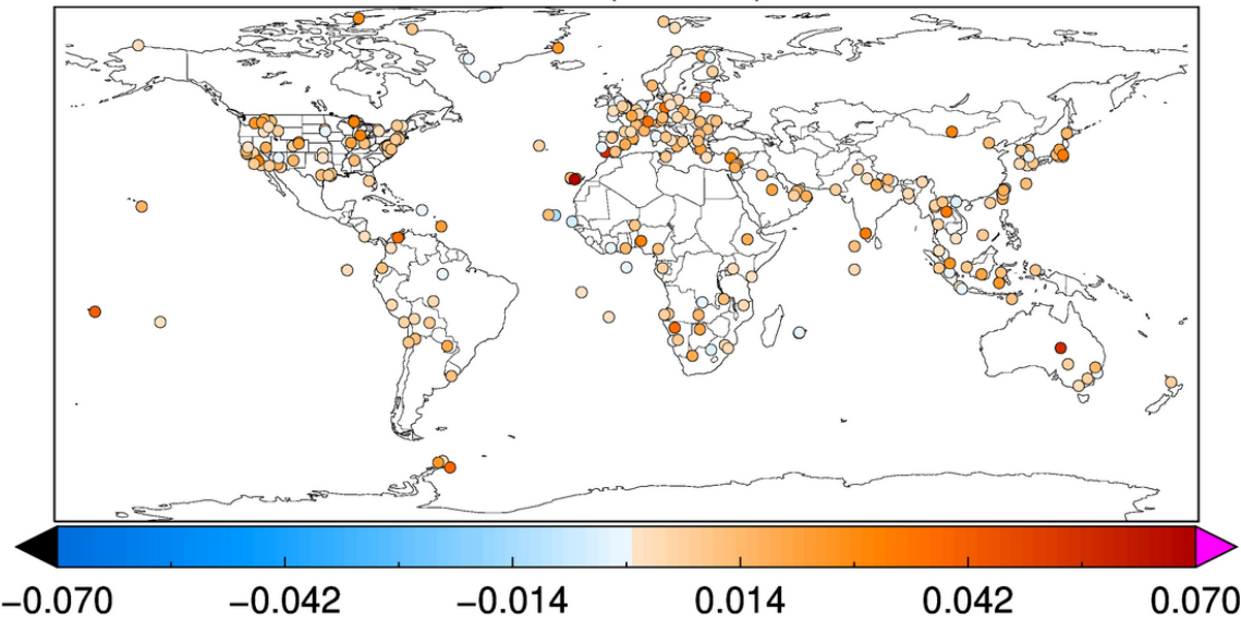
Figure 26. Percentage changes in AOD a) and AE b) due to the FD algorithm application. Positive: increased after applying the FD test, negative: decrease after applying the FD test.
