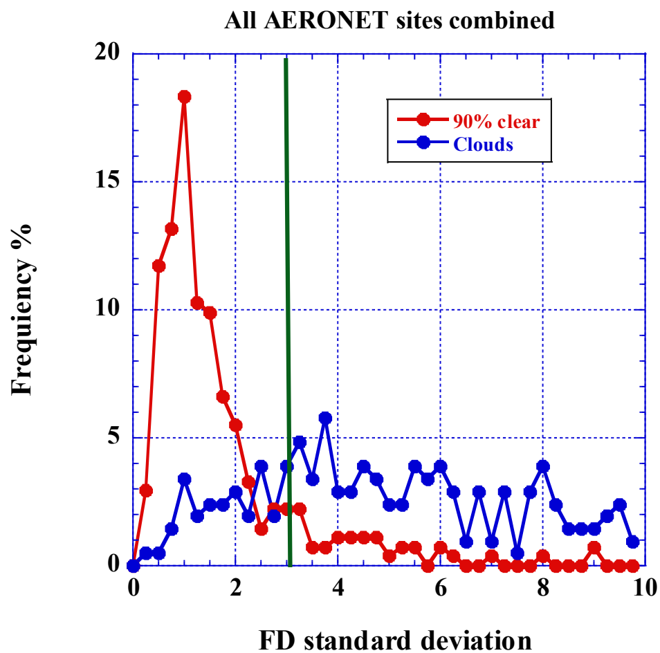
950 Figure 22. Distribution of FD standard deviation for 90% clear (red line) and cloudy (blue line) conditions. Vertical line shows 955 selected value for the threshold.
