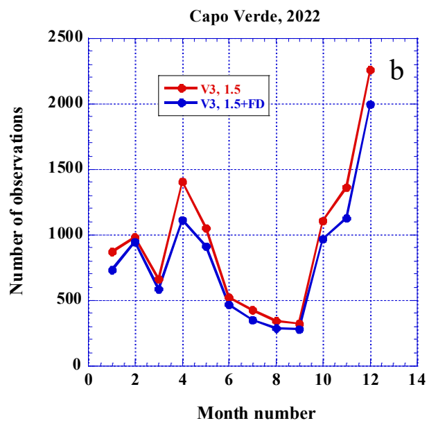
Figure 13. Monthly averaged AE as function of month for Capo Verde AERONET site. Red line corresponds to V3 level 1.5 and blue line after FD algorithm was applied: a) monthly averaged AE(440-870), b) number of observations
