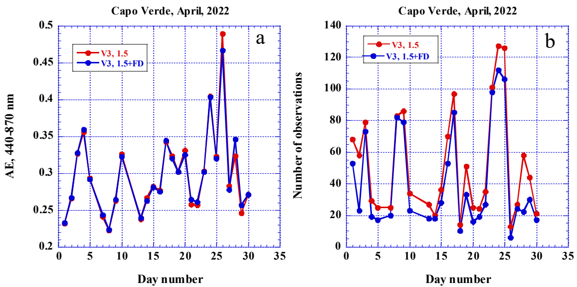
785 Figure 14. Daily averaged AE as function of day number for Capo Verde AERONET site in April 2022. Red line corresponds 790 to V3 level 1.5 and blue line after FD algorithm was applied: a) daily AE(440-870), b) number of observations.
