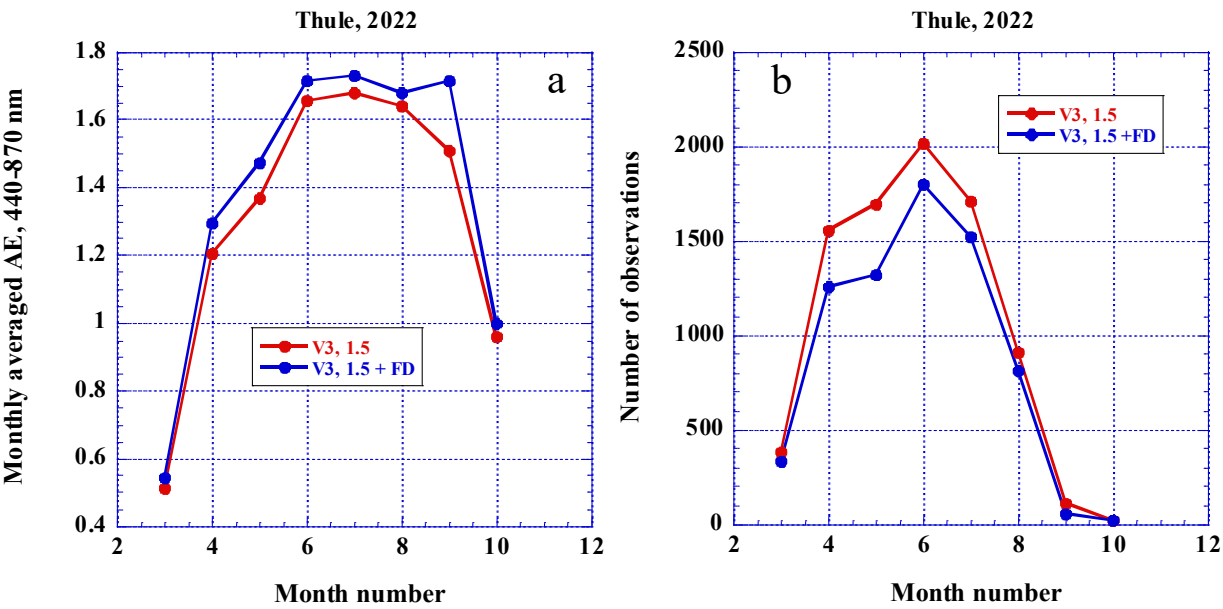
Figure 10. Monthly averaged AE as function of month for Thule AERONET site. Red line corresponds to V3 level 1.5 and 745 blue line after FD algorithm was applied; a) monthly averaged AE, b) number of observations
