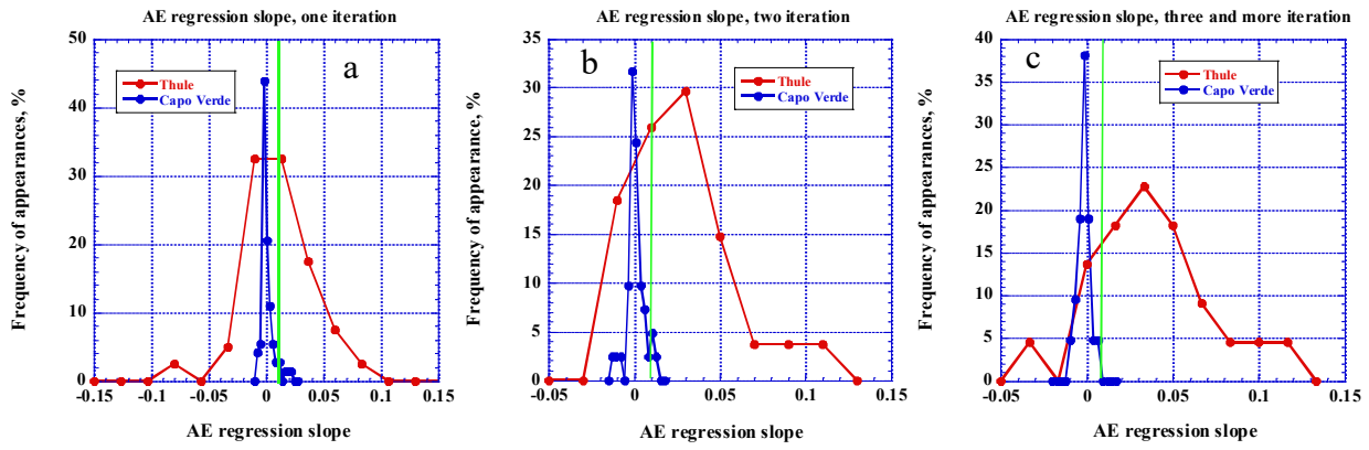
Figure 18. The histograms of AE regression slope after one FD iteration for Thule (red line) and Capo Verde (blue line) for the entire year of 2022: a) after one iteration, b) after two iterations, c) after three and more iterations.
