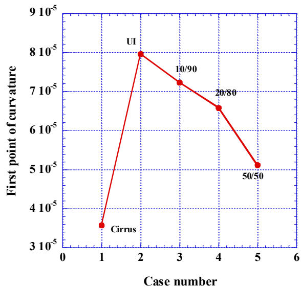
Figure 2. Dependence of the curvature slope on the cloud fraction for the three mixtures of urban industrial aerosol with cirrus clouds, (cirrus clouds/aerosols): 10/90, 20/80, and 50/50 (a), dependence of the first point of the curvature on case number, each case corresponding to the different cloud fraction for the mixture of urban-industrial aerosols with cirrus clouds (b)
