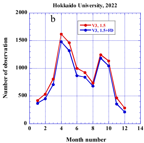
Figure 12. Monthly averaged AE as function of month for Hokkaido University AERONET site. Red line corresponds to V3 level 1.5 and blue line after FD algorithm was applied: a) monthly averaged AE (440-870), b) number of observations.
