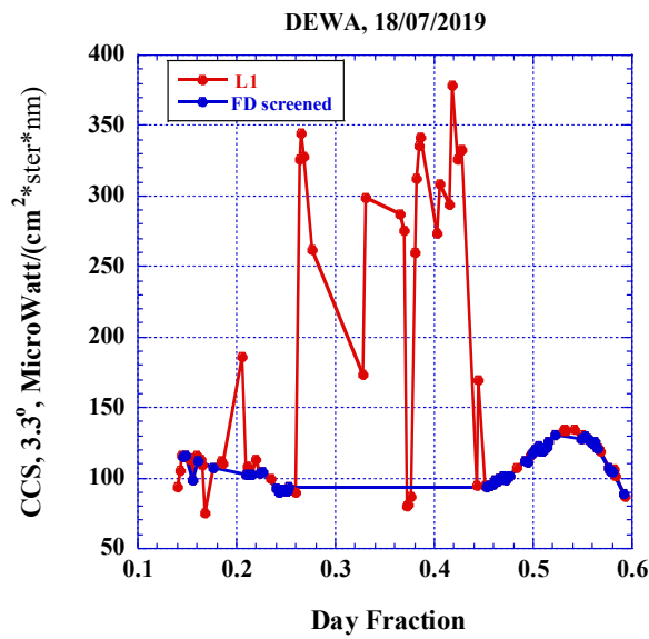
Figure 8. Temporal dependence of CCS (3.3) measured at Kuopio AERONET site on May 2 (a) and at DEWA AERONET site on July 18, 2019 (b)
