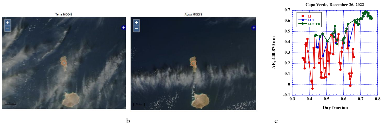
Figure 20. Terra MODIS image of the area in vicinity of the Capo Verde AERONET site on December 26, 2022: Terra (a), Aqua (b), time series of A, red, blue and green lines depict L1, L1.5 and L1.5 after application of the FD algorithm respectively.
