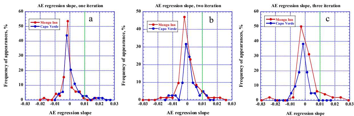
880 Figure 19. The histograms of AE regression slope after one FD iteration for Mongu Inn (red line) and Capo Verde (blue line) 885 for the entire year of 2022: a) after one iteration, b) after two iterations, c) after three iterations.
