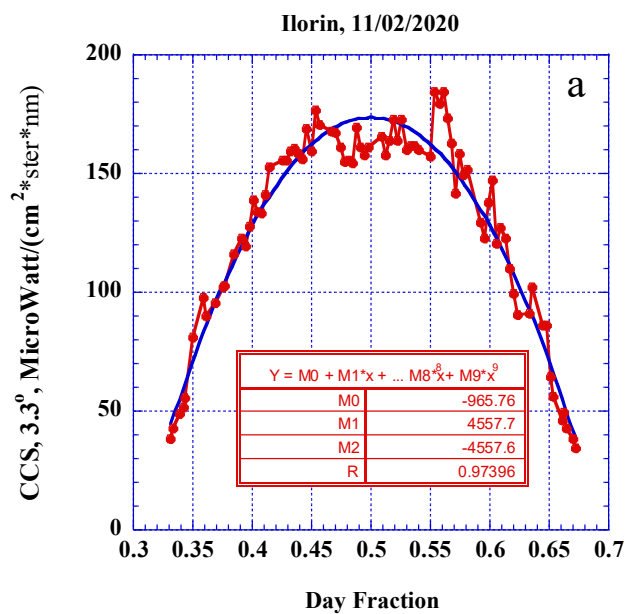
Figure 4. Temporal dependence of CCS (3.3) measured at a) Ilorin AERONET site on February 11, 2020, b) DEWA AERONET site on July 4, 2019
