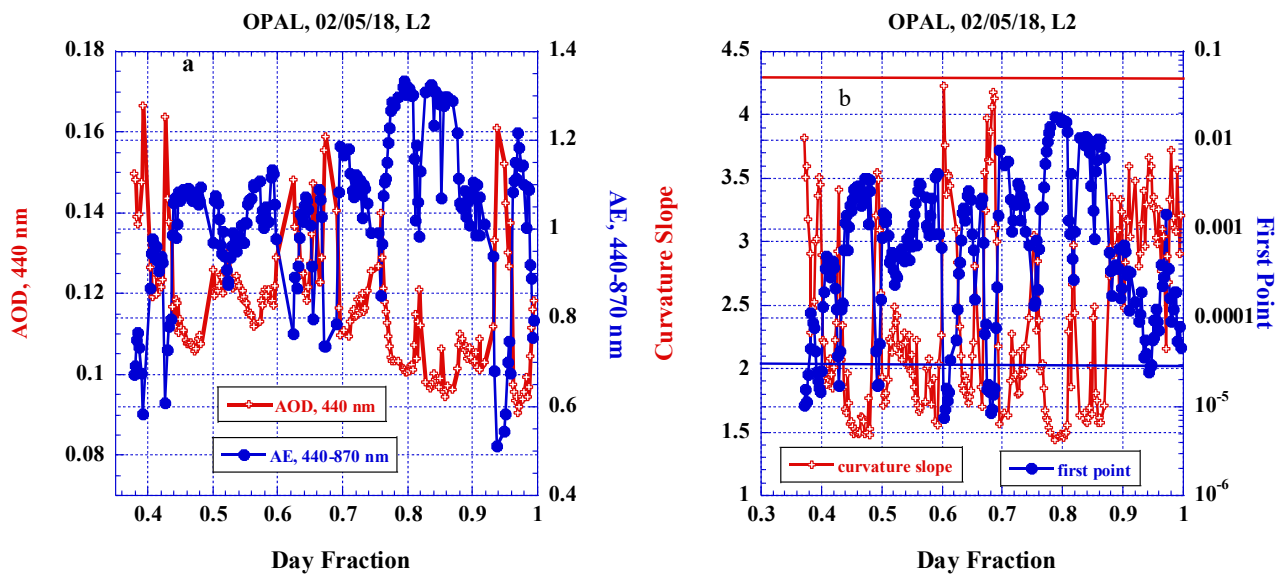
Figure 3. Temporal dependence of level 2 AOD measured at OPAL AERONET site on May 2, 201 (a), slope of the curvature 635 and the first point of curvature calculated from CCS (3.3) measurements (b).
