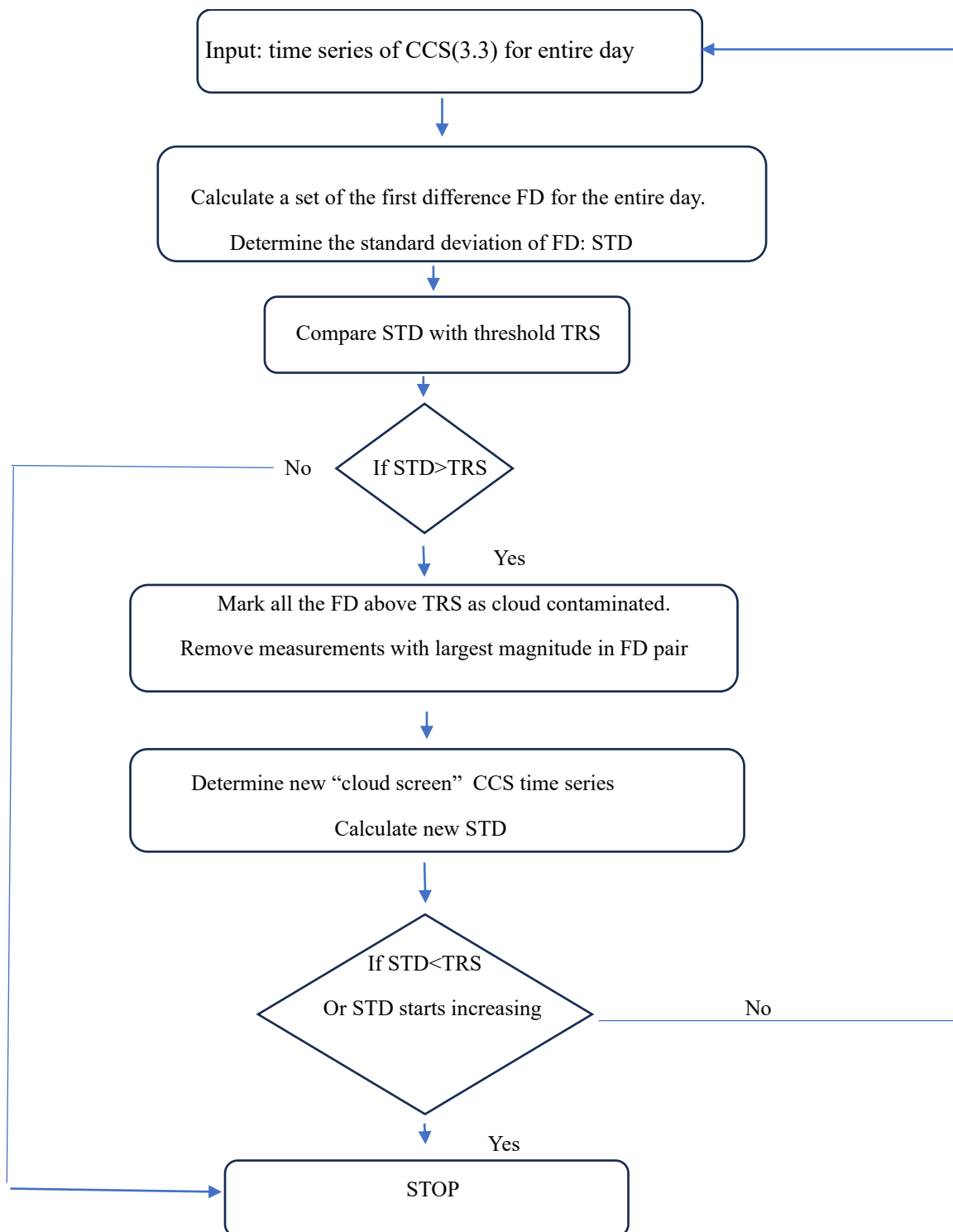
Figure 6. Flow chart of FD algorithm.
