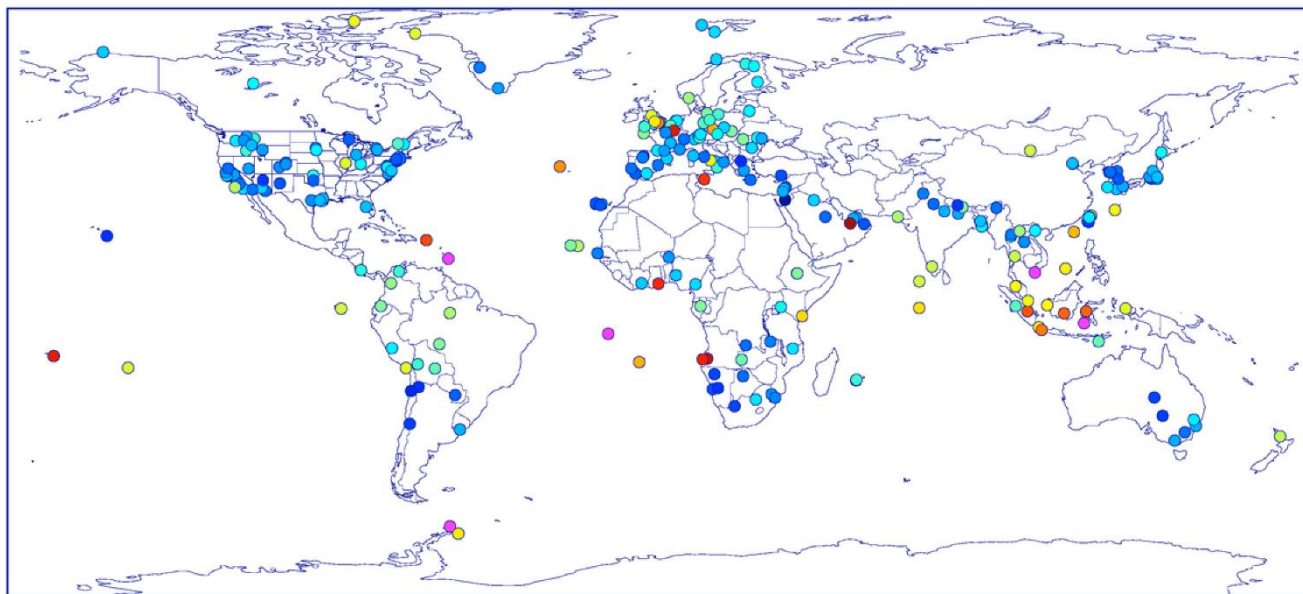
Figure 25. The percentage of data points which did not pass the FD test from V3 L1.5.
