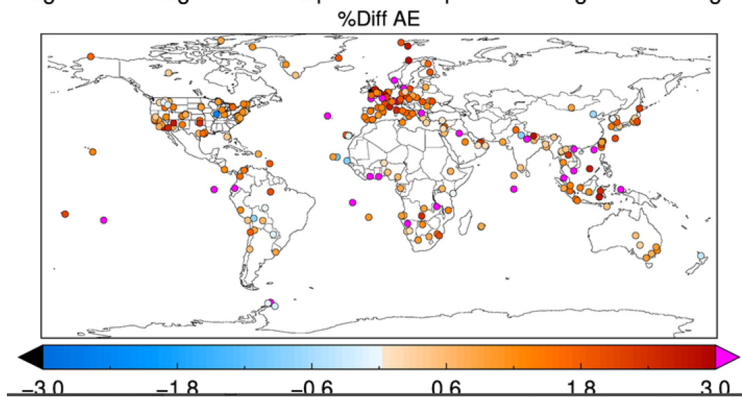
1015 Figure 26. Percentage changes in AOD a) and AE b) due to the FD algorithm application. Positive: increased after applying the FD test, negative: decrease after applying the FD test.
