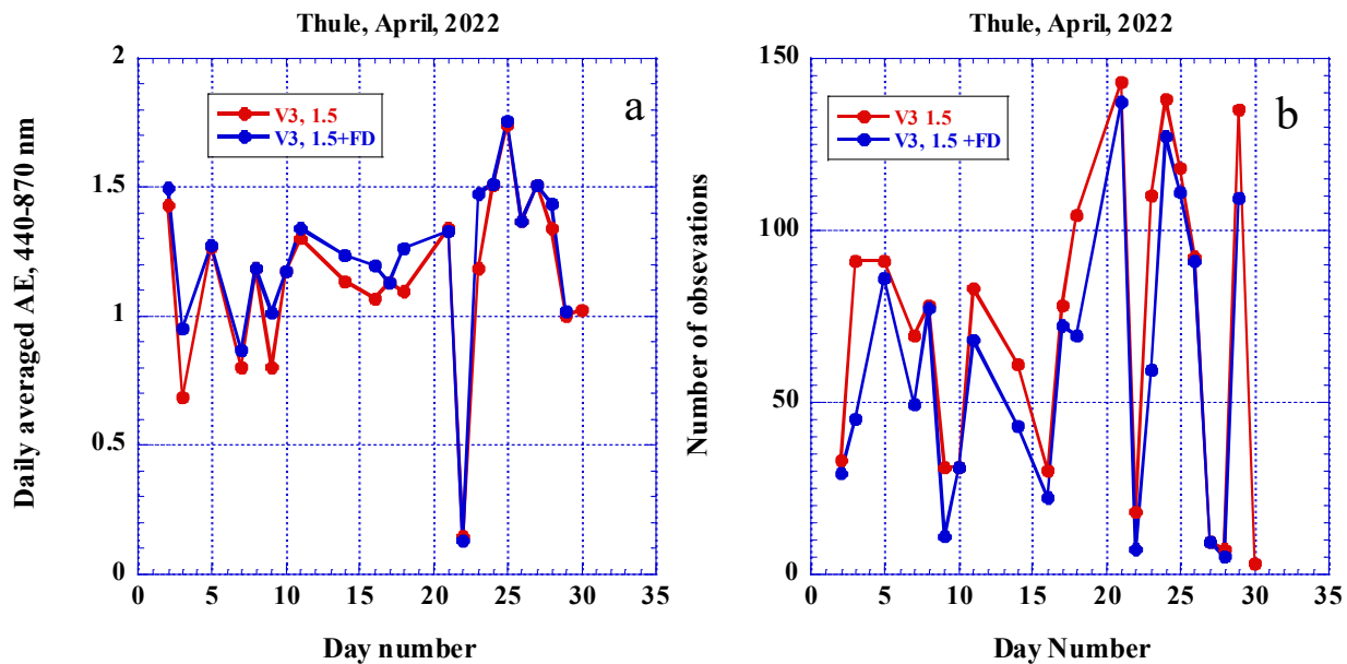
Figure 11. Daily averaged AE as function of day number for Thule AERONET site in April 2022. Red line corresponds to V3 level 1.5 and blue line after FD algorithm was applied: a) daily averaged AE, b) number of observations.
