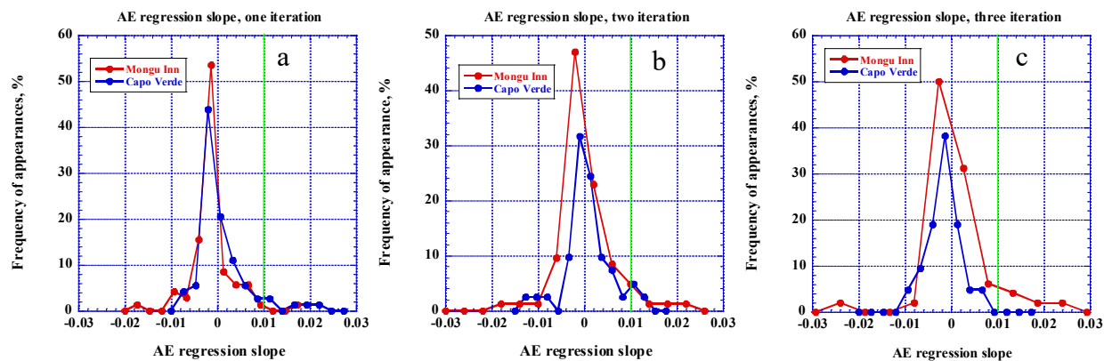
Figure 19. The histograms of AE regression slope after one FD iteration for Mongu Inn (red line) and Capo Verde (blue line) for the entire year of 2022: a) after one iteration, b) after two iterations, c) after three iterations.
