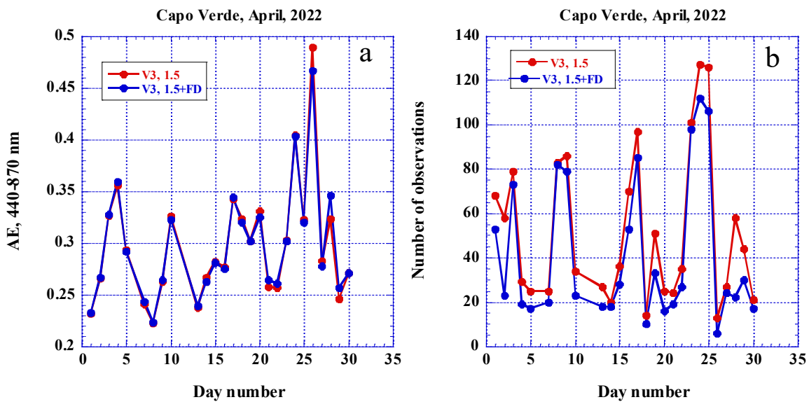
Figure 14. Daily averaged AE as function of day number for Capo Verde AERONET site in April 2022. Red line corresponds to V3 level 1.5 and blue line after FD algorithm was applied: a) daily AE(440-870), b) number of observations.
