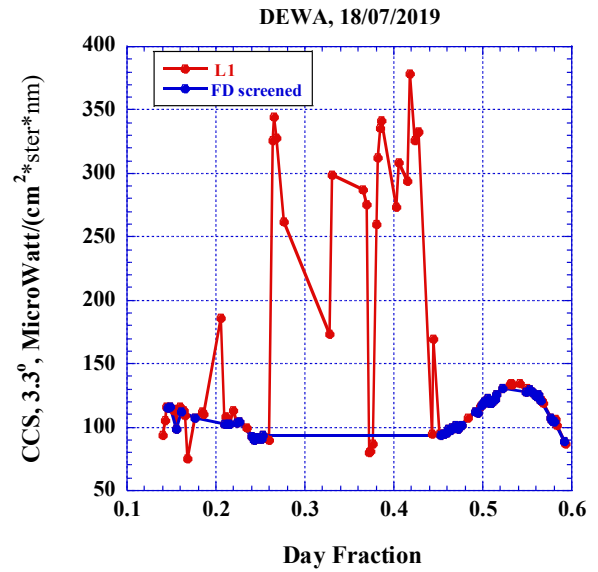
Figure 8. Temporal dependence of CCS (3.3) measured at Kuopio AERONET site on May 2 (a) and at DEWA AERONET site on July 18, 2019 (b)
