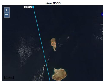
Figure 21. MODIS images of the area in vicinity of the Capo Verde AERONET site on November 16, 2022: Terra (a), Aqua (b), time series of AE, red and blue lines depict V3 and V3 after application of the FD algorithm respectively.
