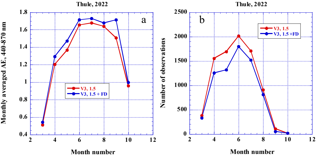
Figure 10. Monthly averaged AE as function of month for Thule AERONET site. Red line corresponds to V3 level 1.5 and blue line after FD algorithm was applied; a) monthly averaged AE, b) number of observations
