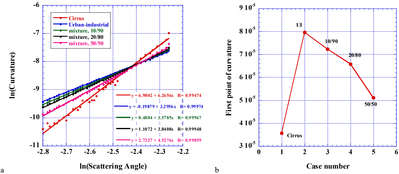
Figure 2. Dependence of the curvature slope on the cloud fraction for the three mixtures of urban industrial aerosol with cirrus clouds, (cirrus clouds/aerosols): 10/90, 20/80, and 50/50 (a), dependence of the first point of the curvature on cloud fraction for the mixture of urban-industrial aerosols with cirrus clouds (b)
