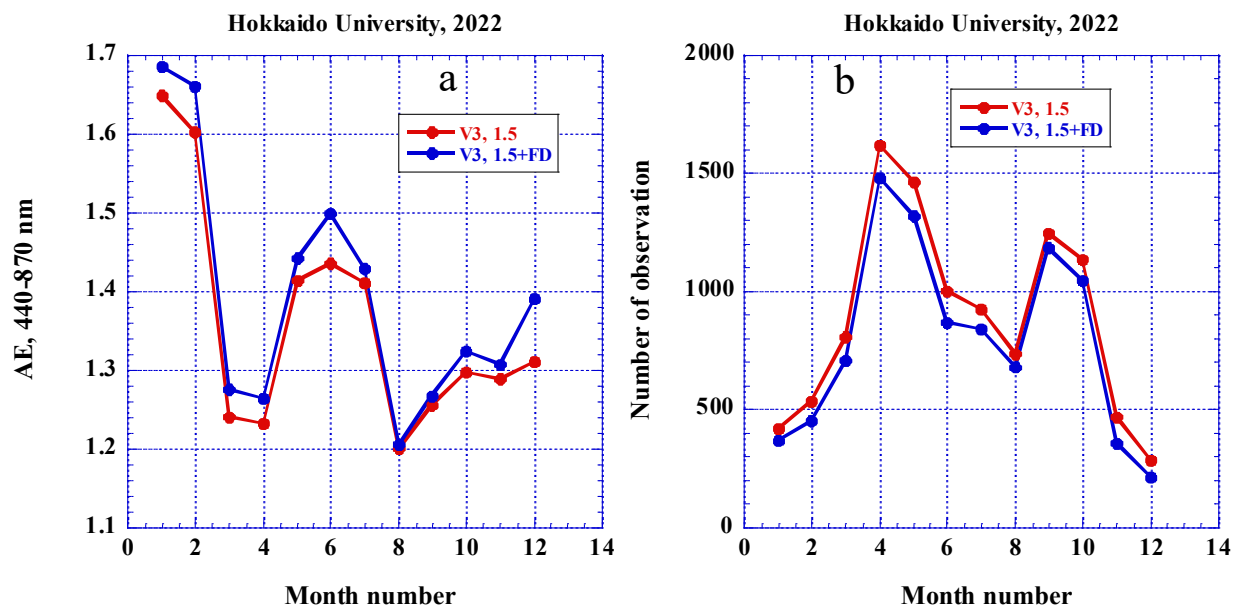
Figure 12. Monthly averaged AE as function of month for Hokkaido University AERONET site. Red line corresponds to V3 level 1.5 and blue line after FD algorithm was applied: a) monthly averaged AE (440-870), b) number of observations.
