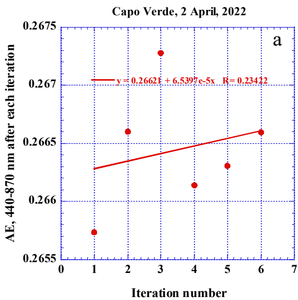
Figure 17. The dependence of net change in AE on the iteration number at a) Capo Verde AERONET site on April 2, 2022, b) Thule AERONET site on April 3, 2022.
