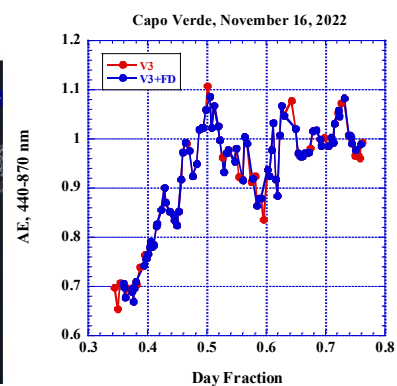
Figure 21. MODIS images of the area in vicinity of the Capo Verde AERONET site on November 16, 2022: Terra (a), Aqua (b), time series of AE, red and blue lines depict V3 and V3 after application of the FD algorithm respectively.
