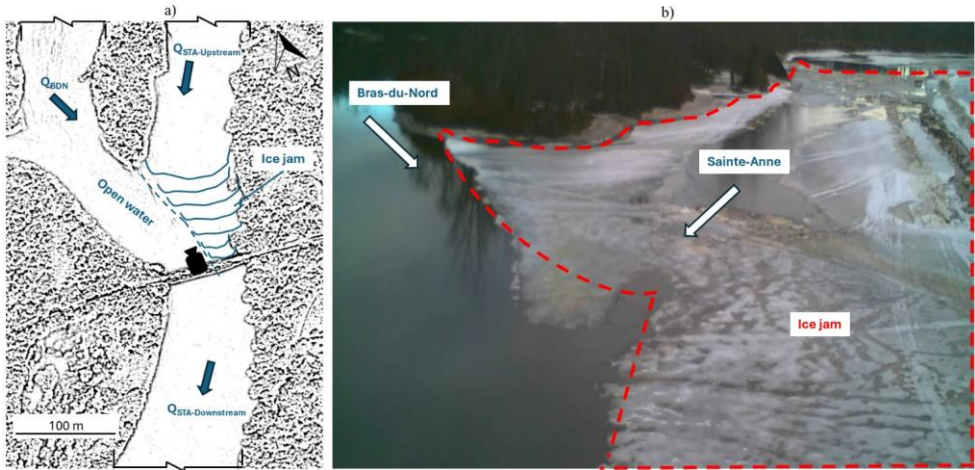
Figure 8: Jamming due to flow impact with a) a schematic representation and b) a picture taken at site BDN0-STA3 on April 7, 2021, looking upstream towards the flow as represented by the camera symbol in a), where the ice jam appeared at STA-BDN. The red dotted line in b) represents the ice jam caused by the effect of flow impact from the BDN on the ice in STA.
