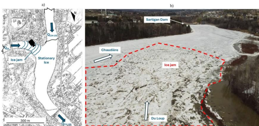
Figure Figure 108: Jamming due to stationary ice with a) a visual representation and b) a drone picture taken at site DL0-CH104 on March 31, 2022, looking downstream in the flow direction as represented by the camera symbol in a) where the ice jam appeared at CH-DL.
