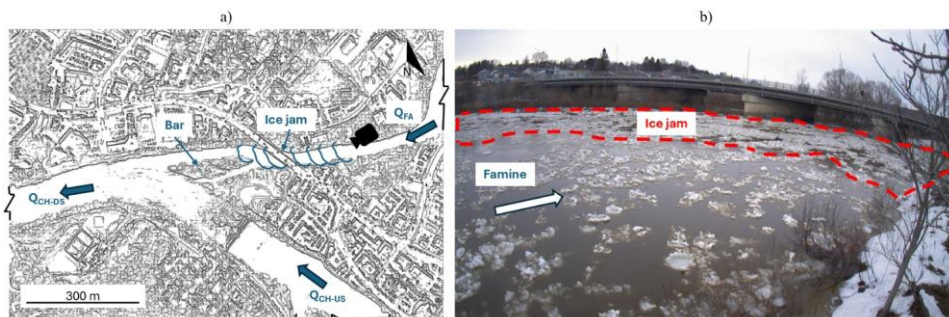
Figure 119: Jamming on depositional fan with a) a visual representation and b) a picture taken at site FA02 on April 11, 2023, looking downstream in the flow direction of FA as represented by the camera symbol in a), where the ice jam appeared at the mouth of the FA.
