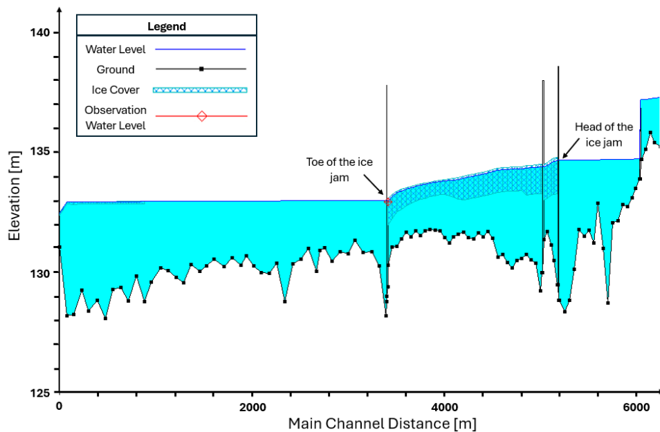
Figure 9: Profile of calibrated ice jam of April 7, 2021, on the STA River confluence.
