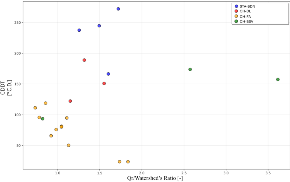
Figure 13: Relationship between discharge ratio (Qr) divided by the Watershed's Ratio (from Table 1) and cumulative degree-days of thawing (CDDT) on the ice jam day at the confluence site over the study period for all four confluences studied.
