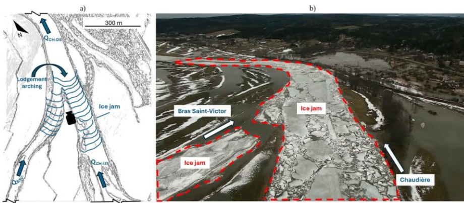
Figure 12: Jamming of arching ice pieces with a) a visual representation and b) a drone picture taken at site BSV0-CH75 on March 6, 2024, looking downstream in the flow direction as represented by the camera symbol in a), where the ice jam occurred at CH-BSV.
