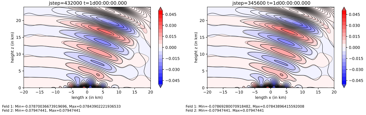
Figure 3. Linear 2D flow over mountain test. Vertical velocity w = v^{3''} after t = 24 h. Black lines: analytic solution, shaded and grey, dashed lines: simulation. Left: Euler equation set ' \rho\Theta ', Right: Euler equation set ' E '.
