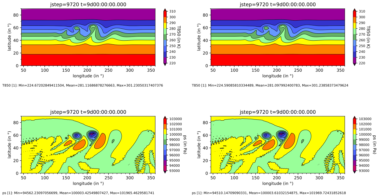
Figure 10. Baroclinic instability test, with filtering. Top: temperature T in 850 hPa at t=9 d, bottom: surface pressure p_s . Left: Euler equation set ' \rho\Theta ', right: equation set ' E '. The colors are similar to those used in (Jablonowski and Williamson, 2006, Fig. 7).
