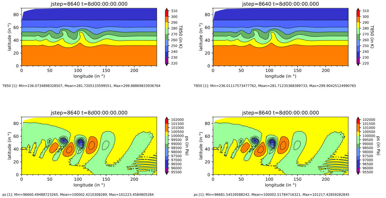
Figure 11. Baroclinic instability test by Ullrich et al. (2014), with filtering. Top: temperature T in 850 hPa at t=8 d, bottom: surface pressure p_s . Left: Euler equation set ' \rho\Theta ', right: equation set ' E '. The isolines and partly the colors are similar to those used in (Ullrich et al., 2014, Fig. 4,5).
