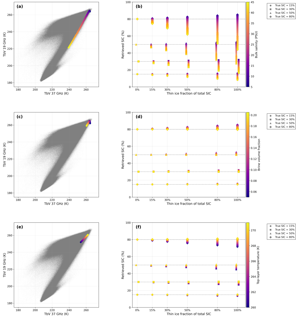
Figure 8. Brightness temperature signature in the 19V–37V space (left column; panels a, c, e) and retrieved SIC (right column; panels b, d, f) for varying proportions of dark nilas mixed with thick first-year sea ice, as obtained with the method described in Sect. 3.5.2. Rows correspond to sensitivity experiments on bulk salinity (a, b), brine volume fraction (c, d), and top-layer temperature (e, f). In the left panels, cold season AMSR2 observations (grey dots) serve as a background, and each modelled point (100% thin ice cover) is colour-coded by the varied parameter value. In the right panels, the true SIC levels (15%, 30%, 50%, 80%) are marked by horizontal dashed lines, and retrieved SIC values are offset horizontally around each thin ice fraction for visual clarity but computed at the exact fraction values.
