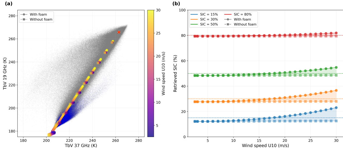
Figure 6. (a) Brightness temperature signature in the 19V–37V space corresponding to wind-induced ocean surface property variations. The MIZ T_B observations (black dots) and open ocean observations (blue dots) from AMSR2 correspond to warm conditions. Both the observation clusters are masked as described in section 3.5. Each data point is coloured by wind speed value, and it derives from a SIC linear combination (shown at 10% SIC increments). (b) Warm season. SIC retrieved for wind speed variation from the reference ocean parametrisation with foam ( 15 \text{ ms}^{-1} ). True SIC values (15%, 30%, 50%, 80% selected to represent characteristic values across the MIZ range) are shown with horizontal lines. Data points are coloured by SIC and shown for increasing wind speeds from 2 to 30 \text{ ms}^{-1} . The simulations are shown both including the foam effect (circles) or not (squares).
