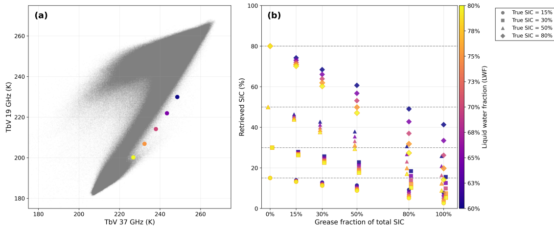
Figure 10. Brightness temperature signature in the 19V–37V space (a) and retrieved SIC (b) for varying proportions of grease ice mixed with thick first-year sea ice. In the left panel, cold season AMSR2 observations (grey dots) serve as a background and each modelled point (100% grease cover) is colour-coded by LWF value. In the right panel, the true SIC levels (15%, 30%, 50%, 80%) are marked by horizontal dashed lines, and retrieved SIC values are offset horizontally around each thin ice fraction for visual clarity but computed at the exact fraction values.
