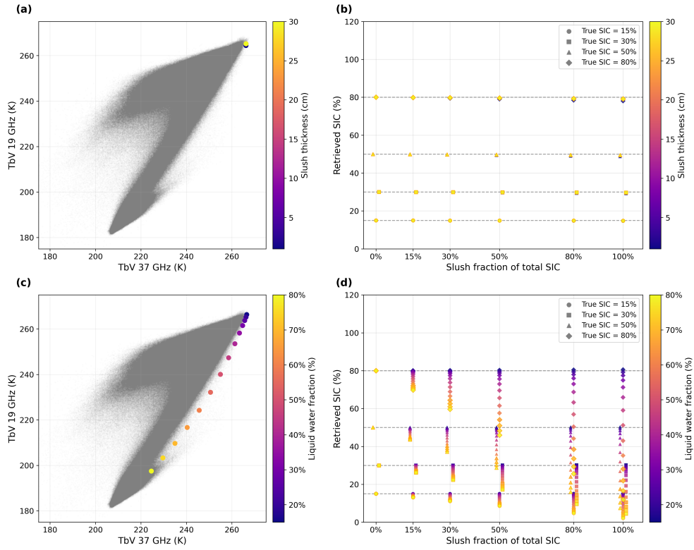
Figure 7. Brightness temperature signature in the 19V–37V space (left column; panels a, c) and retrieved SIC (right column; panels b,d) for varying proportions of slush mixed with thick first-year sea ice. Rows correspond to sensitivity experiments on slush thickness (a, b) and liquid water fraction (c, d). In the left panels, cold season AMSR-2 observations (grey dots) serve as a background and each modelled point (100% slush cover) is colour-coded by the varied parameter value. In the right panels, the true SIC levels (15%, 30%, 50%, 80%) are marked by horizontal dashed lines, and retrieved SIC values are offset horizontally around each thin ice fraction for visual clarity but computed at the exact fraction values.
