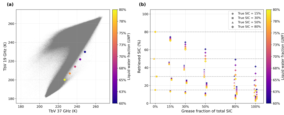
Figure 8. Brightness temperature signature in the 19V–37V space (a) and retrieved SIC (b) for varying proportions of grease ice mixed with thick first-year sea ice. In the left panel, cold season AMSR-2 observations (grey dots) serve as a background and each modelled point (100% grease cover) is colour-coded by LWF value. In the right panel, the true SIC levels (15%, 30%, 50%, 80%) are marked by horizontal dashed lines, and retrieved SIC values are offset horizontally around each thin ice fraction for visual clarity but computed at the exact fraction values.
