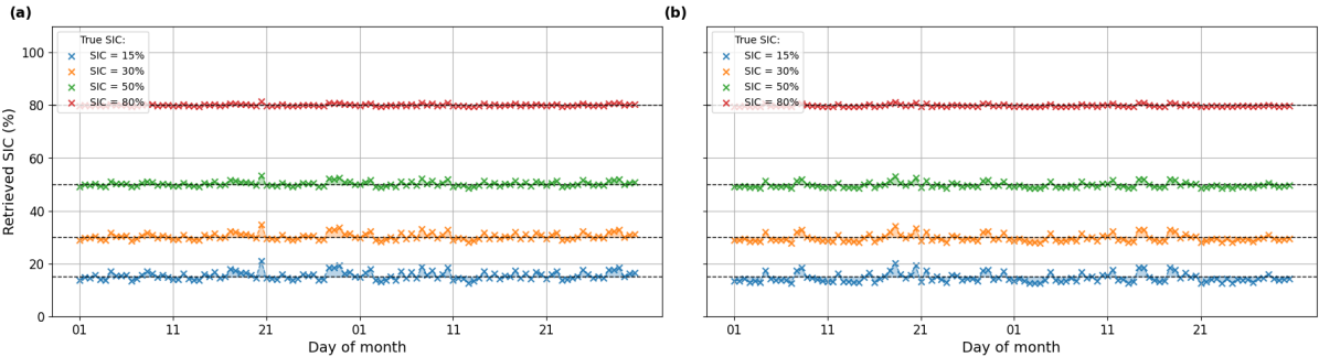
Figure 10. (a) SIC retrieved for different atmospheric profiles selected as in Sect. 3.4 for the warm season. True SIC values (15%, 30%, 50%, 80% shown to represent characteristic values across the MIZ range) are represented with horizontal lines. Data points are coloured by SIC and sampled for the atmosphere at different times and locations, ordered chronologically on the x-axis. (b) Same as (a) for the cold season.
