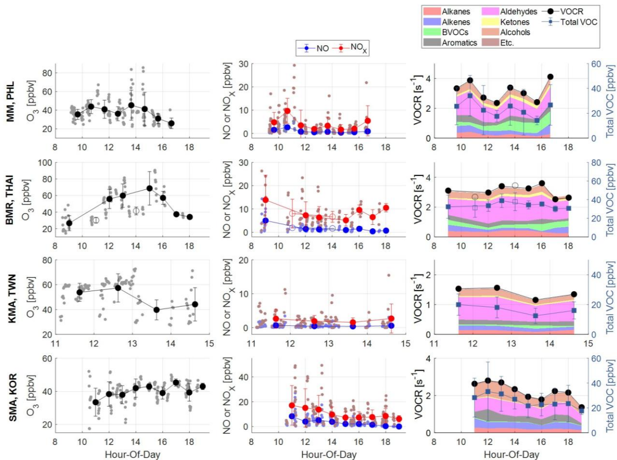
Figure 3. Mean diurnal patterns of the mixing ratios of O_3 , NO, NO_x , VOCs, and non-methane VOC reactivity (VOCR) near the surface ( < 750 m) in Asian megacities. Pale-colored dots represent 1-minute averaged observations. Colored dots and error bars denote hourly averages and standard deviations. Stacked colored areas indicate the contributions of different VOC classes to VOCR. The open circles in the BMR panel indicate data that were sampled at relatively high altitudes. All times are local time (LT).
