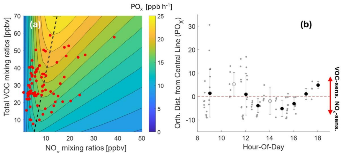
Figure 5. (a) Colored isopleth of ozone production rate (PO x ) as functions of NO x and VOC mixing ratios in the Bangkok Metropolitan Region (BMR), Thailand. The dashed lines denote the transition between NO x -sensitive (left area of the transition) and VOC-sensitive (right area of the transition) regimes. Red dots indicate the observed data points (1-min average) sampled below 750 m. (b) Diurnal variation of the orthogonal distance of observation from the PO x transition line (negative values: NO x -sensitive; positive values: VOC-sensitive). The red dashed lines denote the transition line. Grey dots indicate individual data points (1-min average), and black dots and error bars represent the hourly mean values and standard deviations, respectively. The open circles at 11:00 and 14:00 LT indicates the data were sampled at relatively high altitude. All times are local time (LT).
