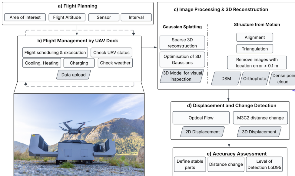
Figure 4 Workflow for multitemporal UAV monitoring and displacement and change detection analysis in alpine terrain, consisting of a) flight planning, b) flight management by the UAV dock. Photograph shows the dock in operation at the study site Skjold, c) image processing and 3D reconstruction, d) spatiotemporal change and displacement detection (optical flow on DSM and M3C2 on point cloud), and e) accuracy assessment.
