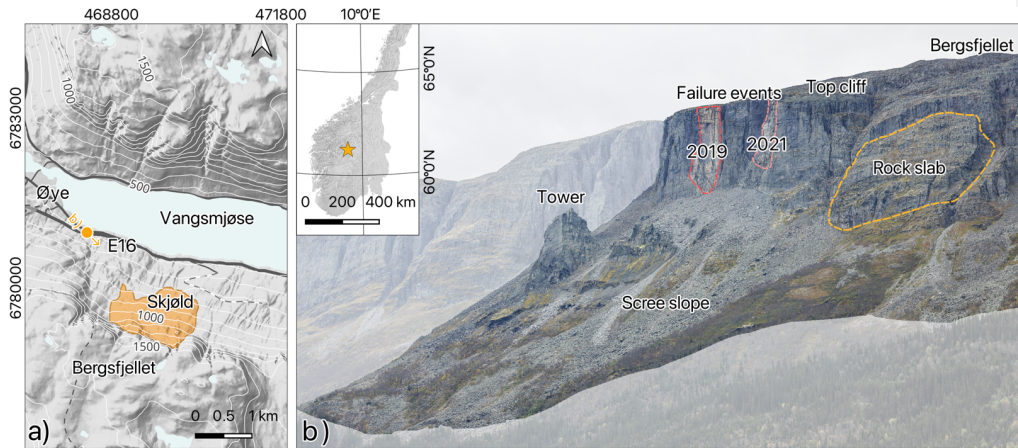
Figure 2 a) Location of the unstable rock slope Skjöld above the road E16 and Vangsmjøse in eastern Norway (inset). Contour lines indicate elevation in m asl. b) Photograph showing the location of the main tower, the failure events from 2019 and 2021 (red outlines) and the rock slab (orange outline). The camera location is indicated in (a) by an orange dot. Elevation data: Kartverket
