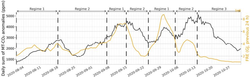
Figure 5: Time series, smoothed using a 72-hour window, of the daily sum of mid-tropospheric CO 2 anomalies derived from IASI morning and evening overpasses (black), over South America during the 2020 fire season and of total FRE (orange) from GOES-16 observations, integrated over South America and computed 24 hours prior to each IASI observation to account for
