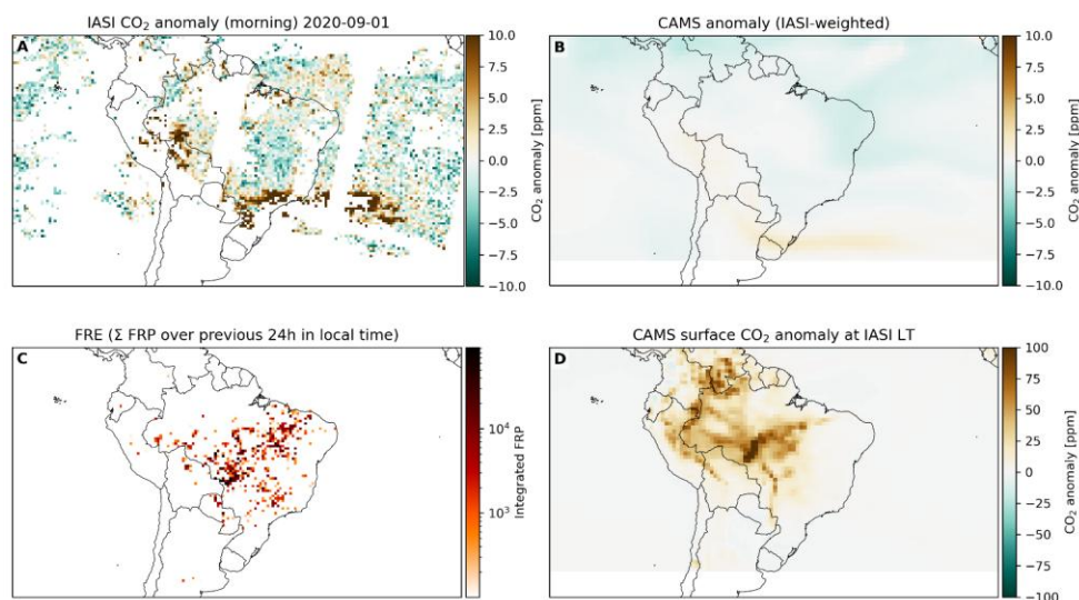
Figure 8: Comparison between IASI mid-tropospheric CO 2 anomalies and the CAMS EGG4 reanalysis for a representative day (1 September 2020). (A) IASI-observed MT-CO 2 anomaly (morning overpass); (B) EGG4 IASI-weighted MT-CO 2 partial-column anomaly; (C) Fire Radiative Energy (Σ FRP over the preceding 24 h); (D) EGG4 surface CO 2 anomaly at the IASI local overpass time.
