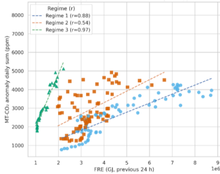
Figure 6: Daily sum of mid-tropospheric CO 2 anomalies (ppm) vs. Fire Radiative Energy (FRE, GJ) for three transport regimes: L ongitudinal transport (blue), C ircular transport (orange), and C ombined transport (green). Pearson correlation coefficients ‘r’ are indicated for each transport regime.
