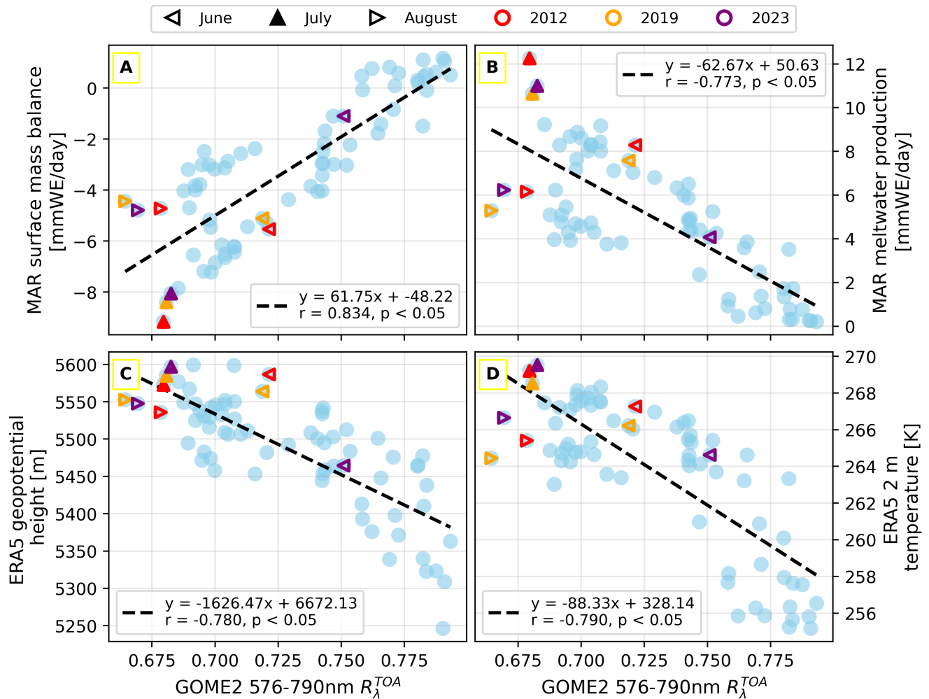
Figure 7. GOME-2 R_{\lambda}^{TOA} plotted against (A) MAR surface mass balance, (B) MAR meltwater production, (C) ERA5 geopotential height, and (D) ERA5 2 m temperature. Each point is a Greenland-wide average for May, June, July and August within the 2007-2024 time frame. June, July and August means for 2012, 2019 and 2023 are all individually represented by left, up and right-facing triangles, respectively, with colors corresponding to the years of interest.
