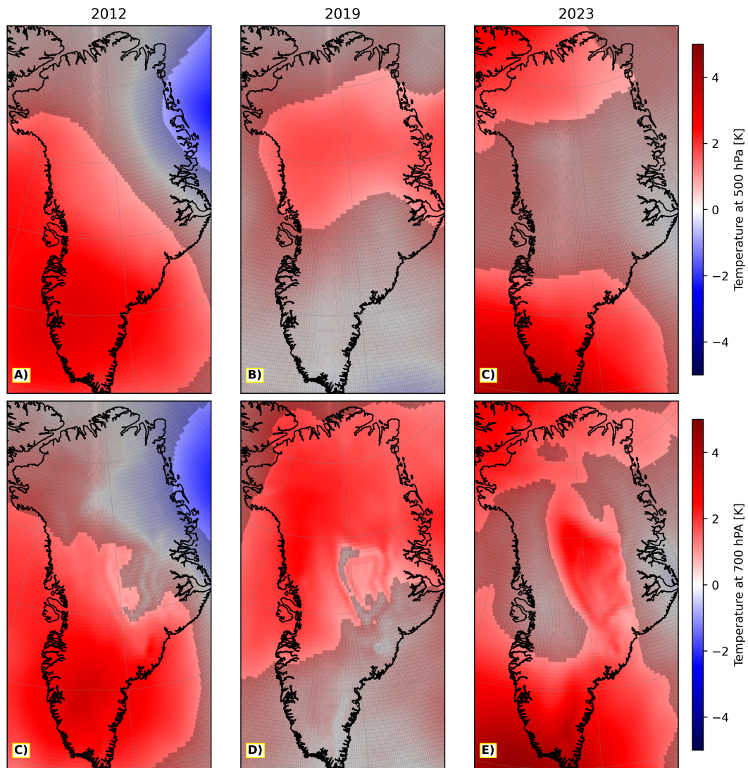
Figure D2. Maps of July ERA5 temperature anomaly at (A-C) 500 hPa and (C-E) 700 hPa. The left, center and right columns correspond 2012, 2019 and 2023, respectively. All anomalies are calculated for the July of each year with respect the 2007-2024 July mean. Grid cells without a gray filter are one standard deviation away from the mean.
