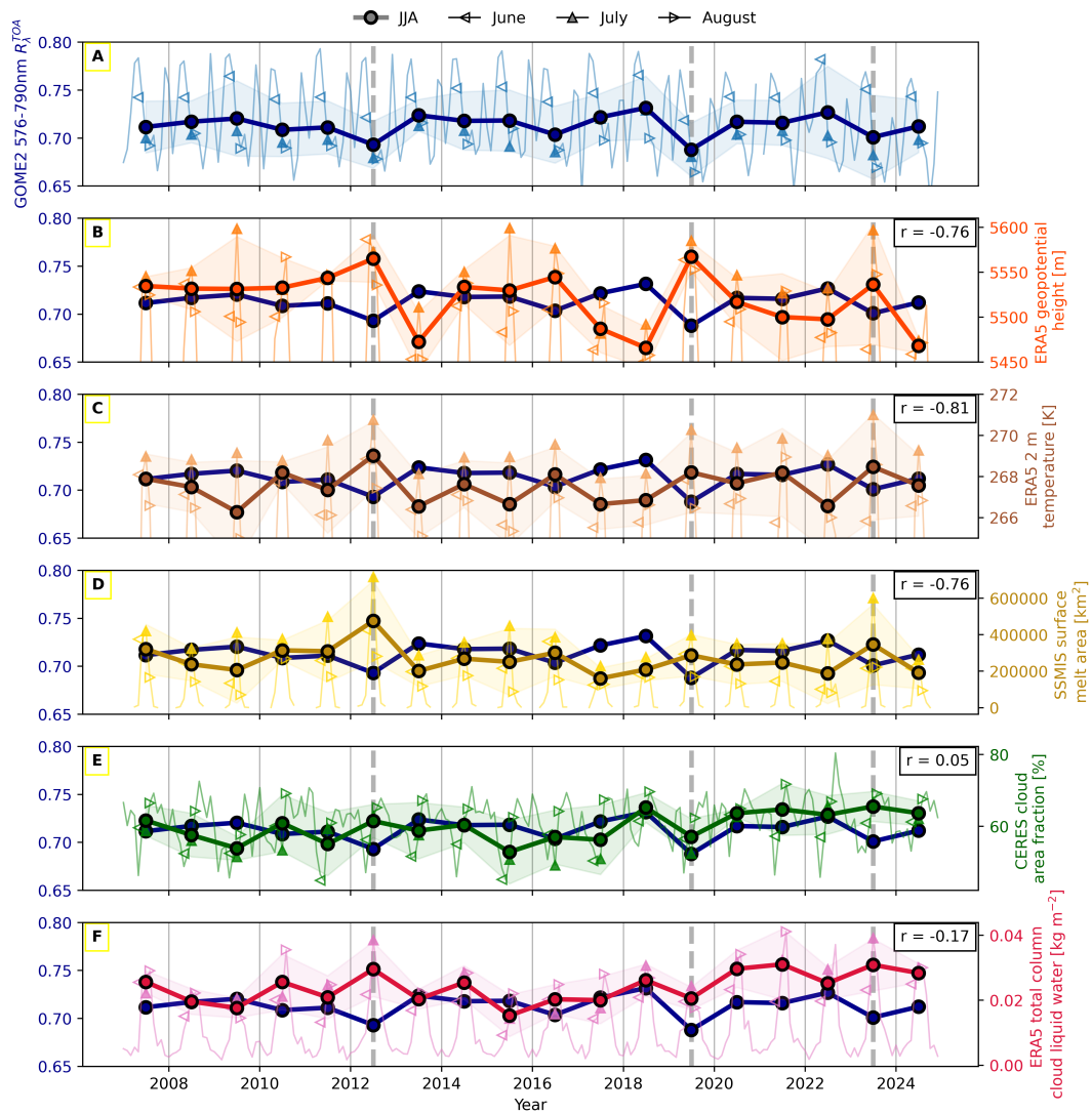
Figure 5. Time series of (A) GOME-2 reflectance at the top of the atmosphere ( R_{\lambda}^{TOA} ) over Greenland, plotted alongside (B) ERA5 500 hPa Geopotential Height averaged over the 60–80°N, 20–80°W region, (C) ERA5 2 m temperature, (D) SSMIS surface melt area, (E) CERES cloud area fraction, and (F) ERA5 total column cloud liquid water, respectively. Filled circles connected by thick solid lines show only the June-July-August (JJA) averages, while the thinner line depicts the full monthly dataset. June, July and August means are all individually represented by left, up and right-facing triangles, respectively. All points in the time series represent Greenland-wide spatial averages weighted by latitude for the respective parameter. The data is color-coded according to the axis label, and the semi-transparent sleeves around the main data represents one standard deviation (calculated over the averaging period). Vertical dashed gray lines represent the anomalous summers of interest: 2012, 2019 and 2023. The pearson correlation coefficient reported in the legend is computed between the JJA averages of the parameters shown in each subplot.
