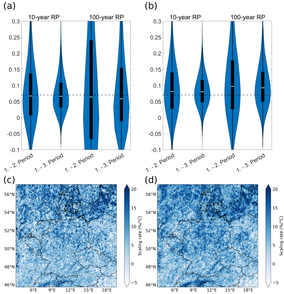
Figure 5. Temperature scaling for the 10-year and 100-year return levels for the GEV (a) and sMEV (b) approach across the study area. For Fig. (a) & (b) the y-axis shows the relative change of the return level per degree of warming, based on the 30-year average temperature of each period. The temperature scaling is shown for the difference between the first and second period as well as the first and third period. Black bars mark the 25th and 75th quantiles with the white marker showing the mean. The dashed line indicates the Clausius-Clapeyron scaling of \frac{7\%}{^{\circ}\text{C}} . Figures (c) and (d) display the 10-year return level change per degree of warming for the GEV (c) and sMEV (d) approach. The rate of change is calculated based on the return levels of the periods 2071-2100 and 1971-2001.
