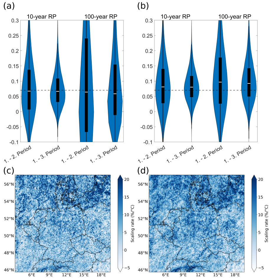
Figure 5. Temperature scaling for the 10-year and 100-year return levels for the GEV (a) and sMEV (b) approach across the study area. The For Fig. (a) & (b) the y-axis shows the relative change of the return level per degree of warming, based on the 30-year average temperature of each period. The temperature scaling is shown for the difference between the first and second period as well as the first and third period. Black bars mark the 25th and 75th quantiles with the white marker showing the mean. The dashed line indicates the Clausius-Clapeyron scaling of \frac{7\%}{^{\circ}\text{C}} . Figures (c) and (d) display the 10-year return level change per degree of warming for the GEV (c) and sMEV (d) approach. The rate of change is calculated based on the return levels of the periods 2071-2100 and 1971-2001.
