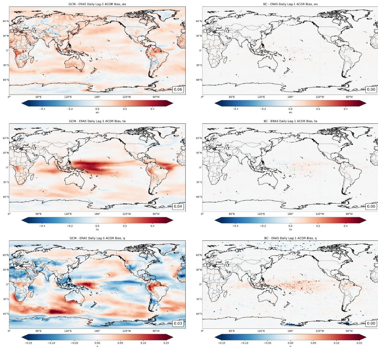
Figure 5 As in Figure 3, but for lag1 auto-correlation. Domain-averaged MAE values are shown; very small errors ( \sim 10^{-3} ) appear as 0.00 due to rounding.
