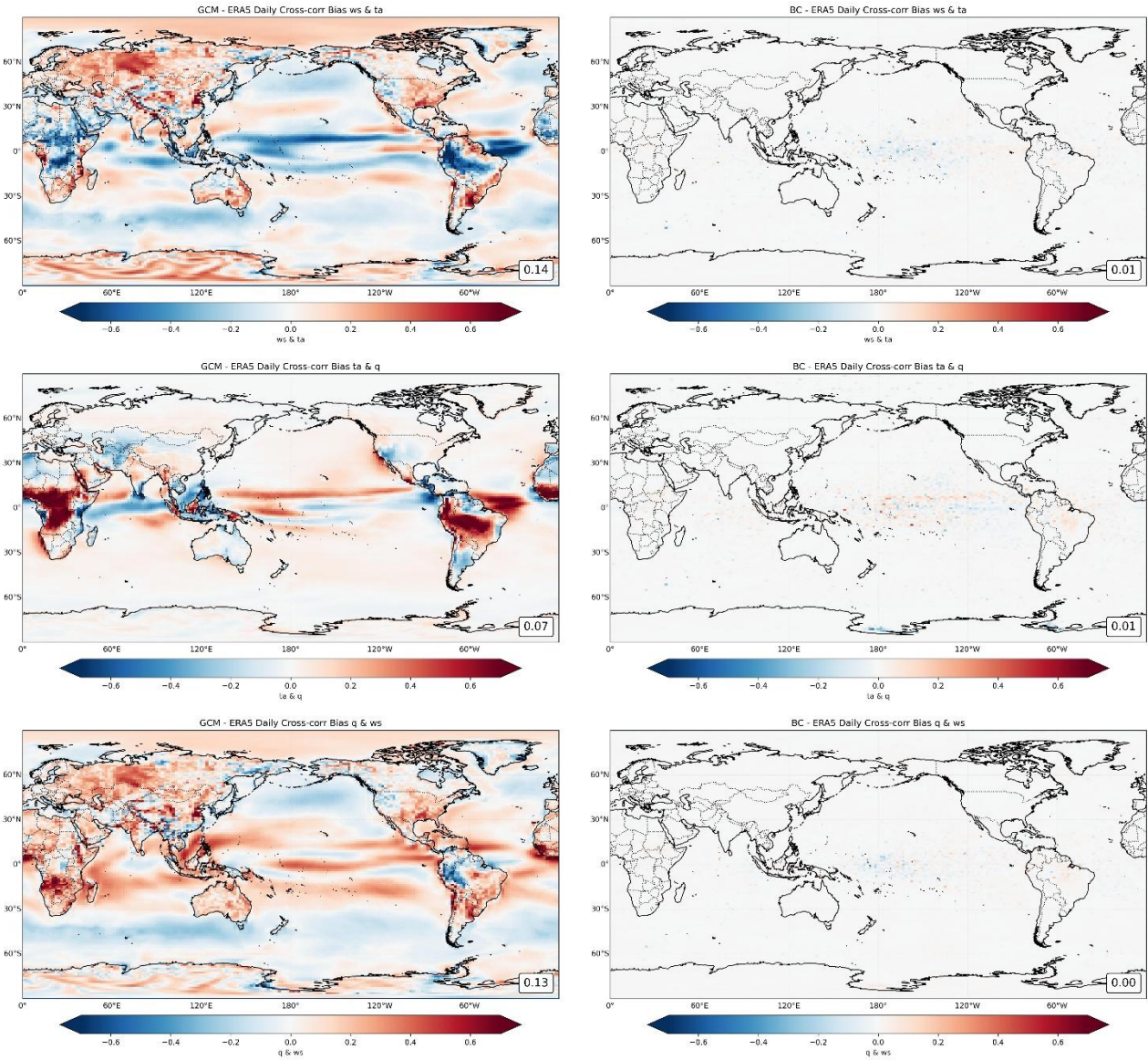
Figure 6 As in Figure 3, but for lag0 cross-correlation
