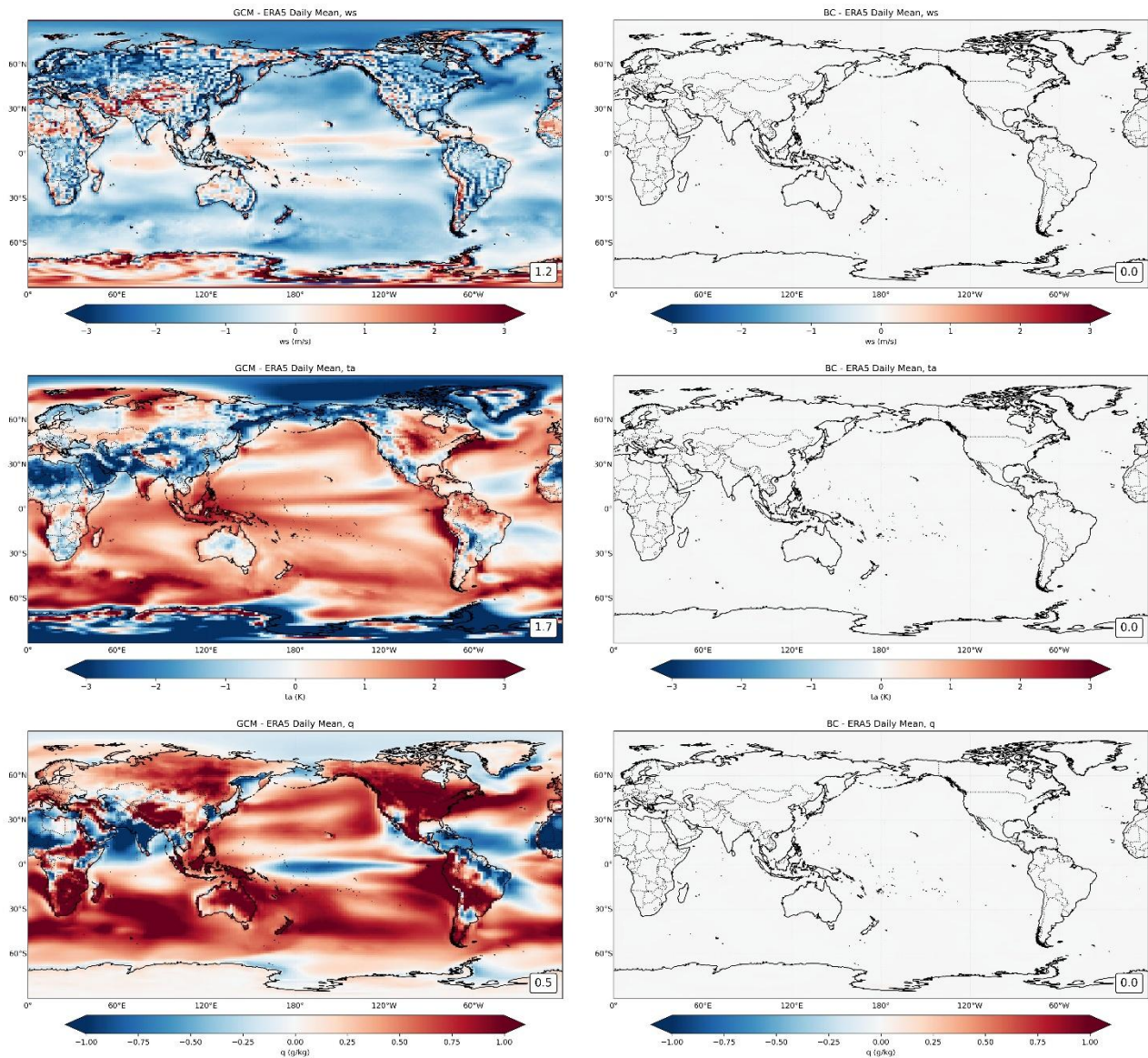
270 Figure 3 Climatological mean bias maps comparing ERA5 with GCM outputs before (left panels) and after (right panels) bias correction (BC), evaluated at the lowest model level on a daily time scale for the calibration period (1959–1989). The panels show results for wind speed (ws), air temperature (ta), and specific humidity (q). The number at the bottom right shows the mean absolute error.
