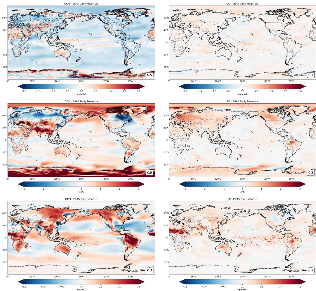
365 Figure 10 As in Figure 9, but for standard deviation
