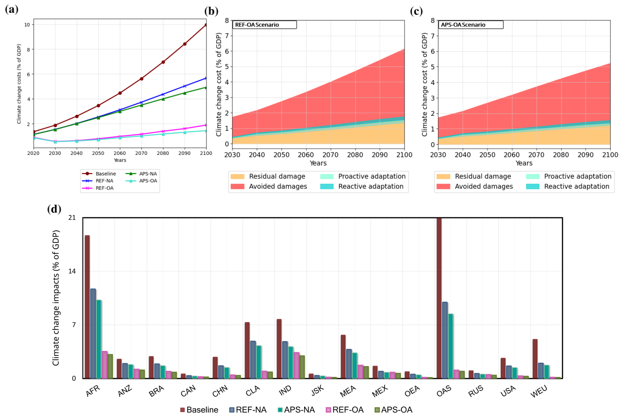
Figure 10. (a) Global total climate change impacts; (b) impacts components in REF-OA and (c) APS-OA scenario; and (d) regional climate impacts in 2100 as a percentage of GDP.
