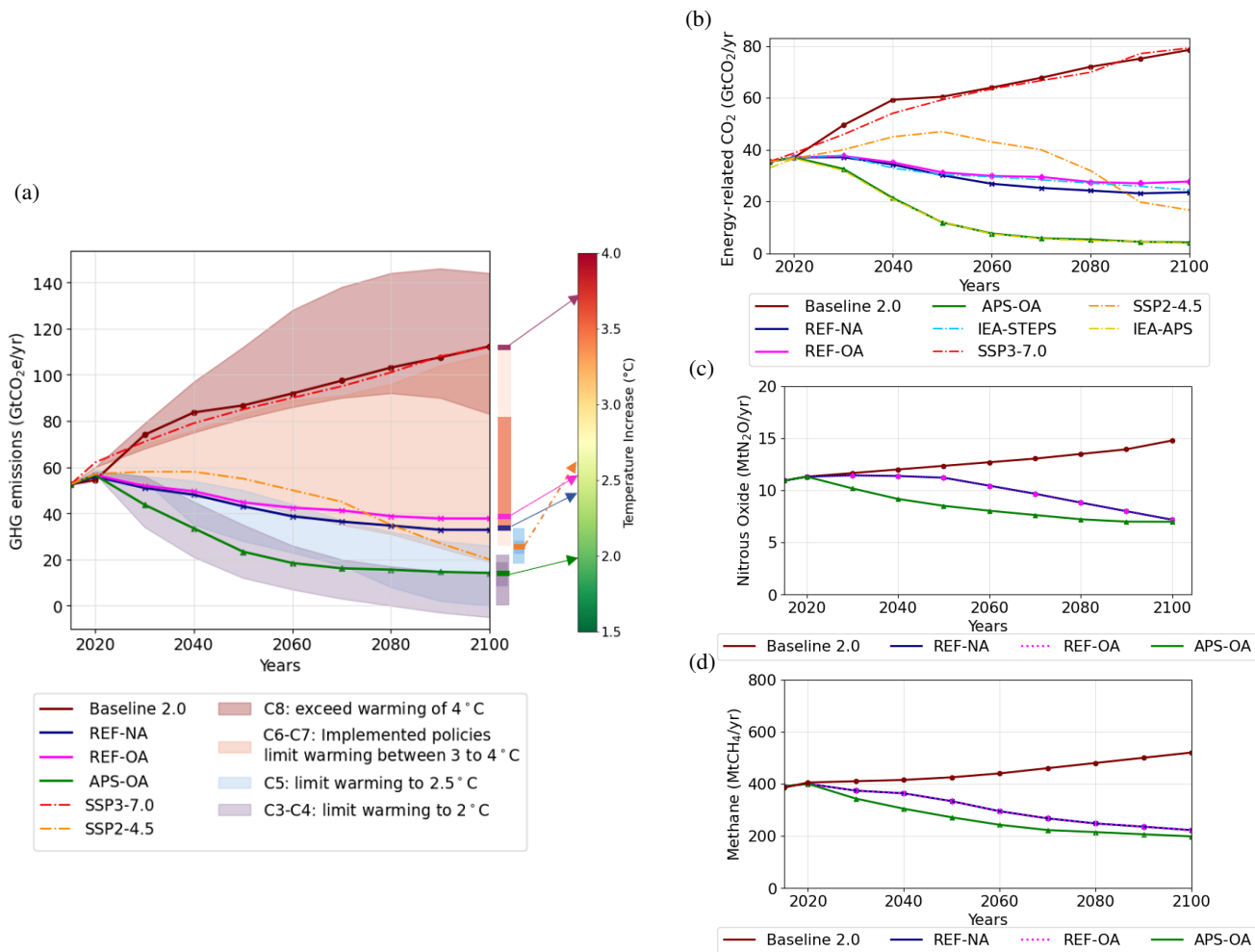
Figure 7. Projected anthropogenic emissions of primary climate change drivers; (a) Total GHG emissions (b) energy-related CO 2 emissions (c) total N 2 O emissions, and (d) total CH 4 emissions comparison across various scenarios: AD-MERGE 2.0 (Baseline 2.0, REF-NA, REF-OA and APS-OA), two IPCC representative pathways (SSP2-4.5 and SSP3-7.0), and IEA scenarios (IEA-STEPS and IEA-APS). Shaded patterns represent the C8 to C3 warming levels based on IPCC (2022a) classifications, providing a comparative context for emission trajectories. The ‘Implemented policies’ ranges show emissions pathways assuming policies implemented by the end of 2020 and pathways assuming implementation of NDCs before COP26. The gradient boxes show the 5th to 95th percentile of the projected warming levels in 2100. The figure also illustrates each scenario’s warming levels relative to the period 1850–1900.
